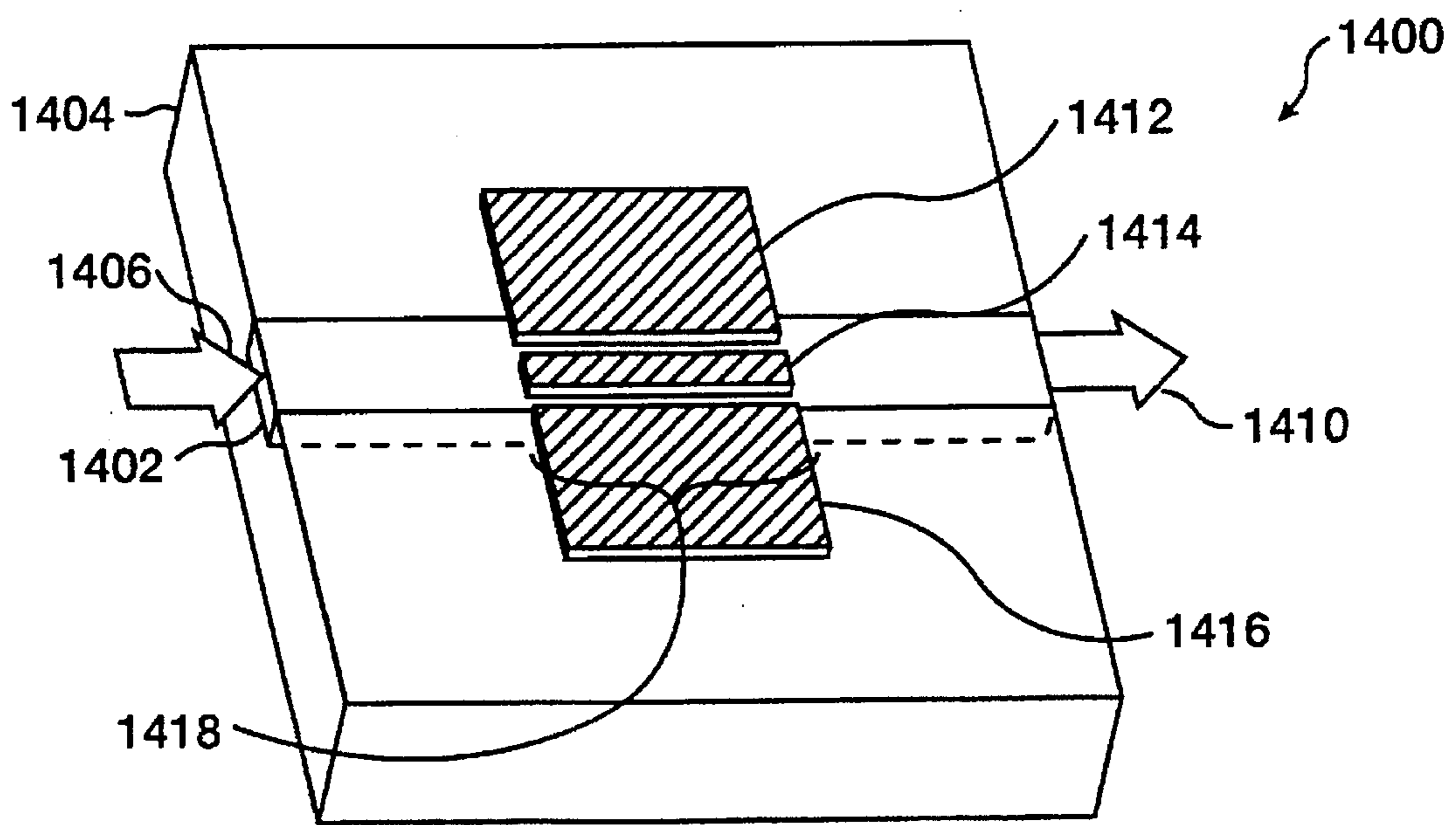
Figure 50 (Prior Art)
