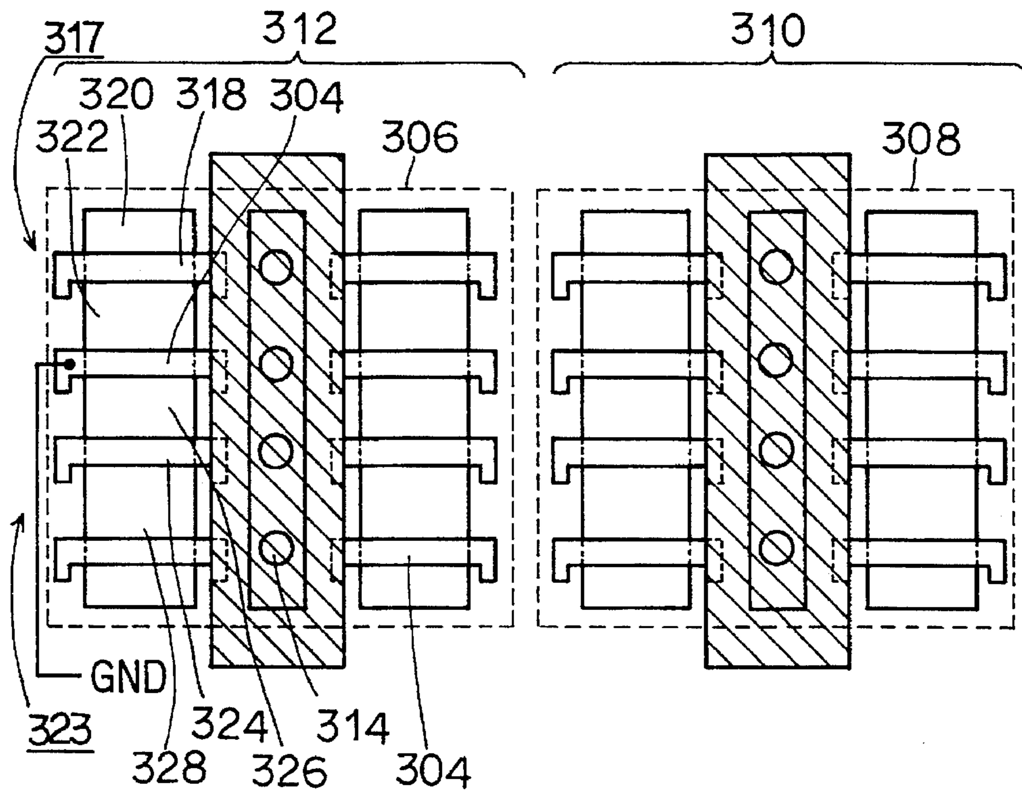
FIG. 78 PRIOR ART
