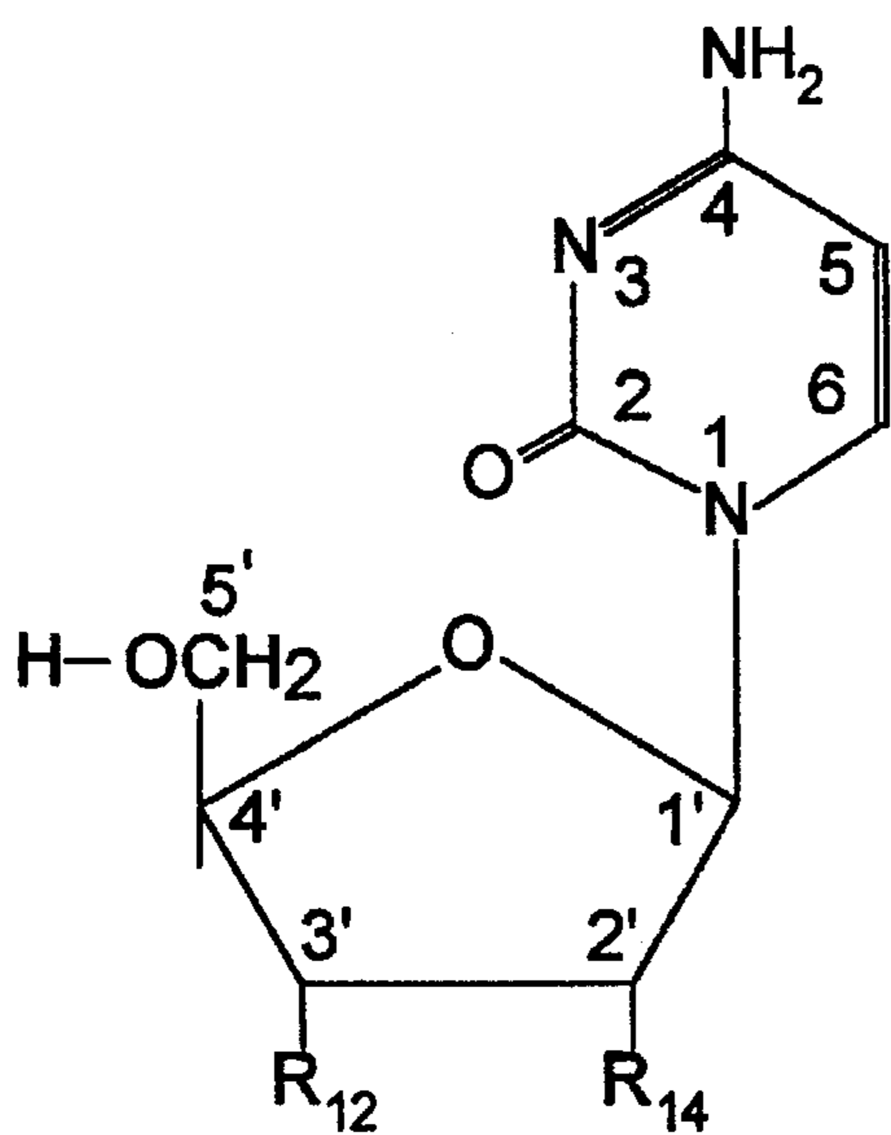
Cytidine
