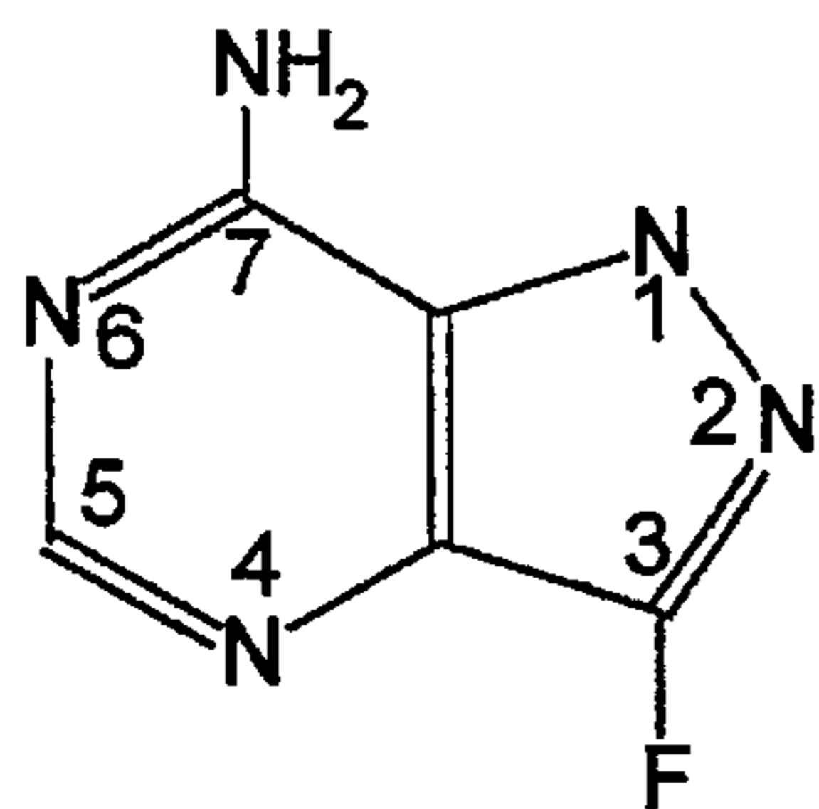
FORMYCIN A
