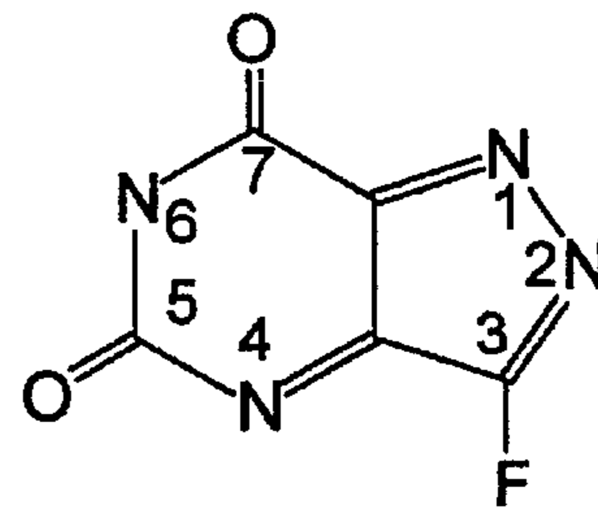
OXYFORMYCIN B
