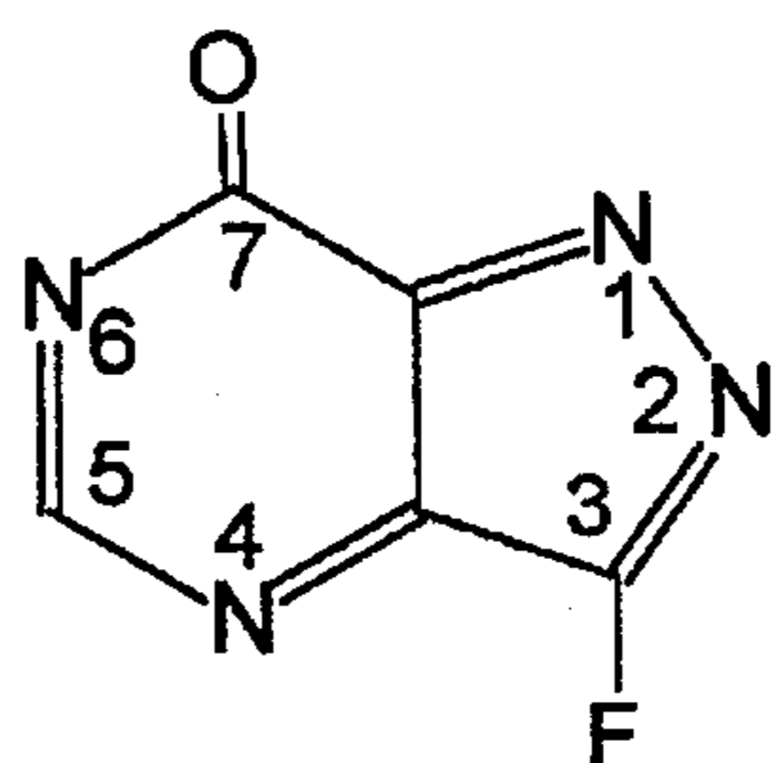
FORMYCIN B
