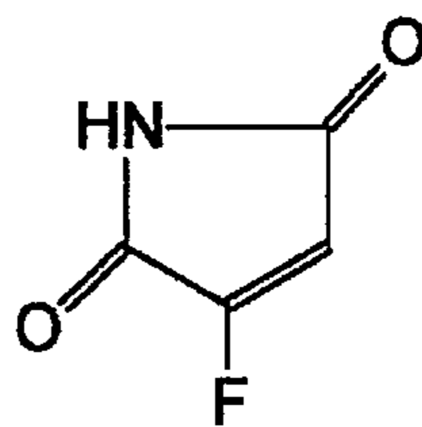
SHOWDOMYCIN
