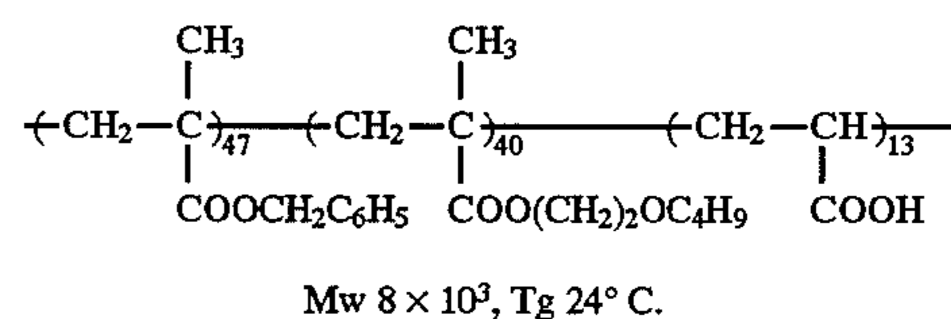
Resin (A-2)
