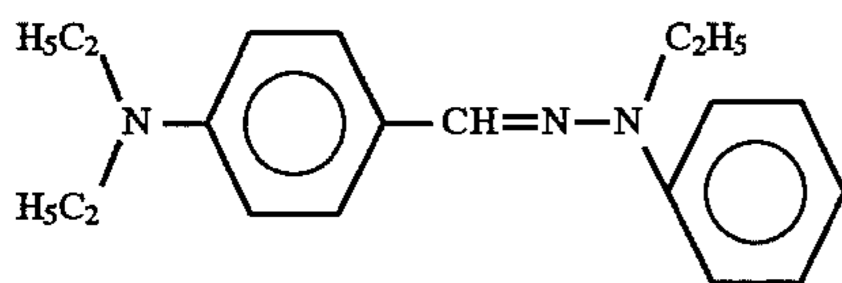
Hydrazone Compound
