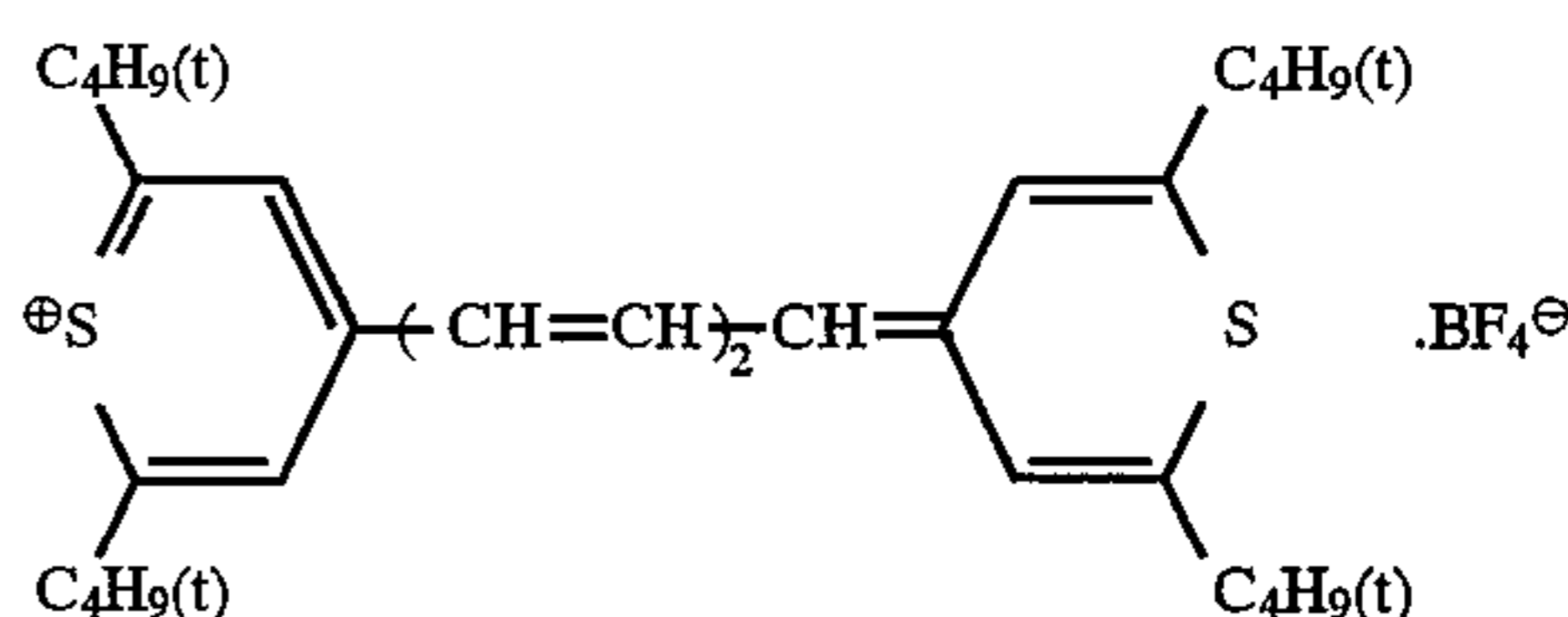
Dye (D-1)
