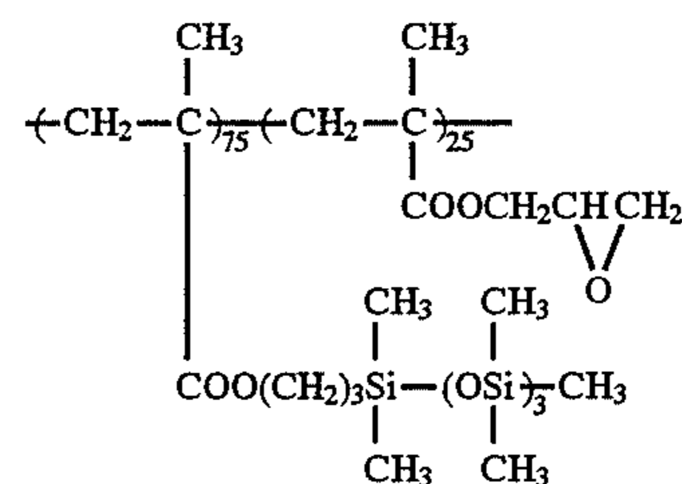
Resin (PP-3)
