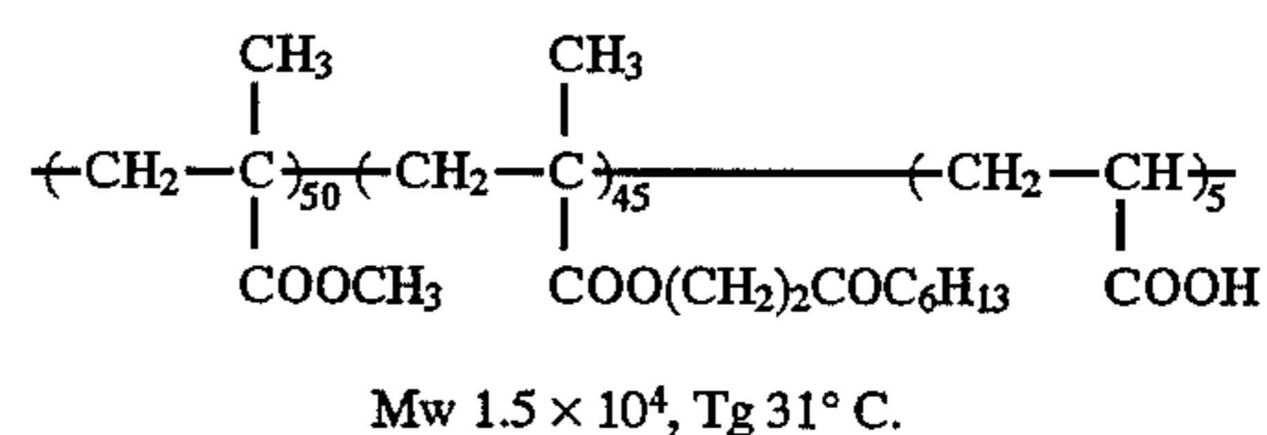
Resin (A-2)
