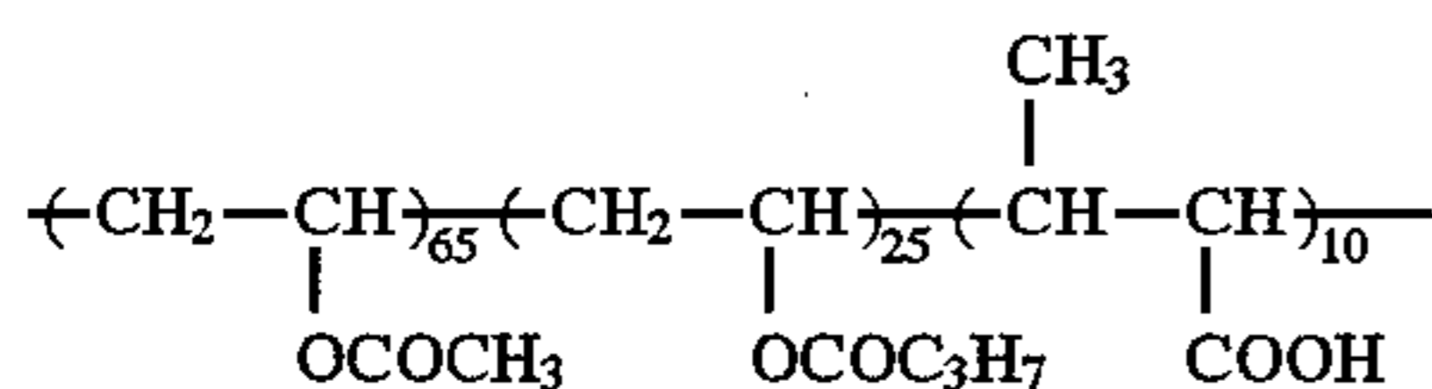
Resin (A-3)
