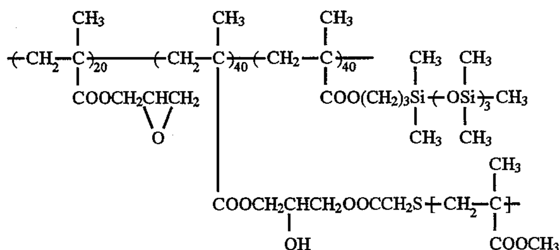
Resin (PP-1)
