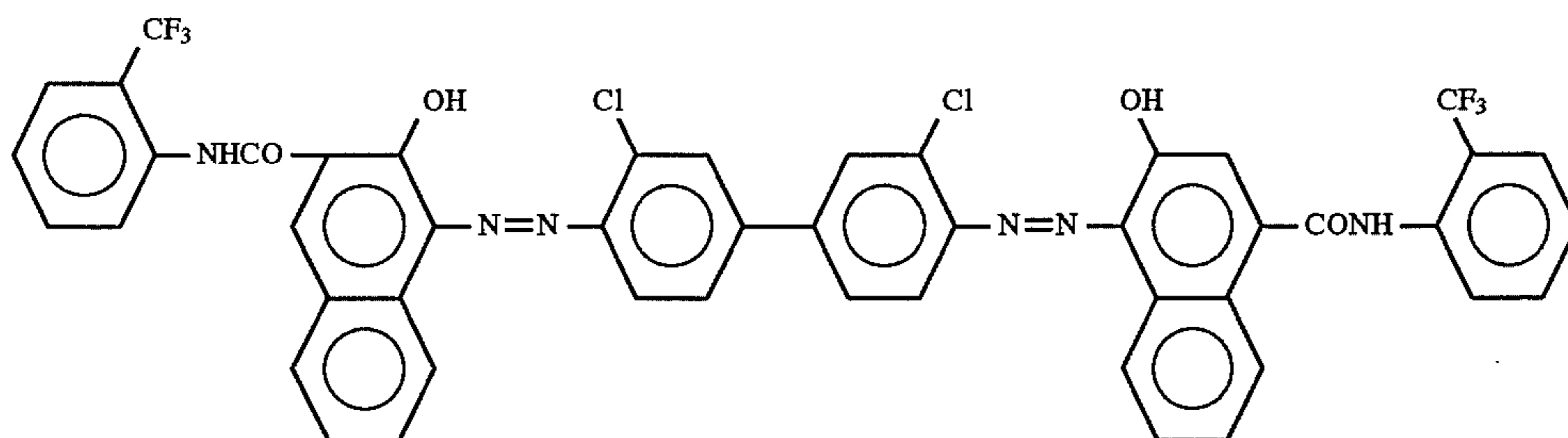
Bisazo Pigment
