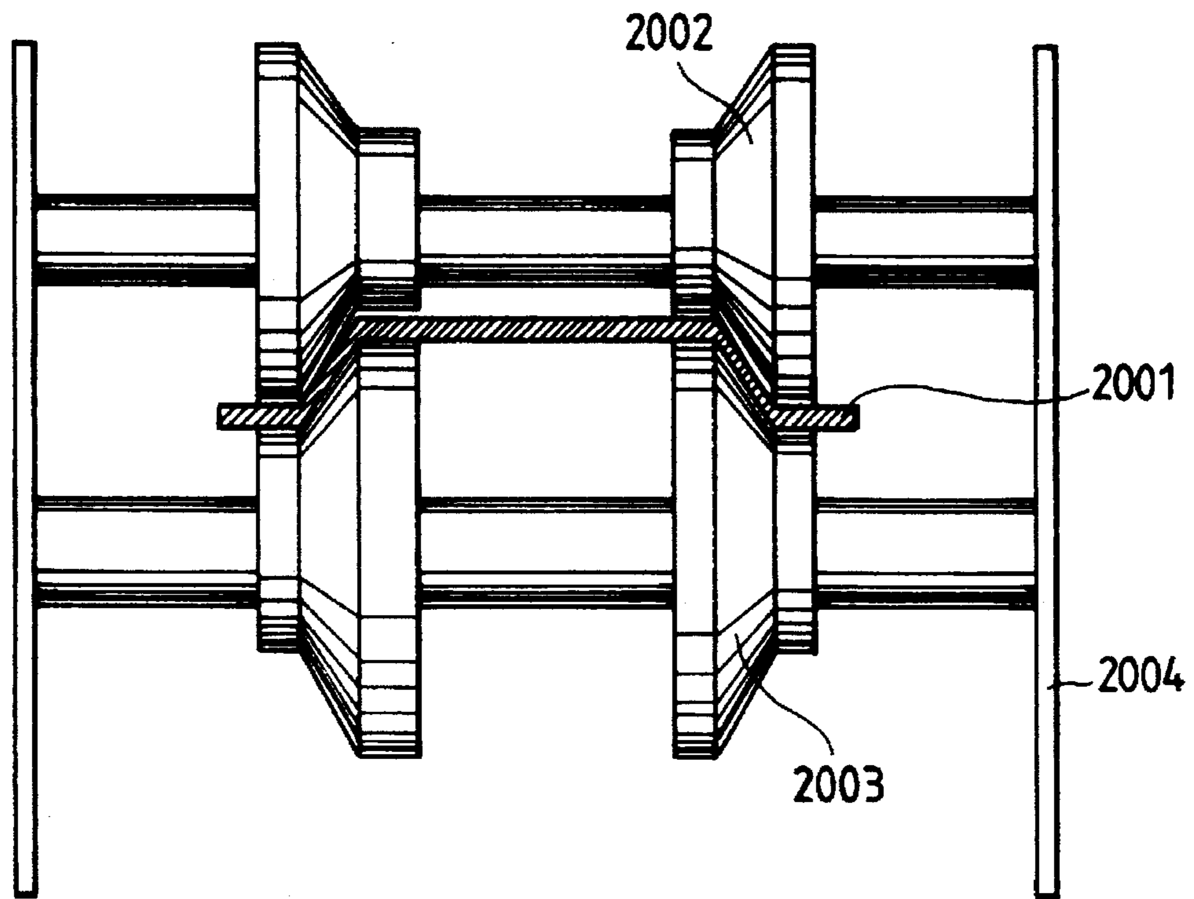
FIG. 20 PRIOR ART
