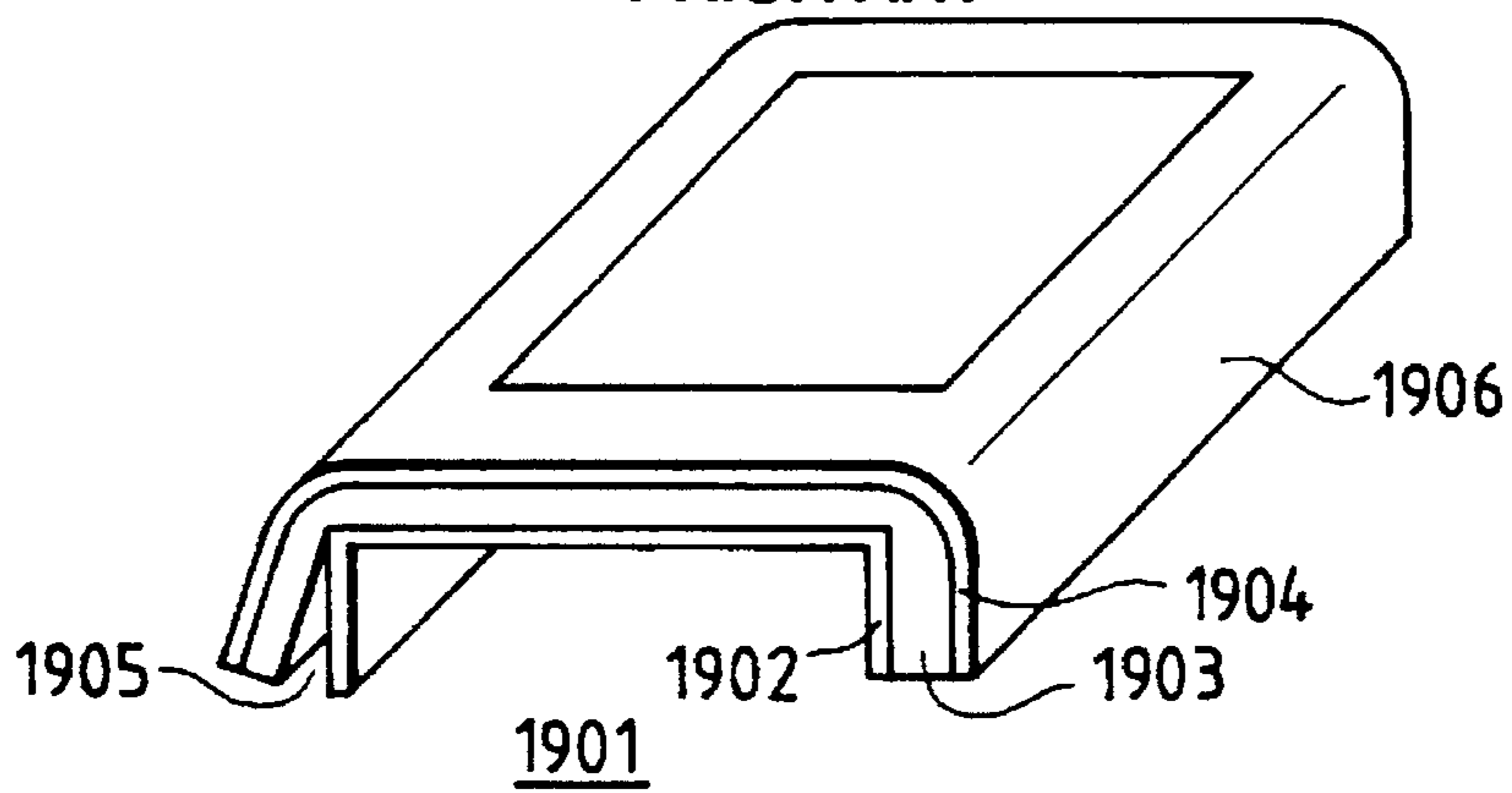
FIG. 19 PRIOR ART
