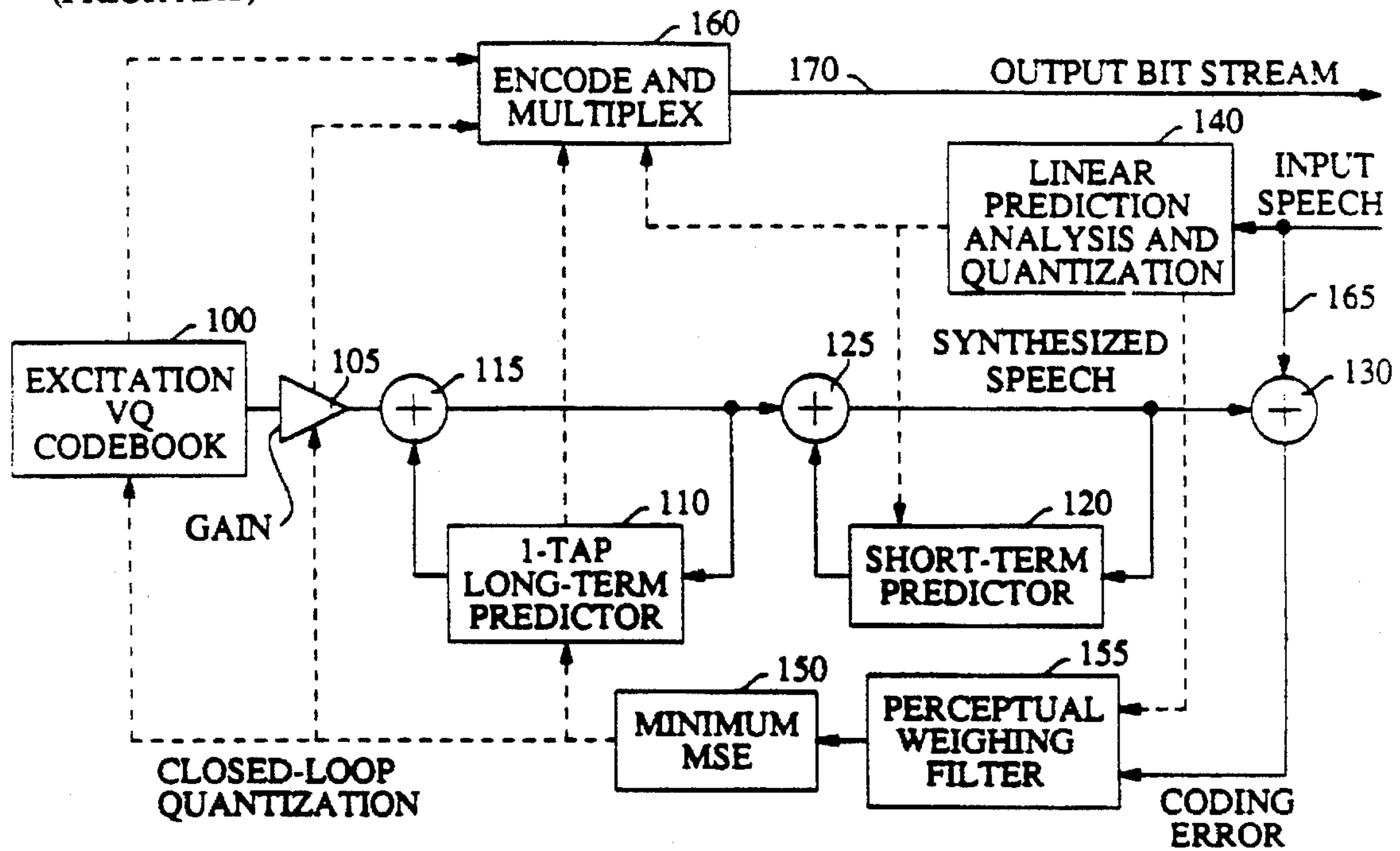
FIG. 1 (PRIOR ART)
