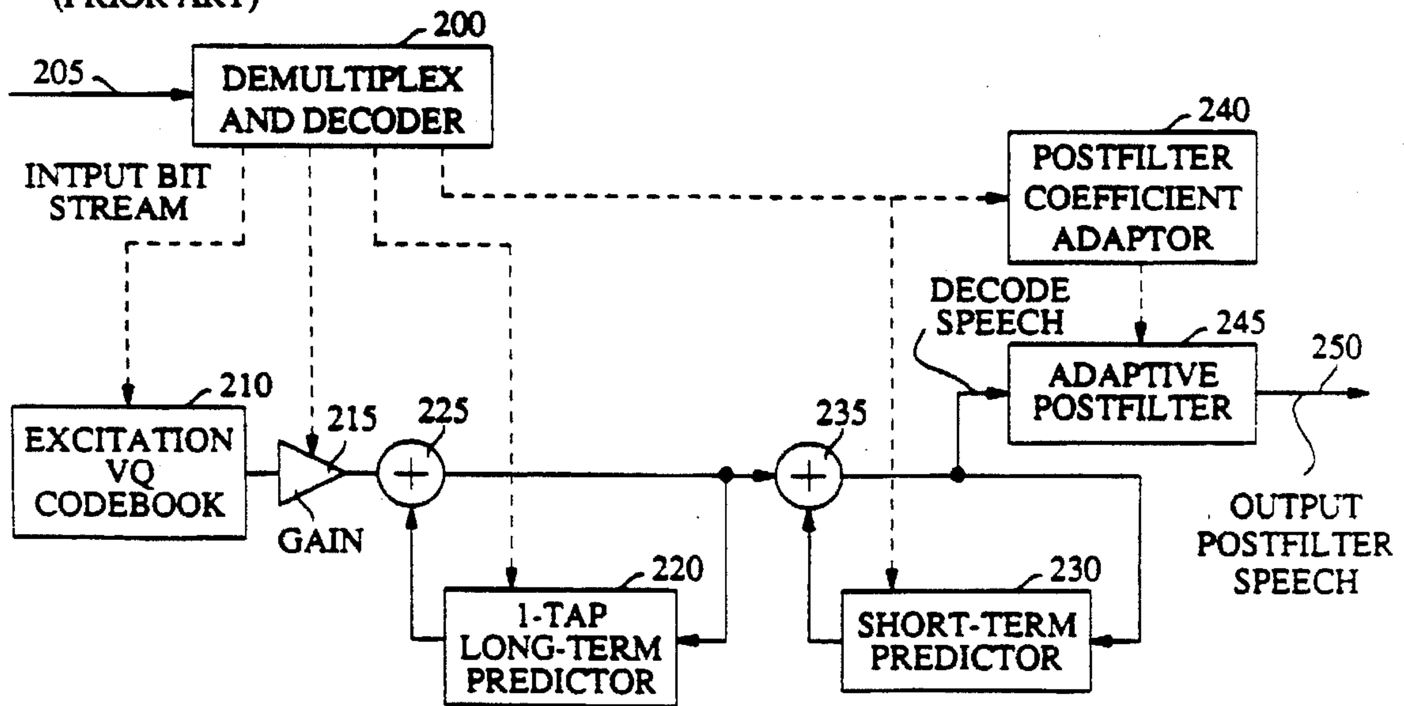
FIG. 2 (PRIOR ART)
