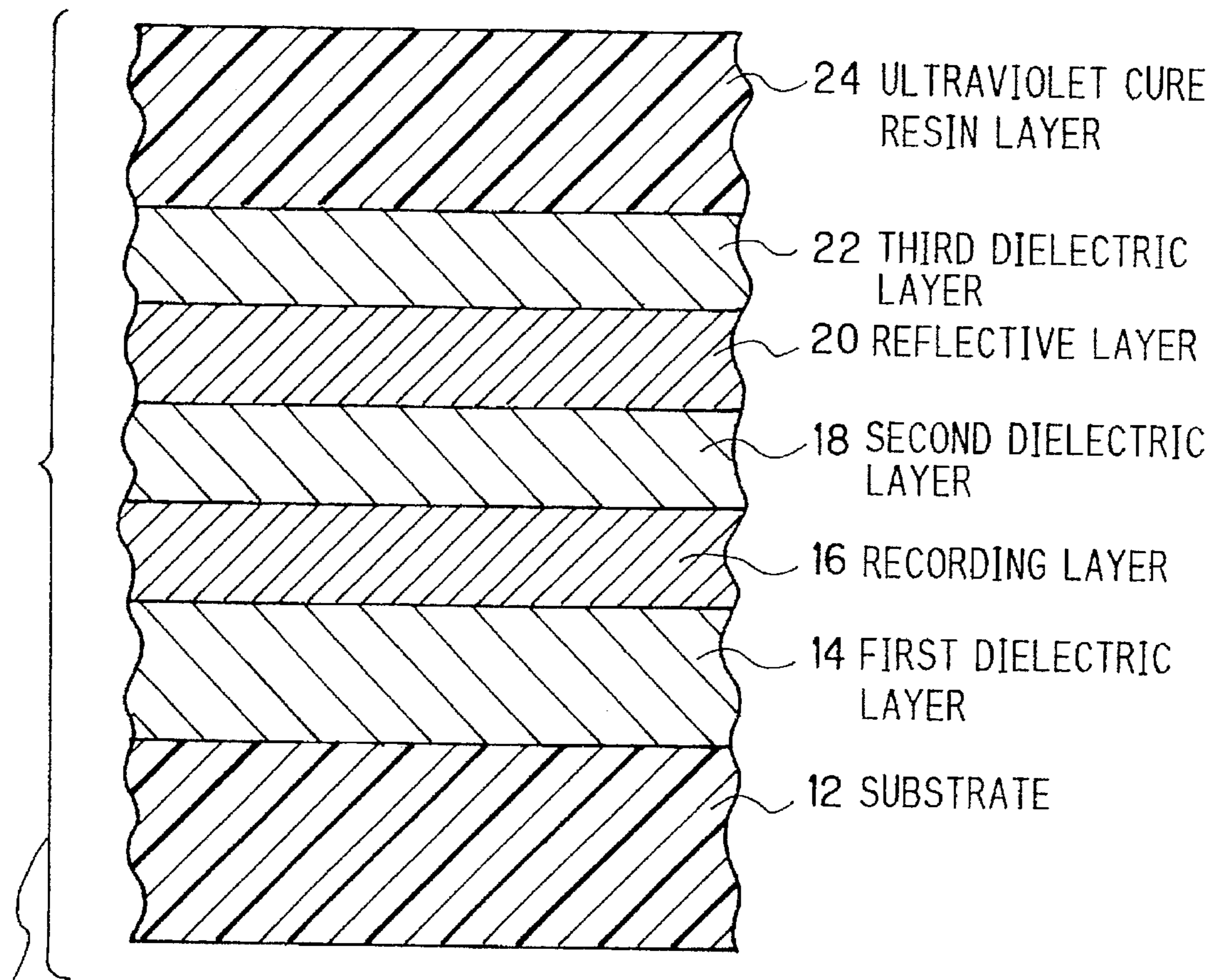
10 PHASE CHANGE OPTICAL DISK
