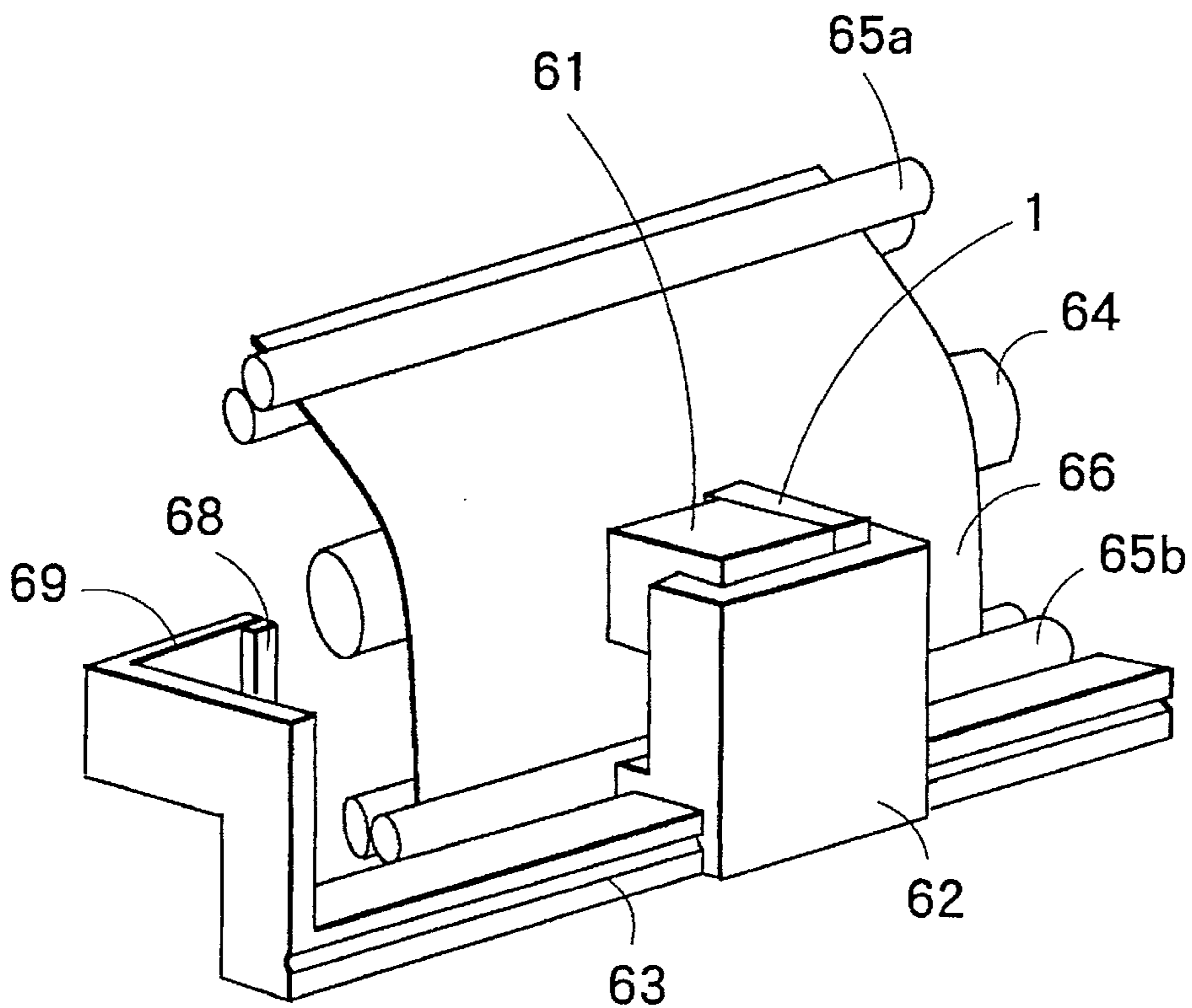
FIG. 5 PRIOR ART
