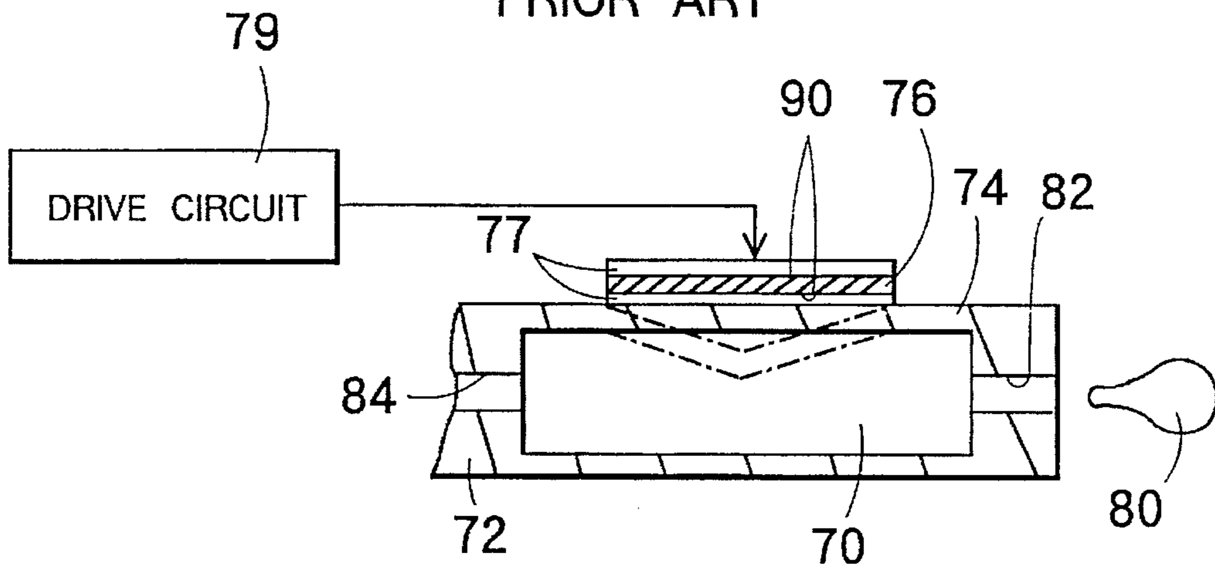
FIG. 1 PRIOR ART
