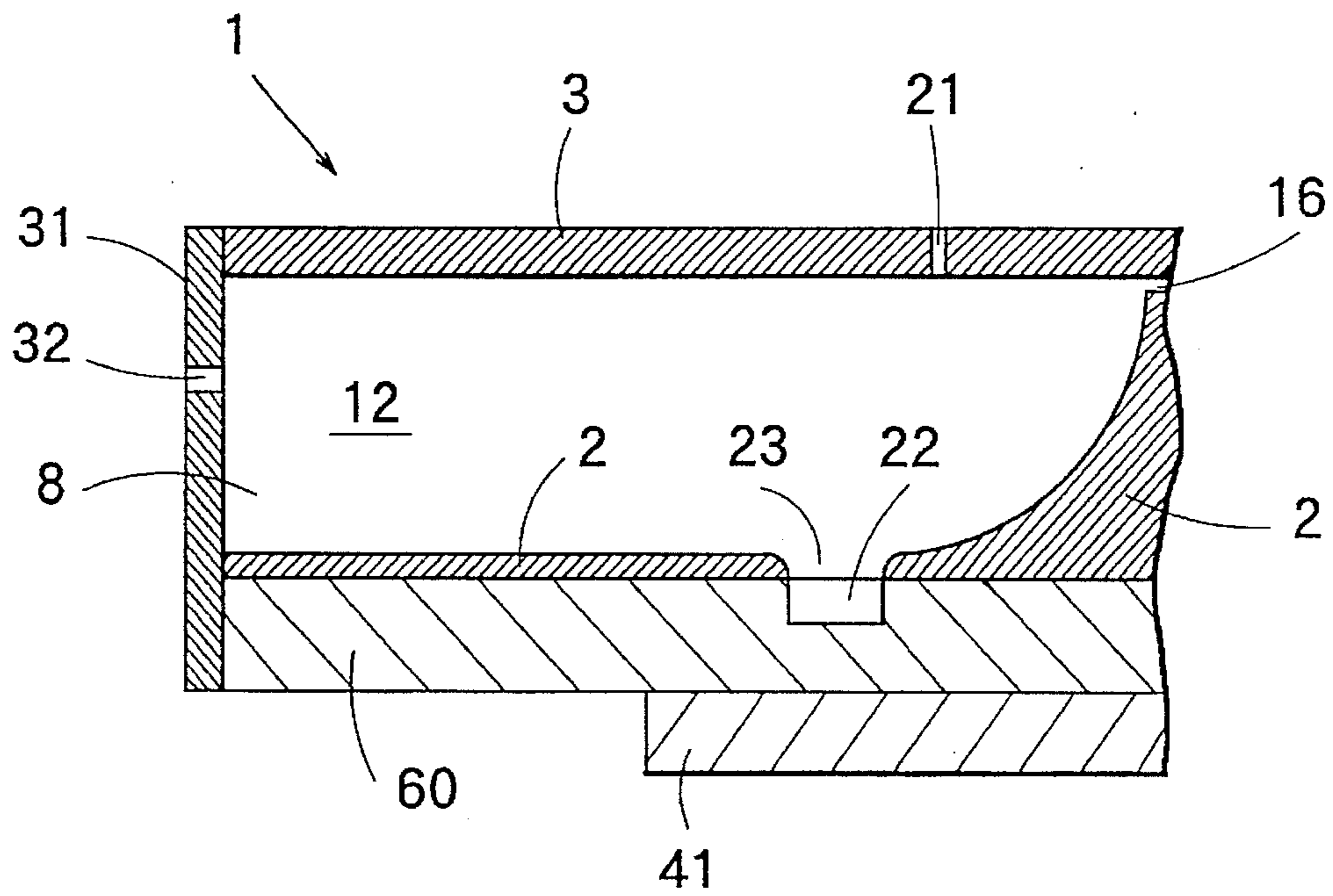
FIG. 6 PRIOR ART
