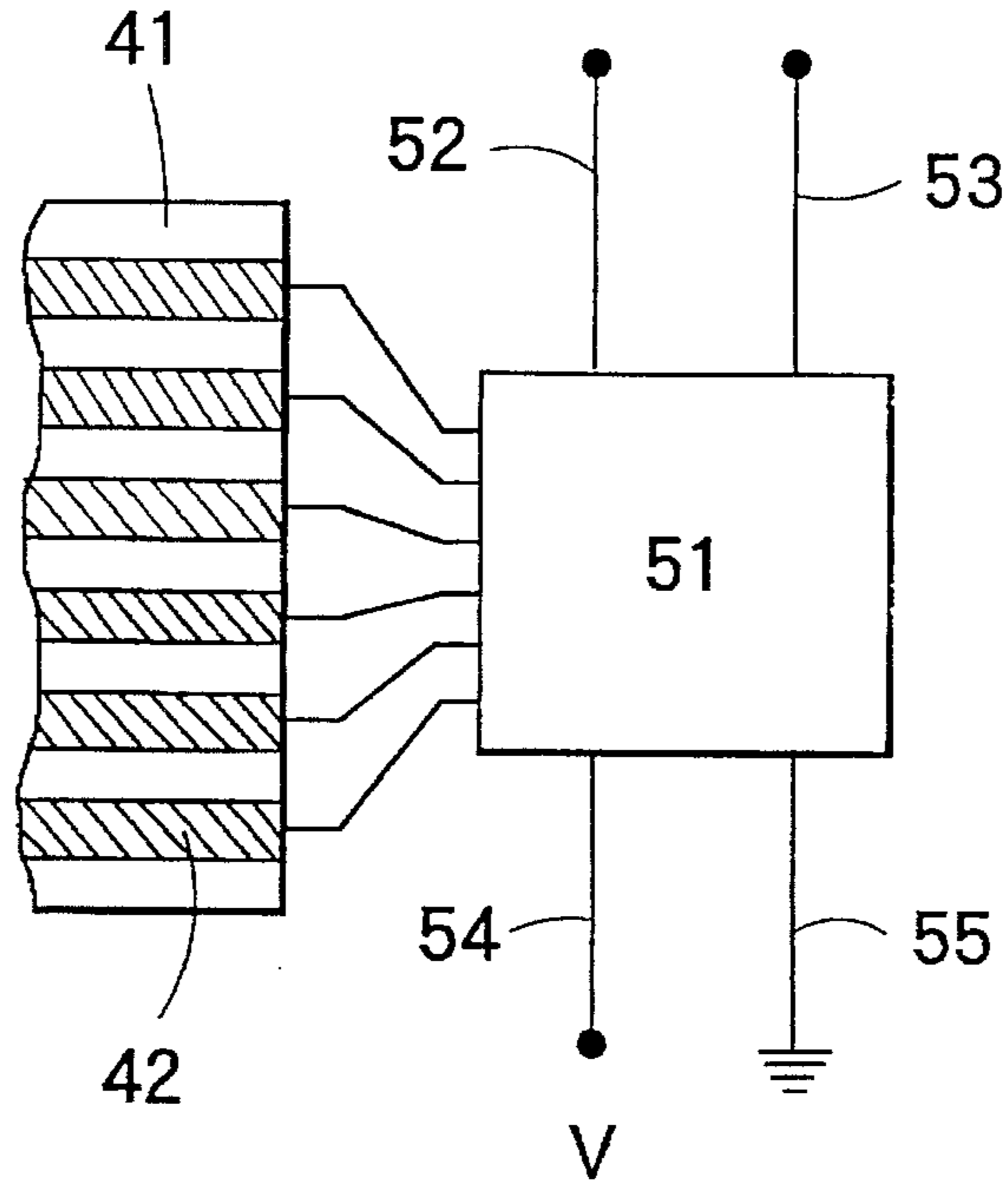
FIG. 4 PRIOR ART
