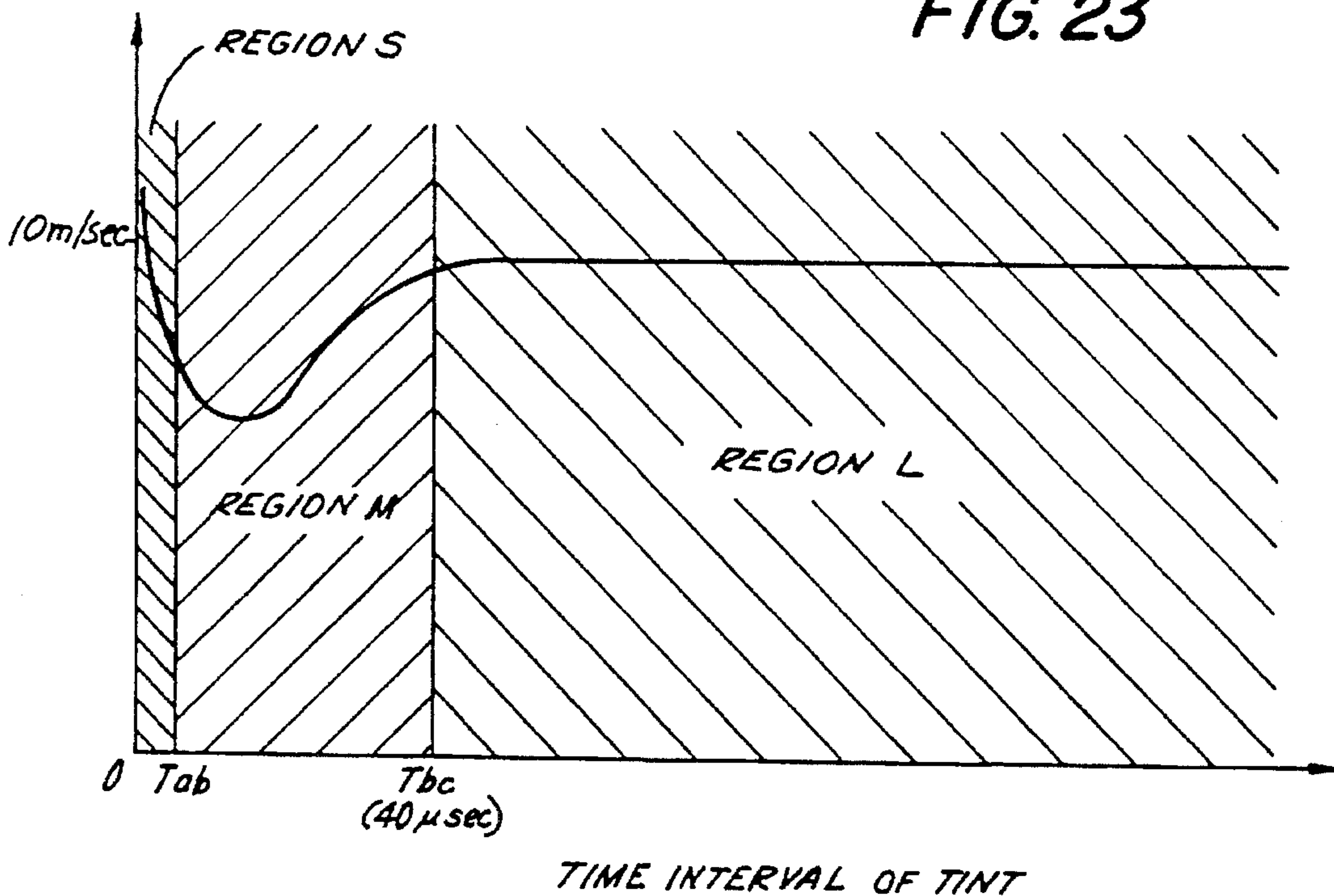
EJECTING SPEED OF INK DROPLETS
