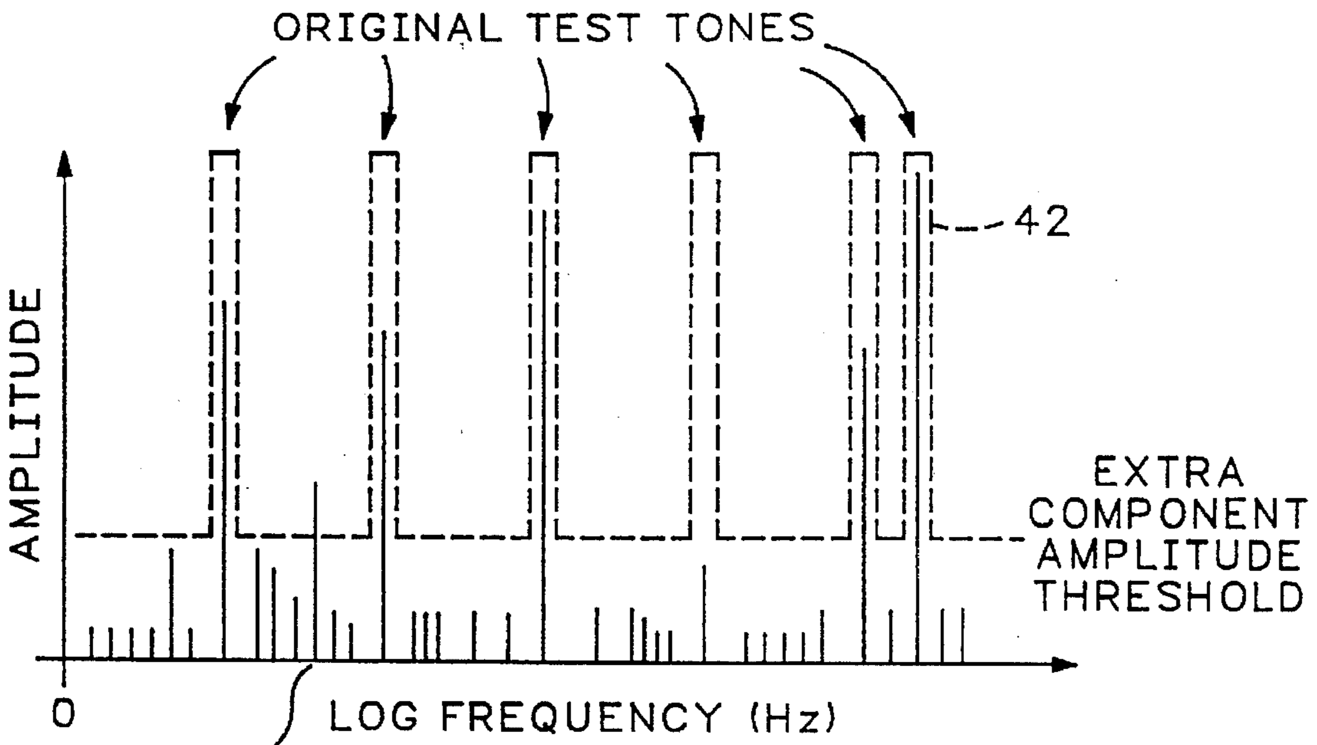
FIG.17B EXTRA COMPONENT
