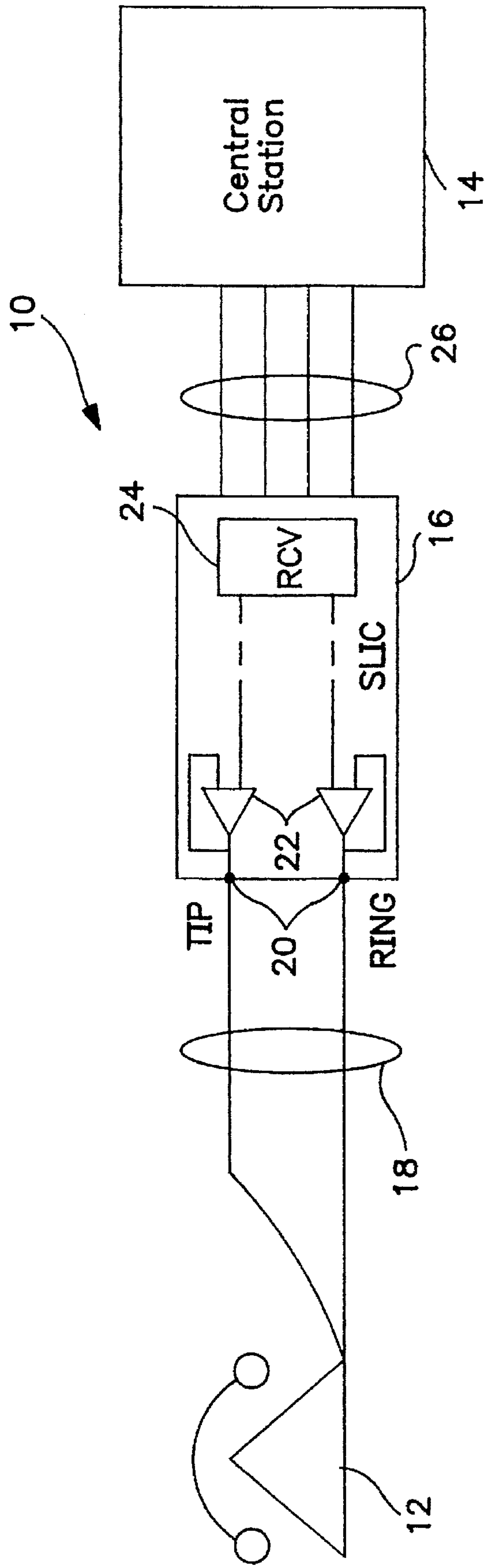
FIG. 1 (Prior Art)
