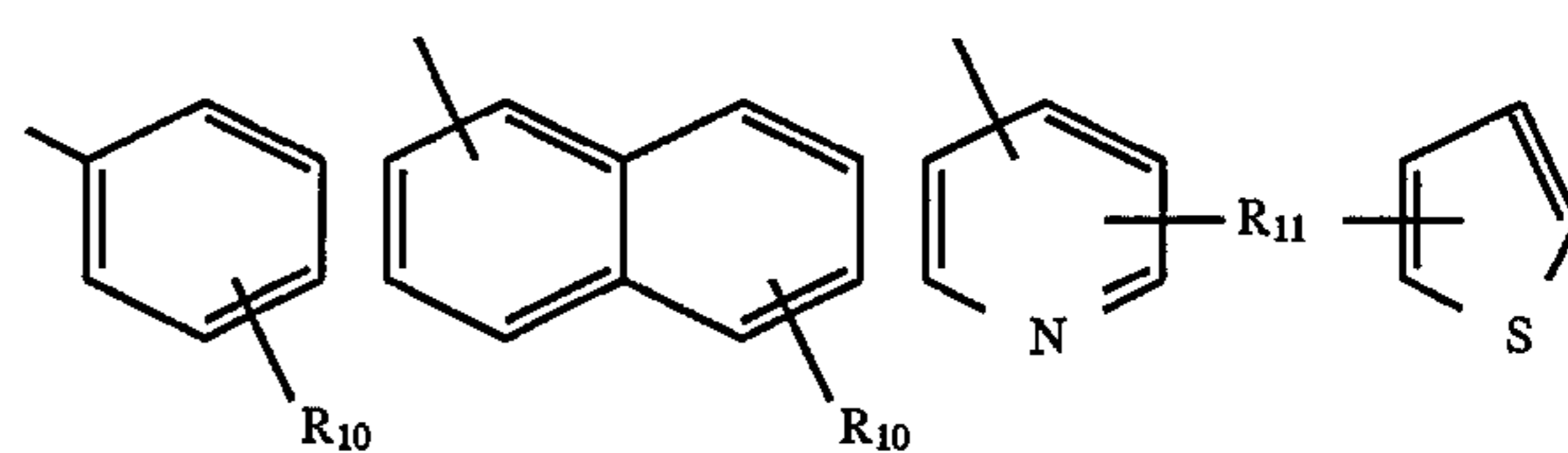
Reaction Scheme K.1
