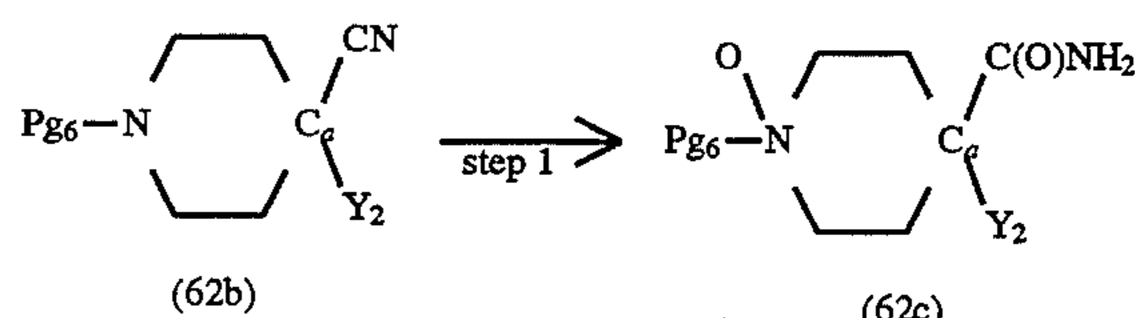
Reaction Scheme K.1
