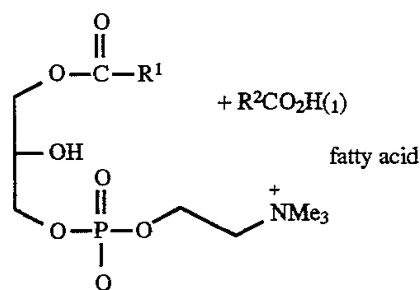
lysophospholipid
