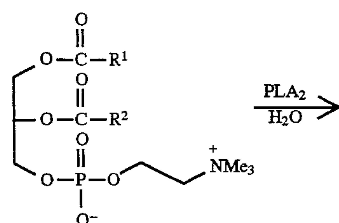
diacylphospholipid
