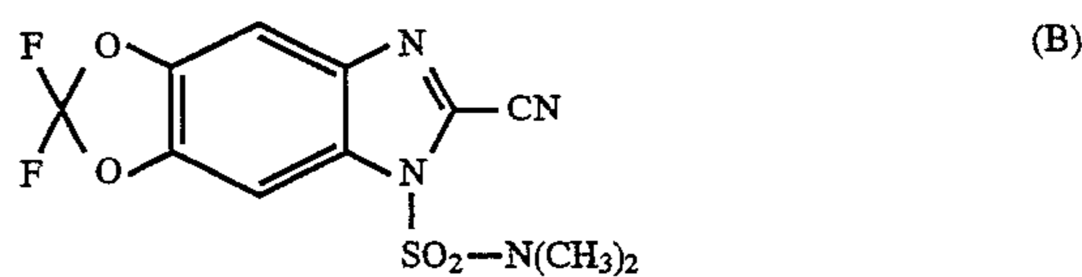
2-cyano-6,6-difluoro-3-dimethylaminosulphonyl-[1,3]dioxolo[4,5-f]benzimidazole
