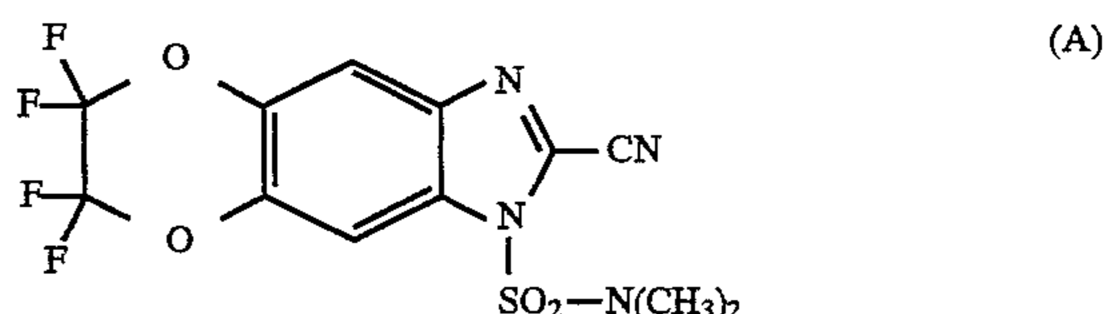
2-cyano-3-dimethylaminosulphonyl-6,6,7,7-tetrafluoro-[1,4]dioxino[2,3-f]benzimidazole
