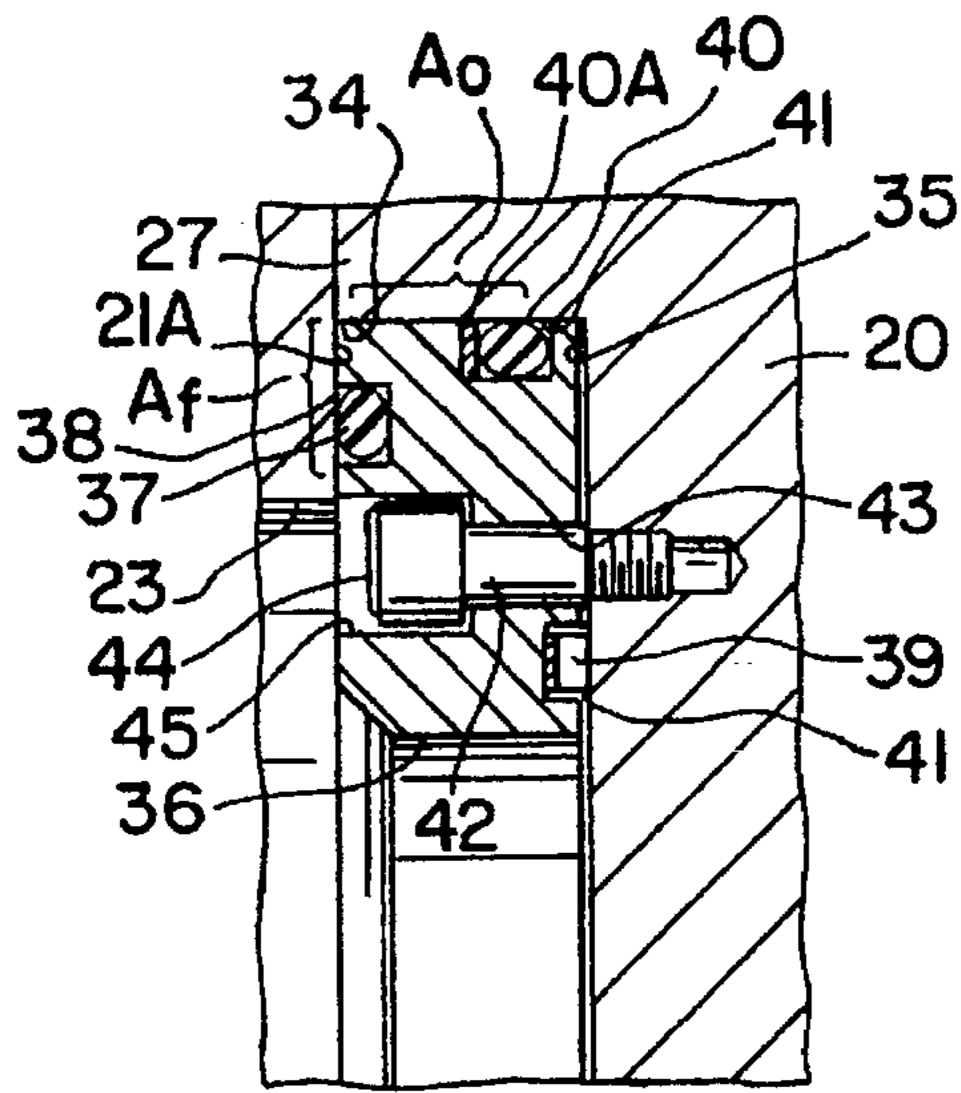
FIG. 3 (PRIOR ART)
