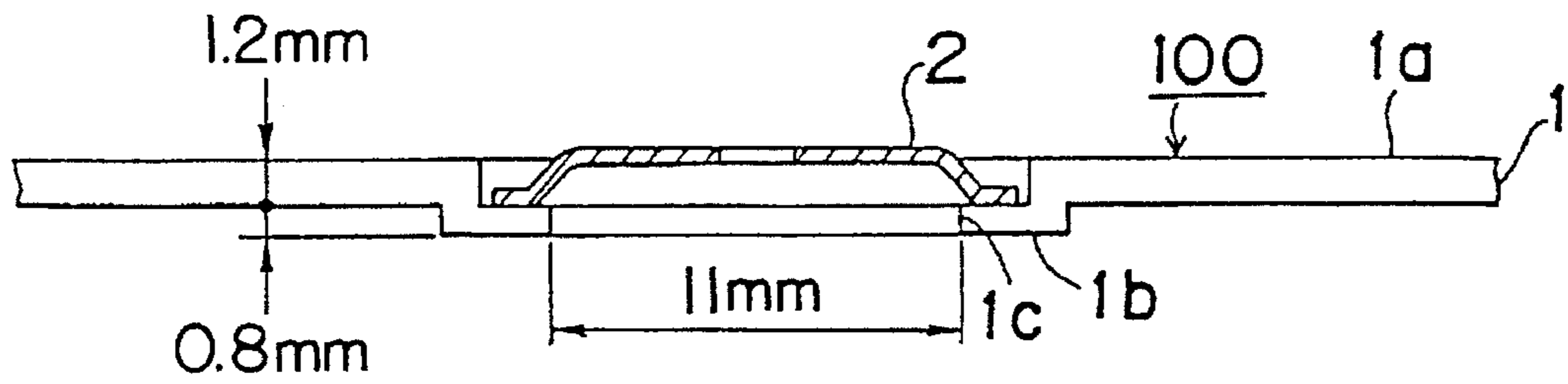
Fig. 8(a) (Prior Art)
