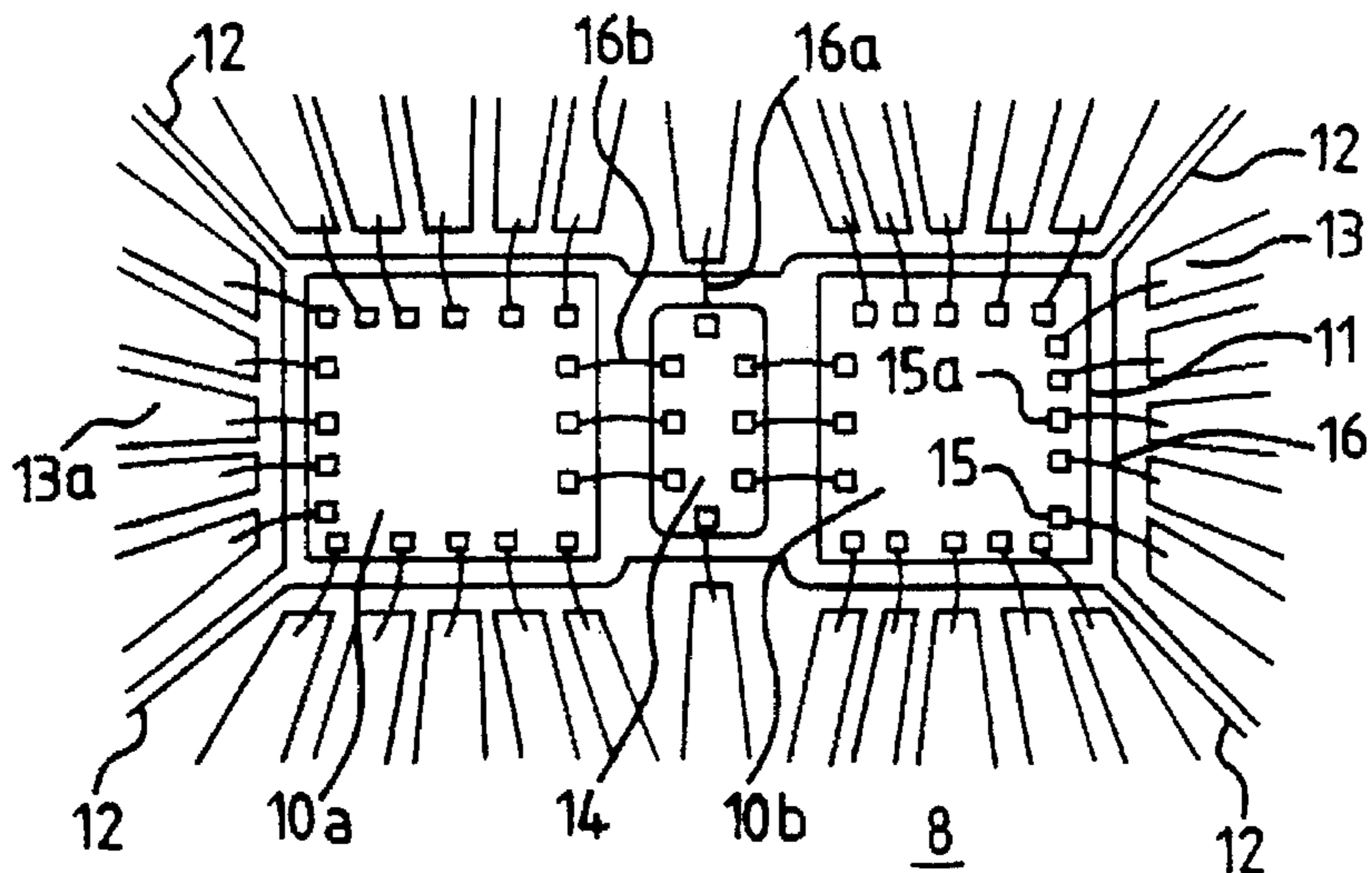
FIG. 1 PRIOR ART
