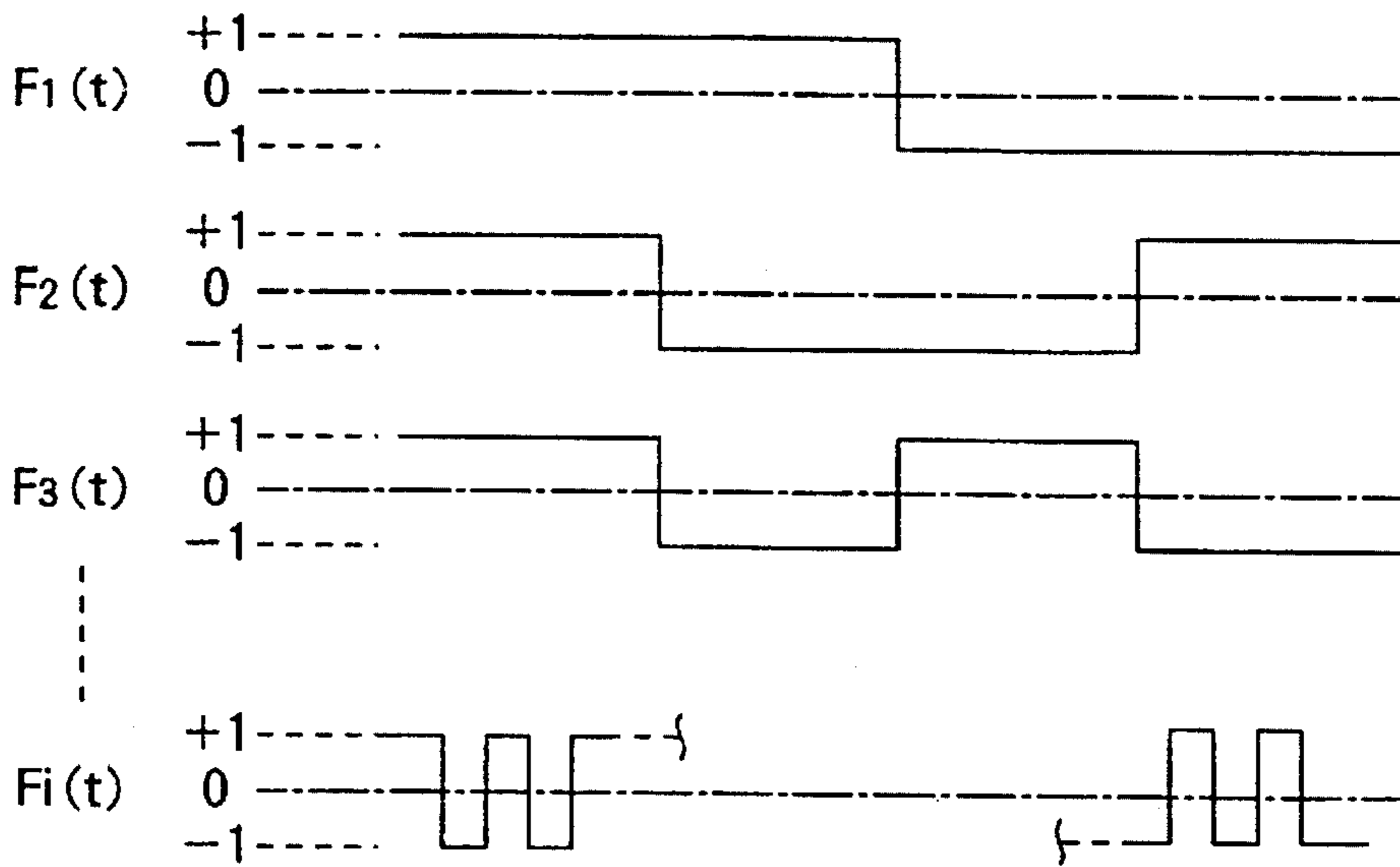
SCANNING WAVEFORM
