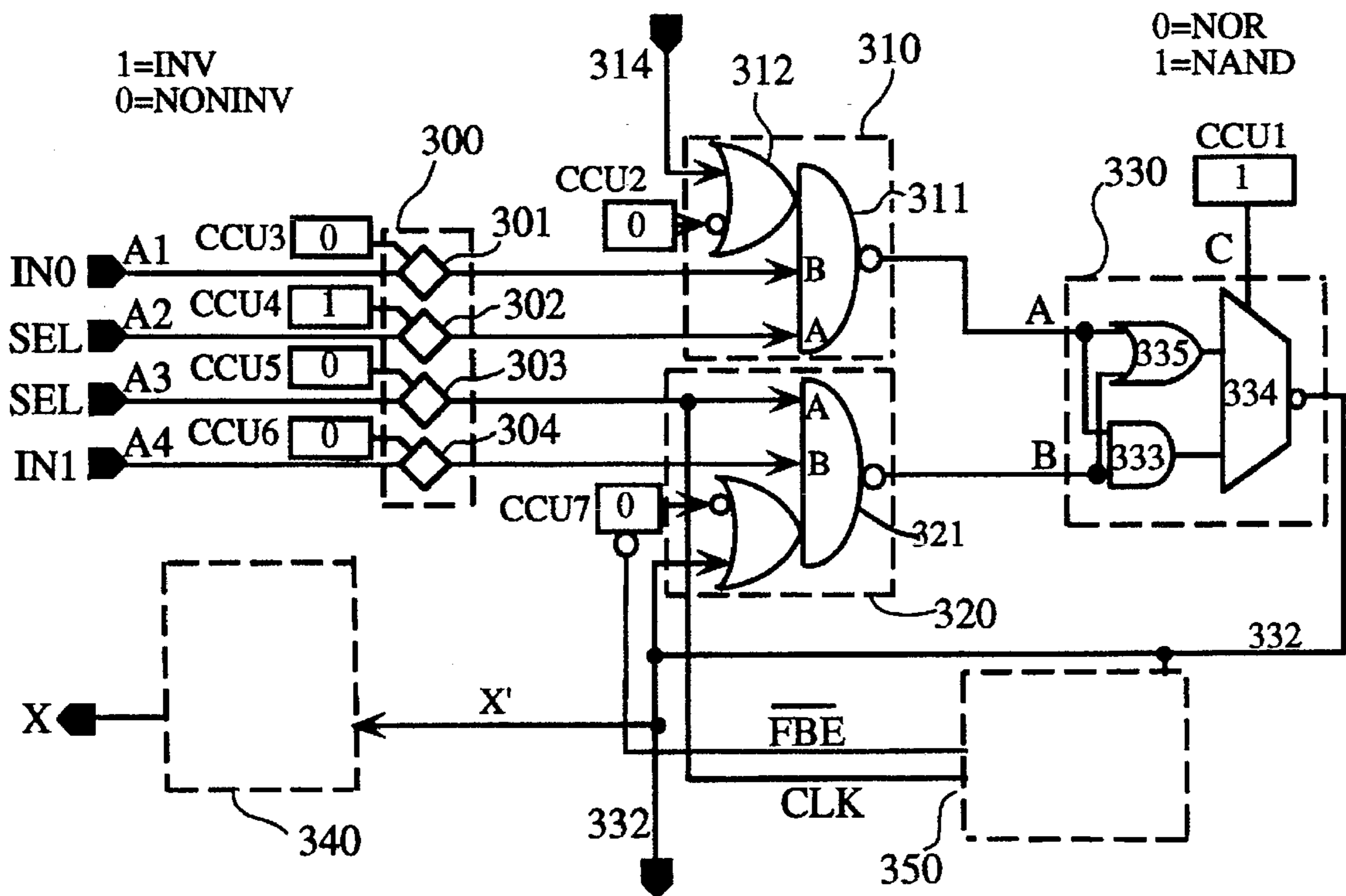
FIG. 5B MULTIPLEXER
