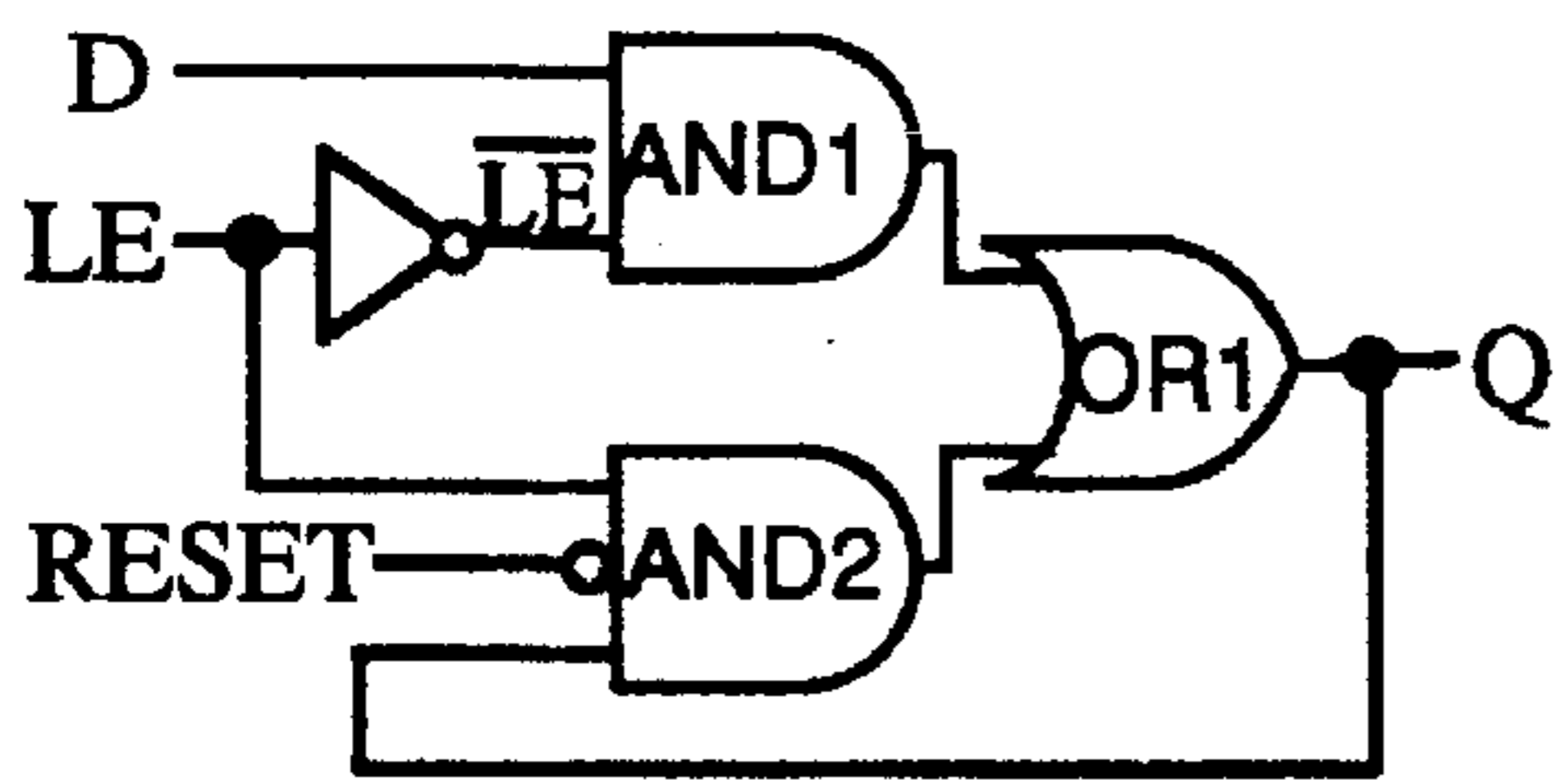
LATCH WITH CLEAR FIG. 9A
