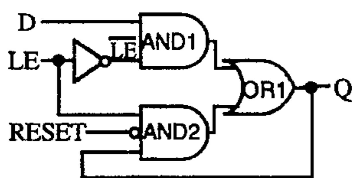
LATCH WITH CLEAR
