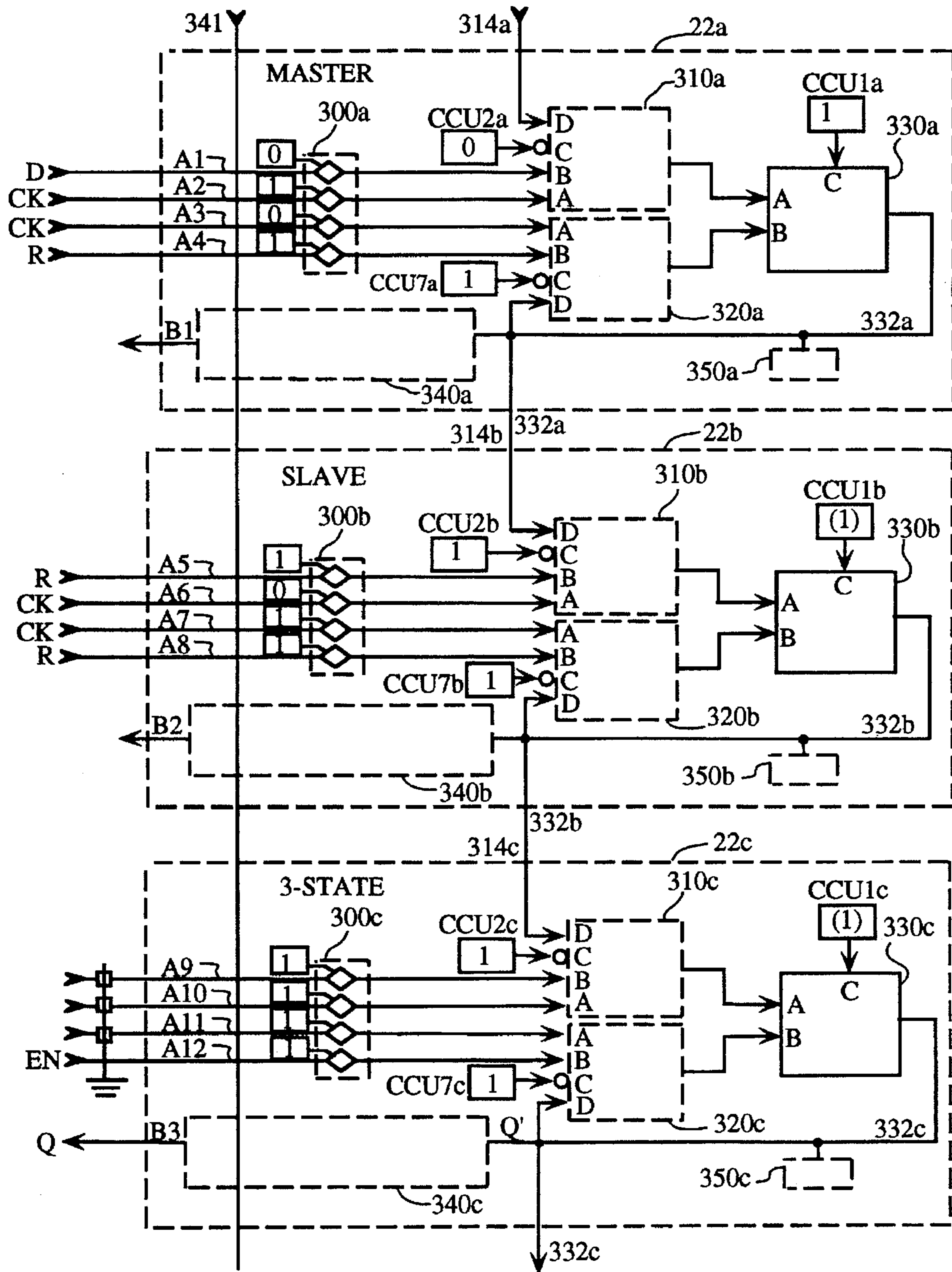
FIG. 21B D FLIP FLOP WITH 3-STATE
