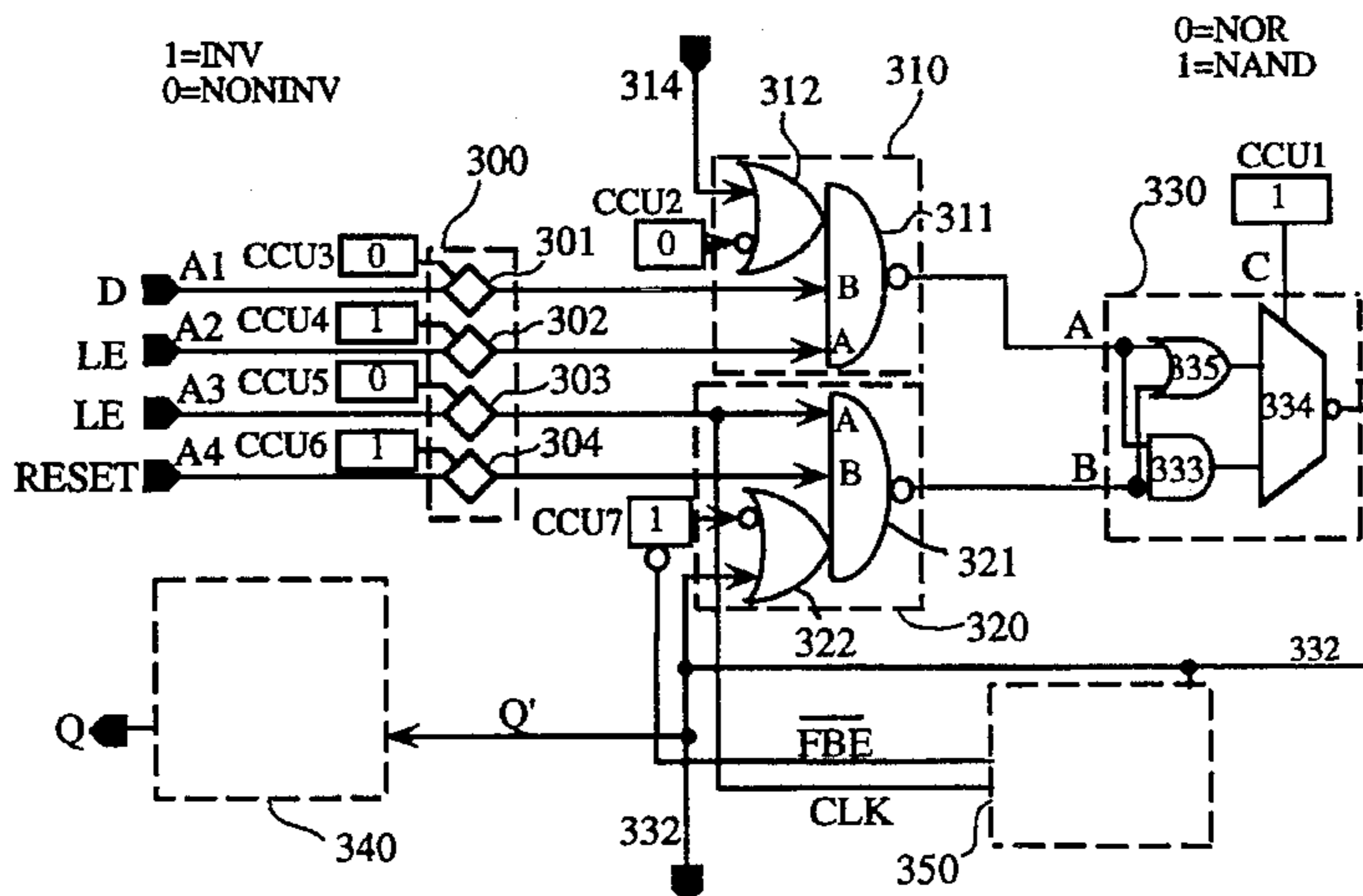
LATCH WITH CLEAR
