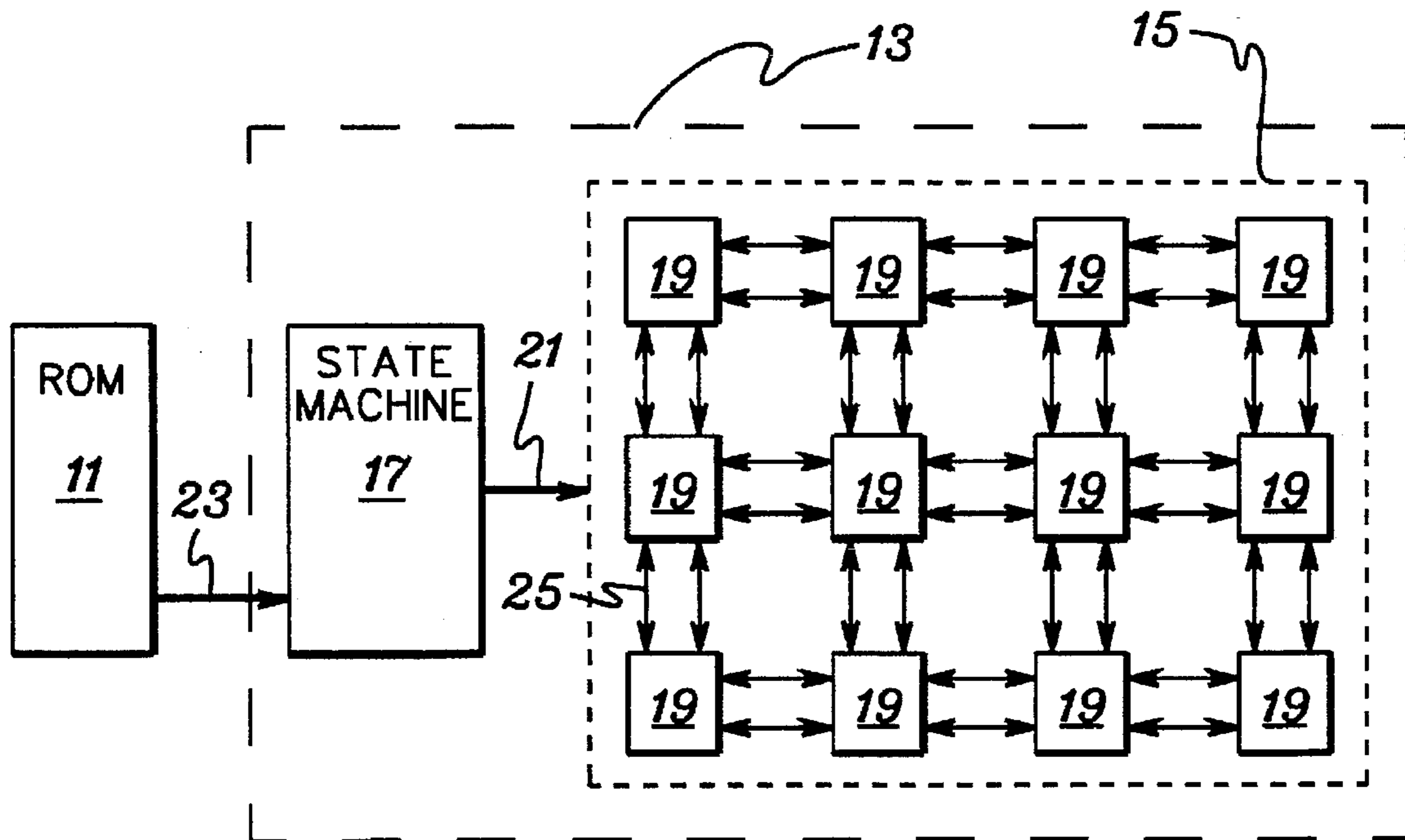
fig. 1 (PRIOR ART)
