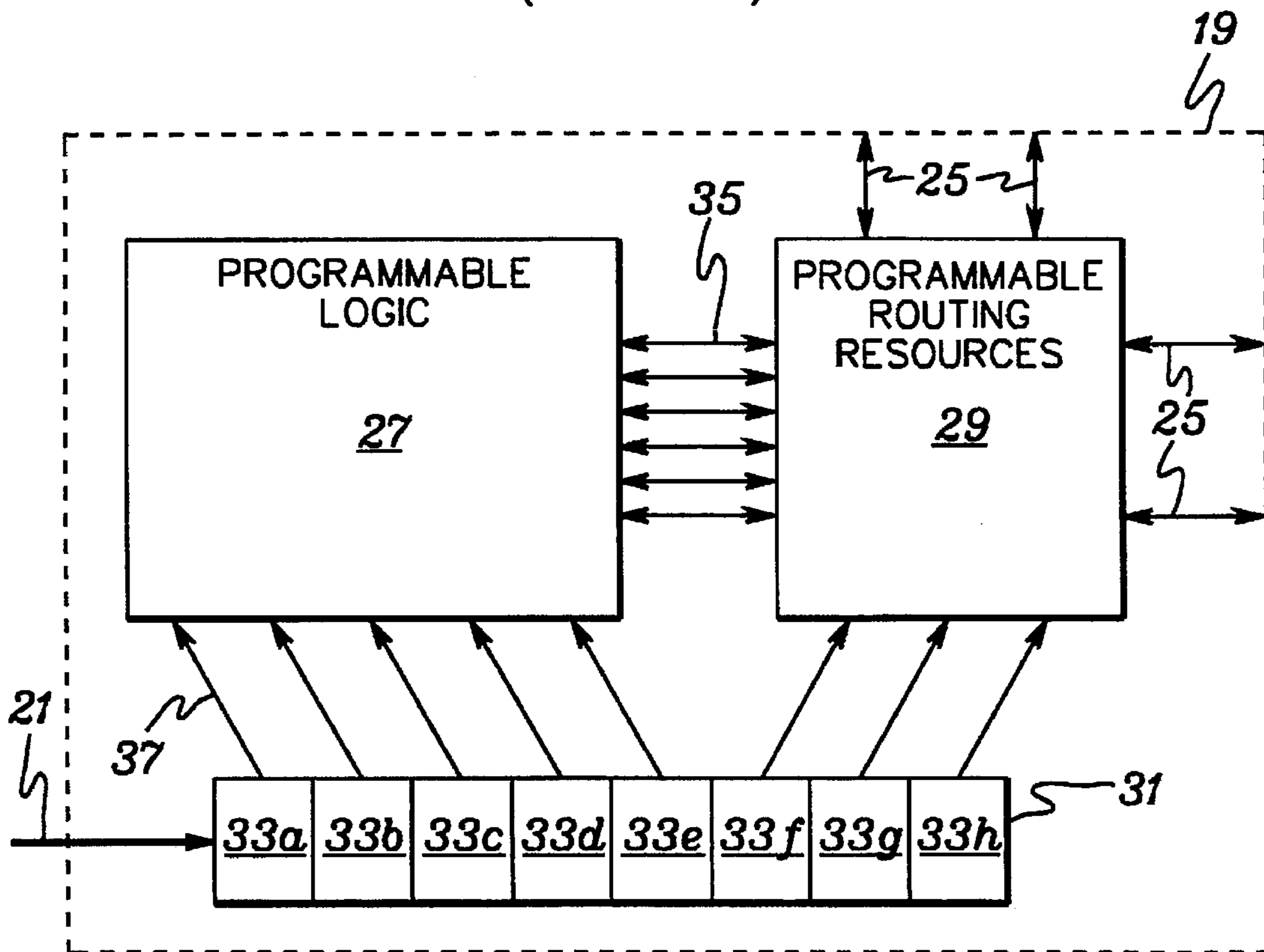
fig. 2 (PRIOR ART)
