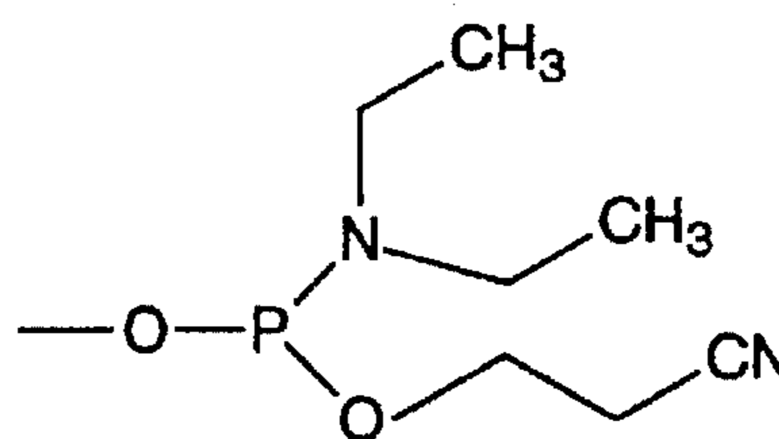
N,N-diethylamino-β-cyanoethoxyphosphine
