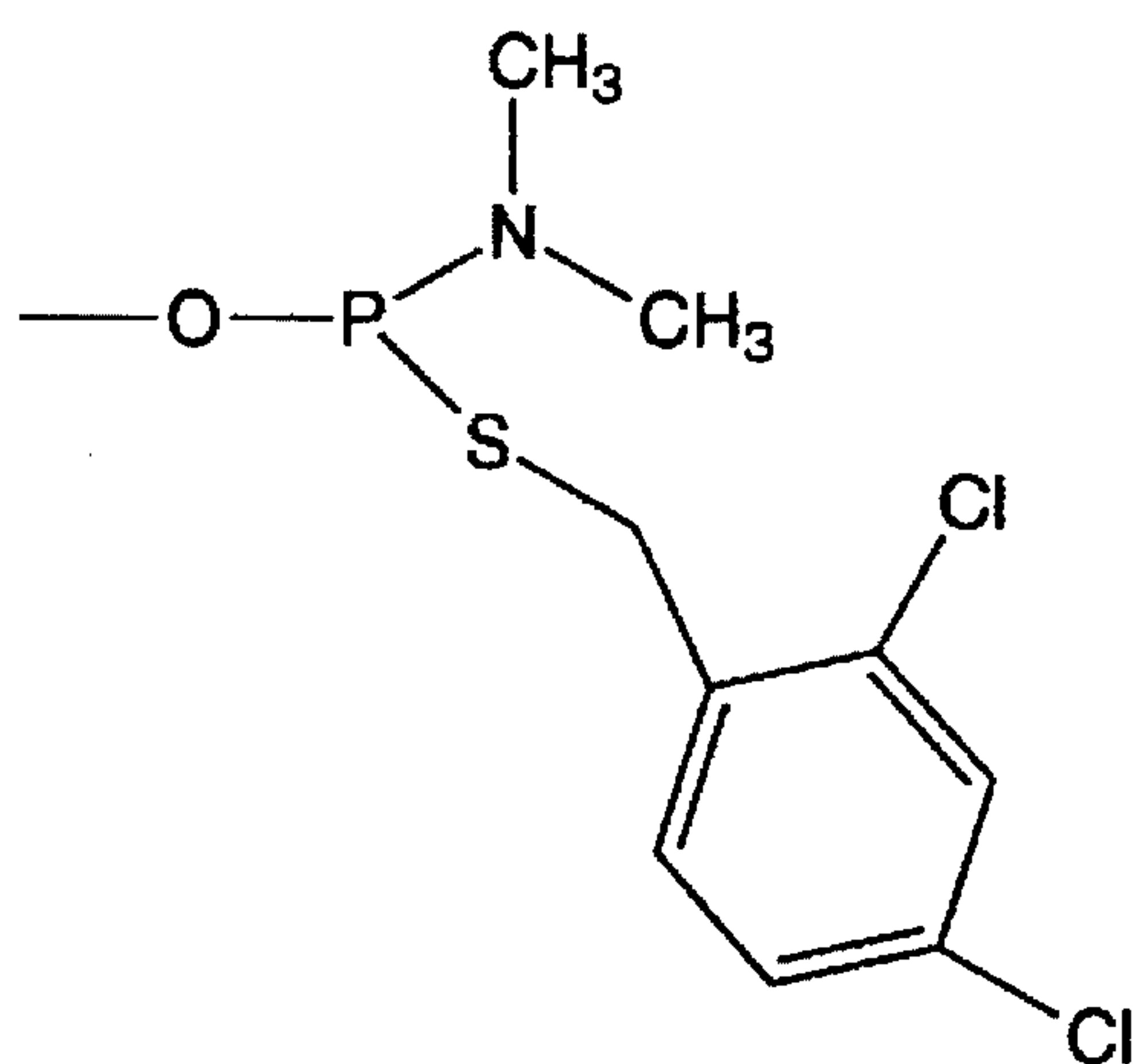
N,N-dimethylamino- 2,4-dichlorobenzylmercapto- phosphine
