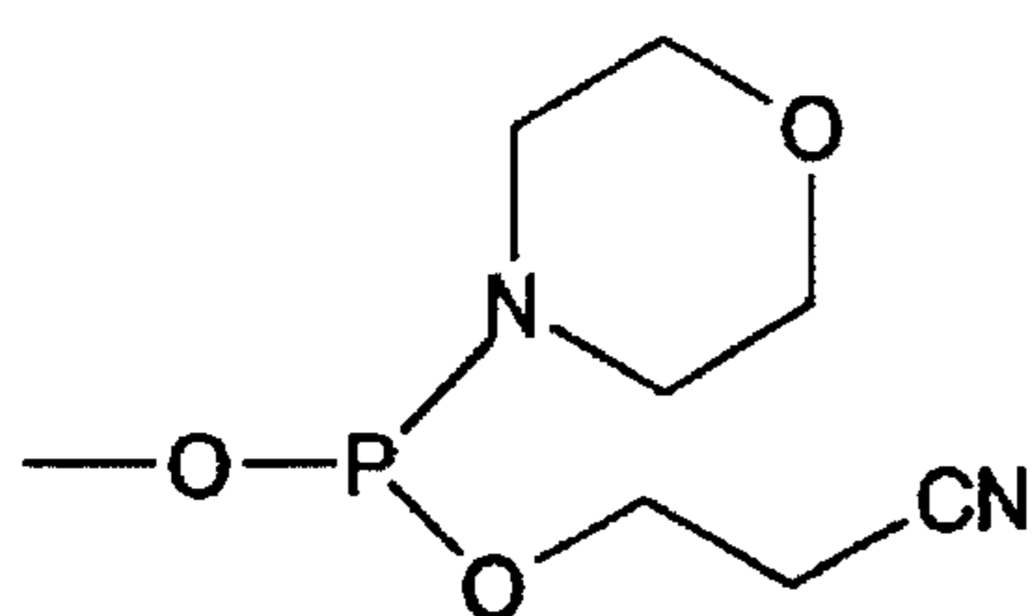
N-morpholino-β-cyanoethoxyphosphine
