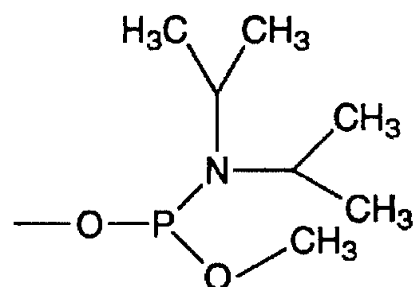
N,N-diisopropylamino-methoxy- phosphine
