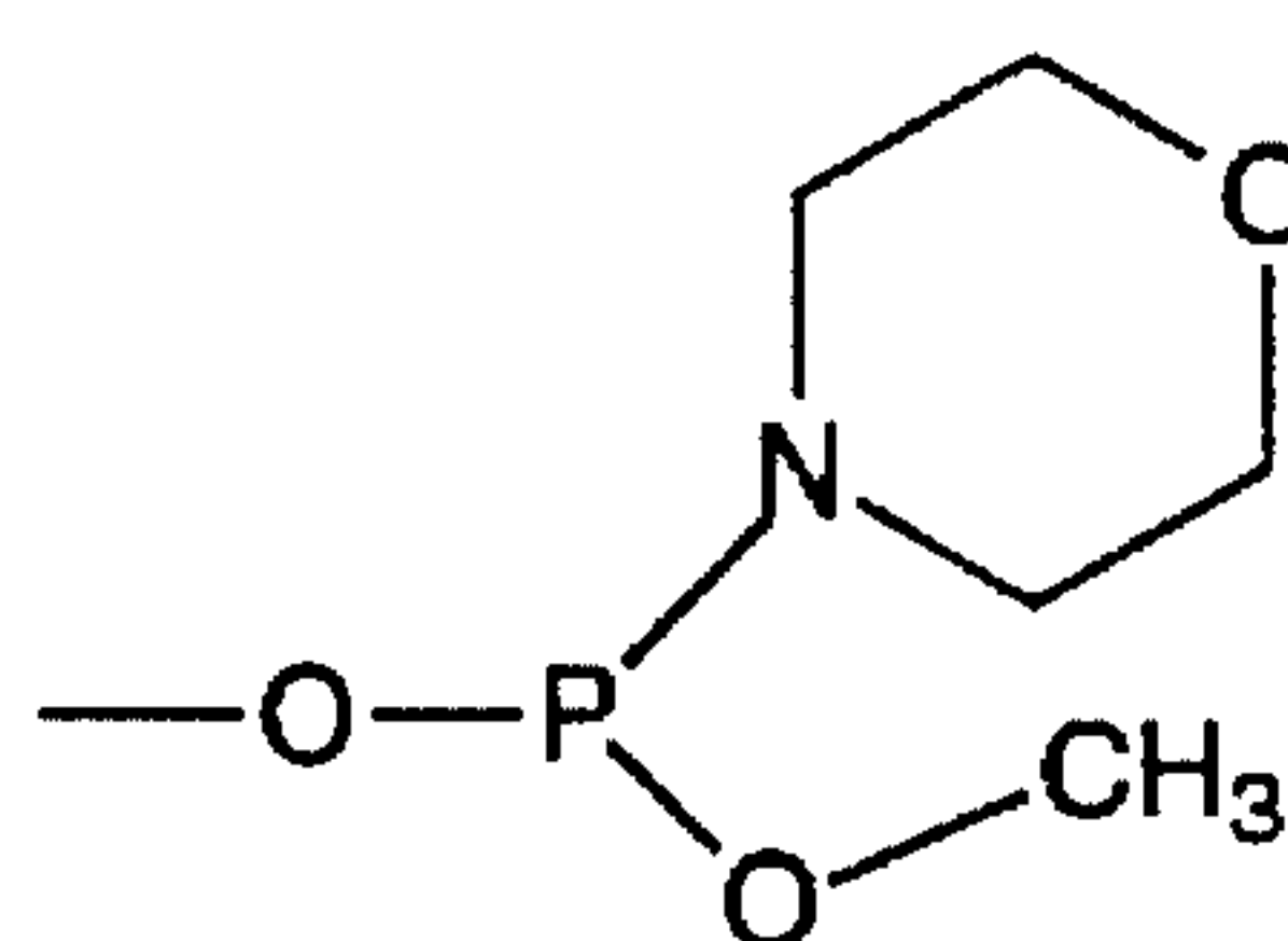
N-morpholino methoxyphosphine
