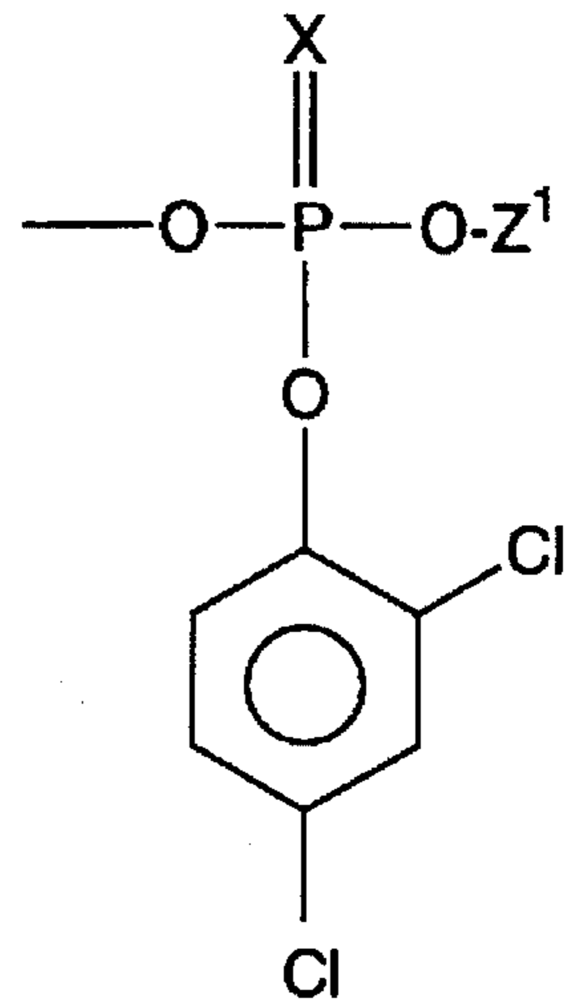
2,4-dichlorophenyl phosphate
