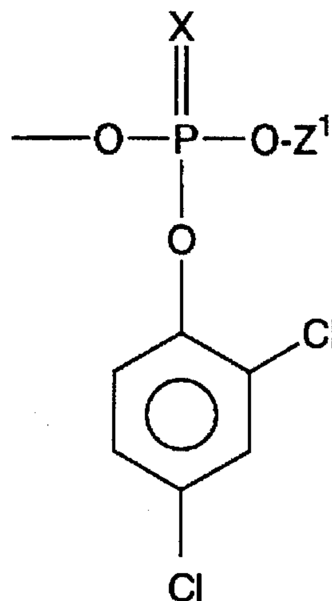
2,4-dichlorophenyl phosphate
