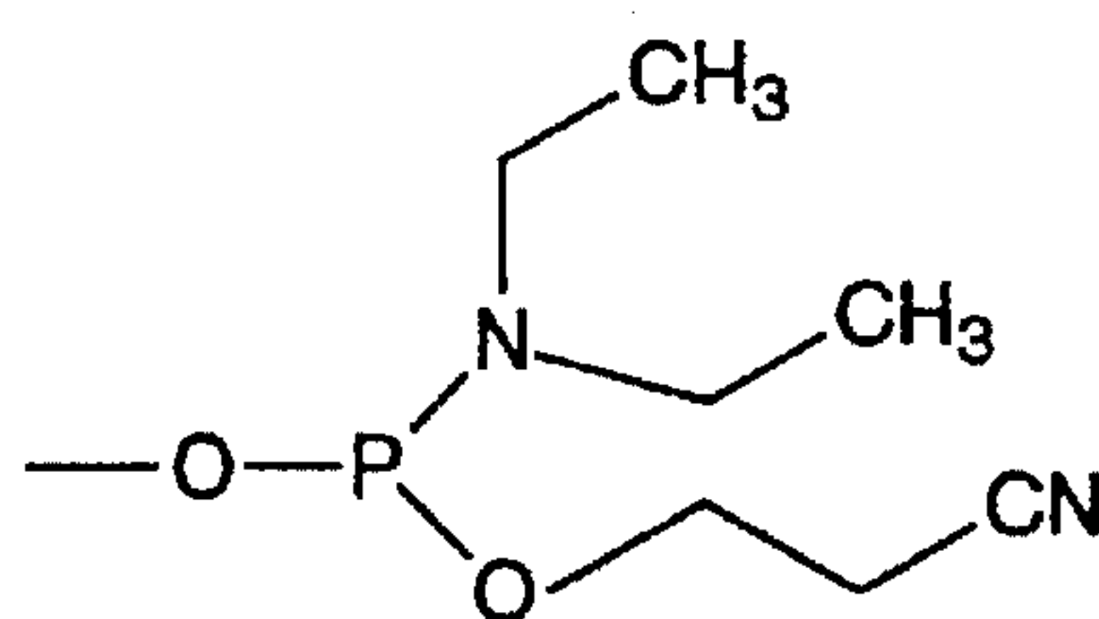
N,N-diethylamino- \beta -cyanoethoxy phosphine
