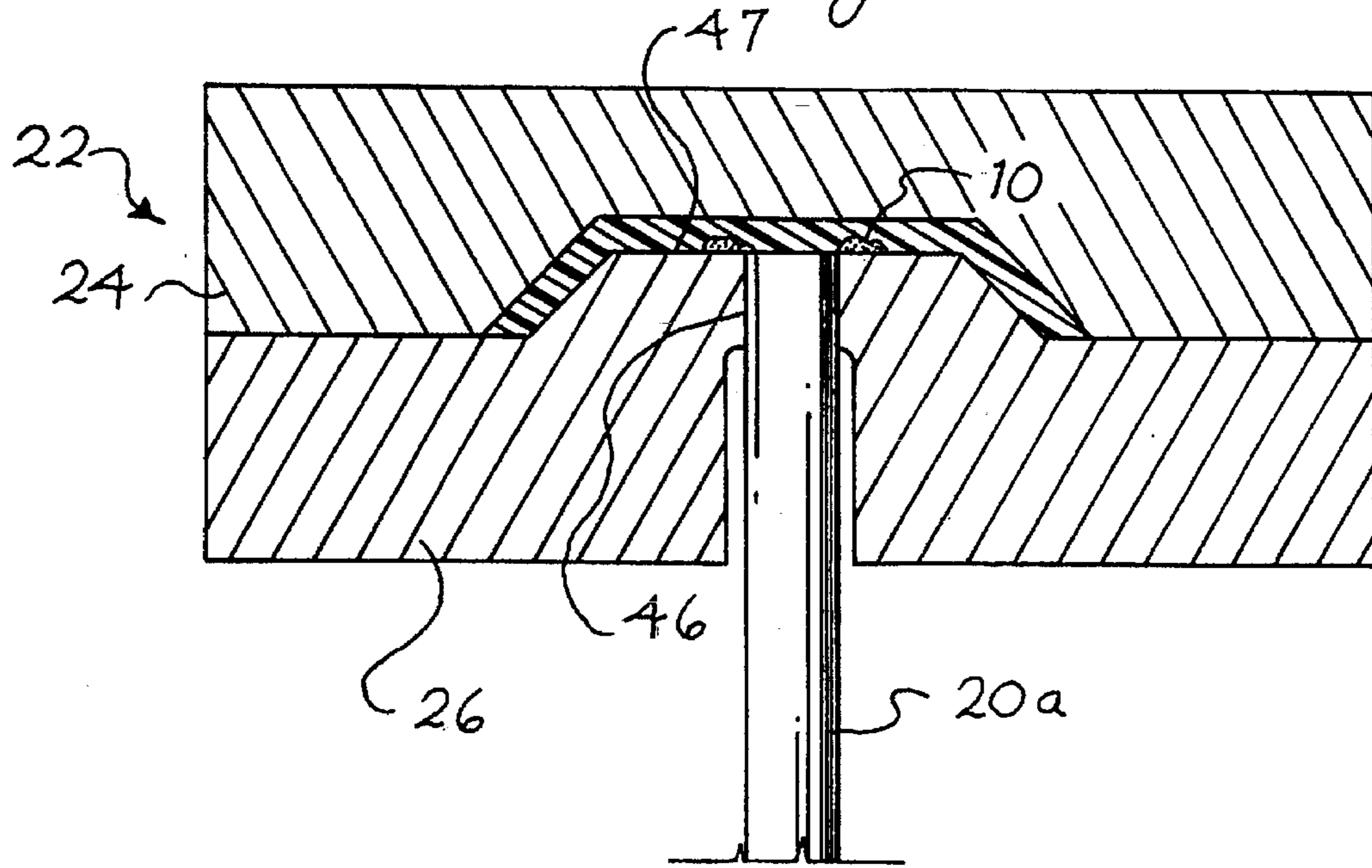
Fig. 5 (PRIOR ART)
