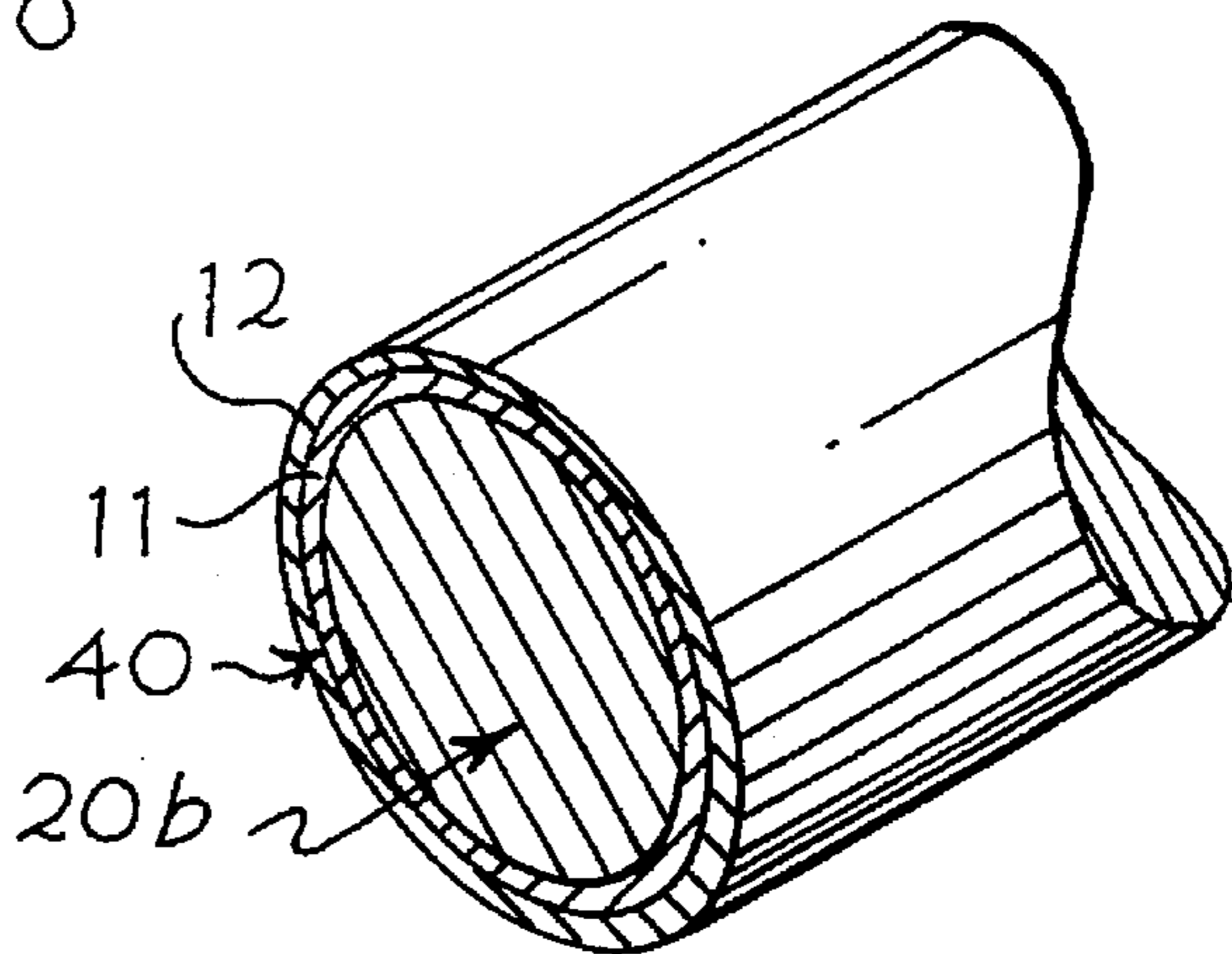
Fig. 8 (PRIOR ART)
