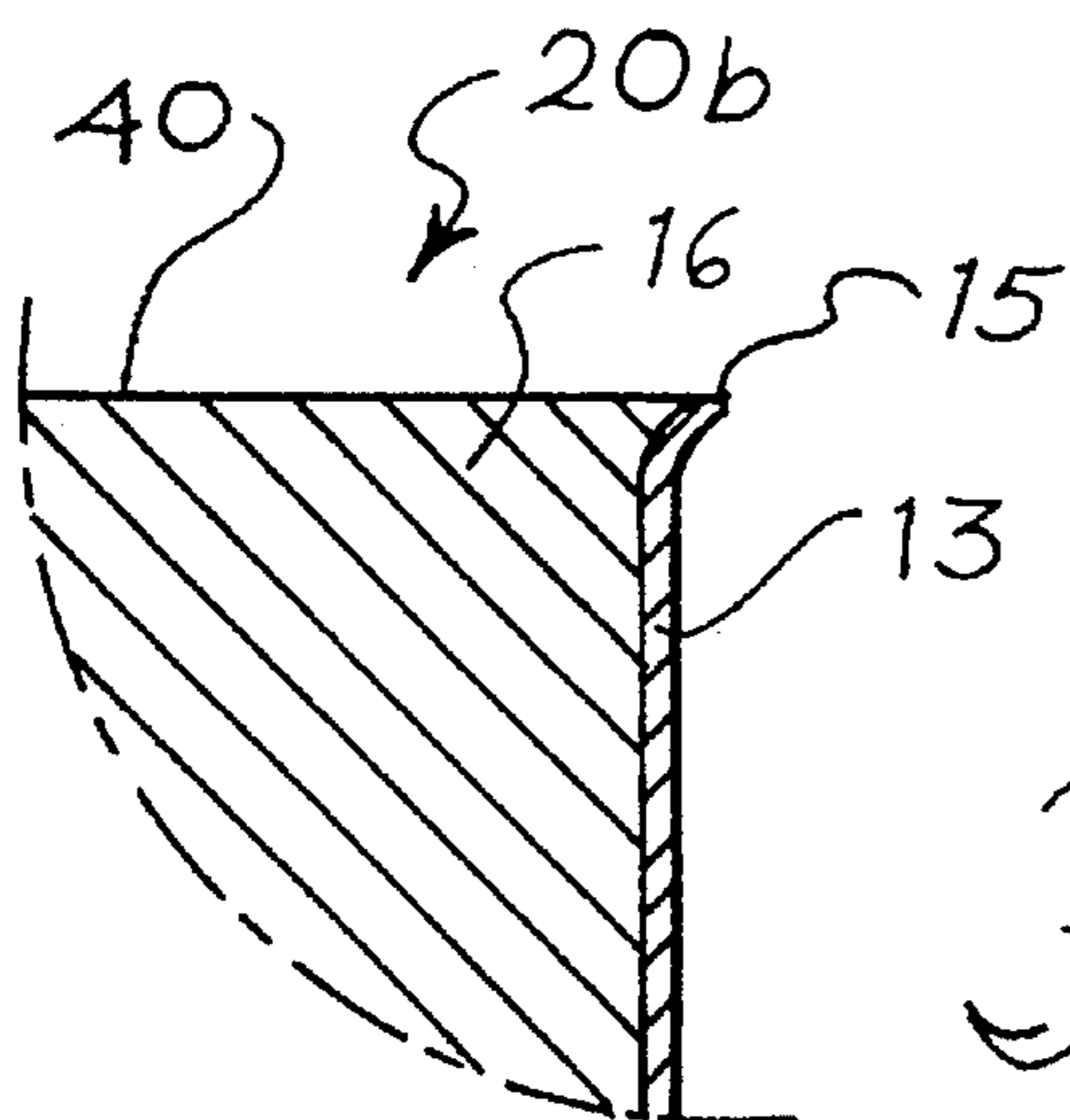
Fig. 8 (PRIOR ART)
