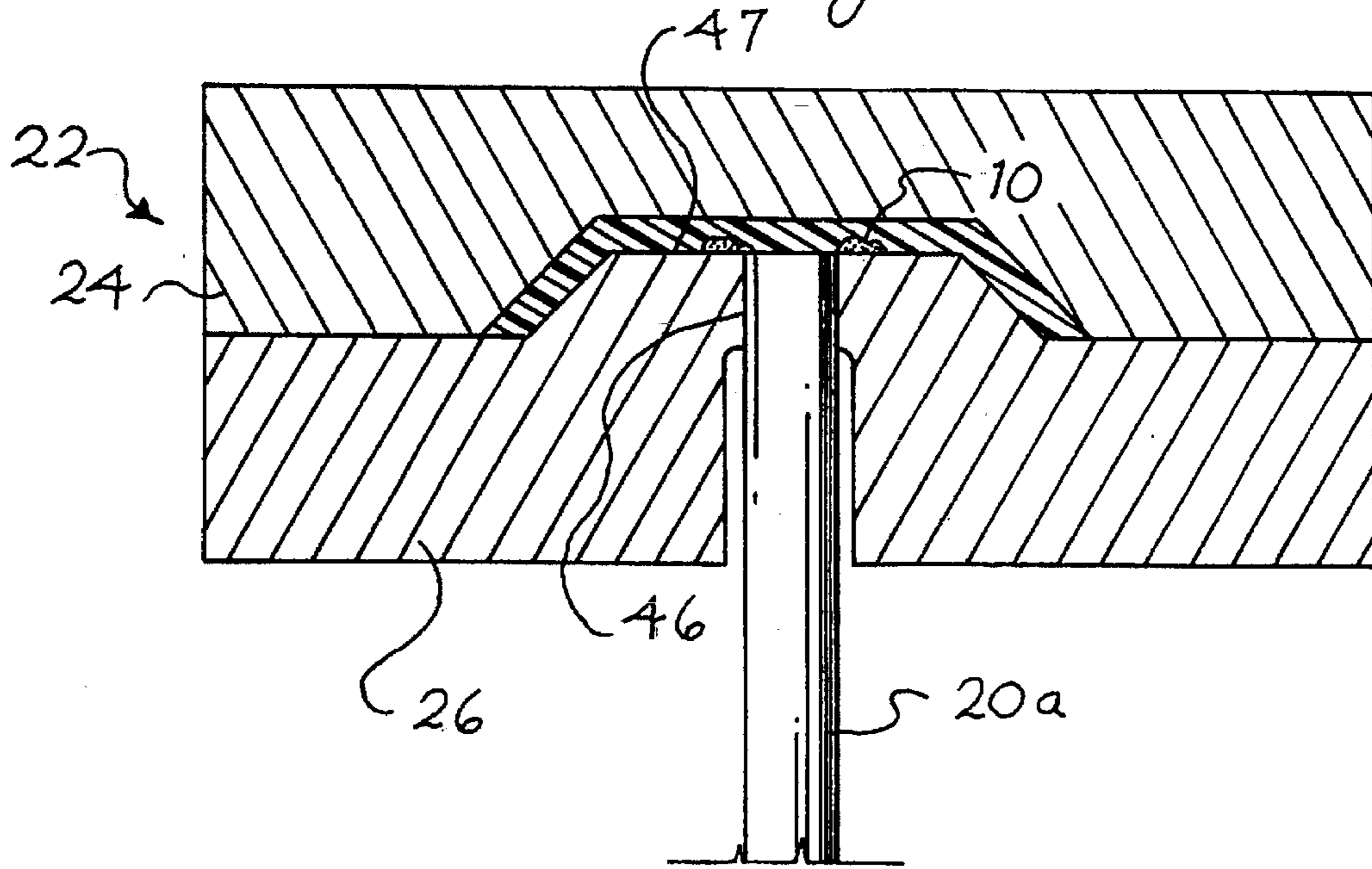
Fig. 5 (PRIOR ART)
