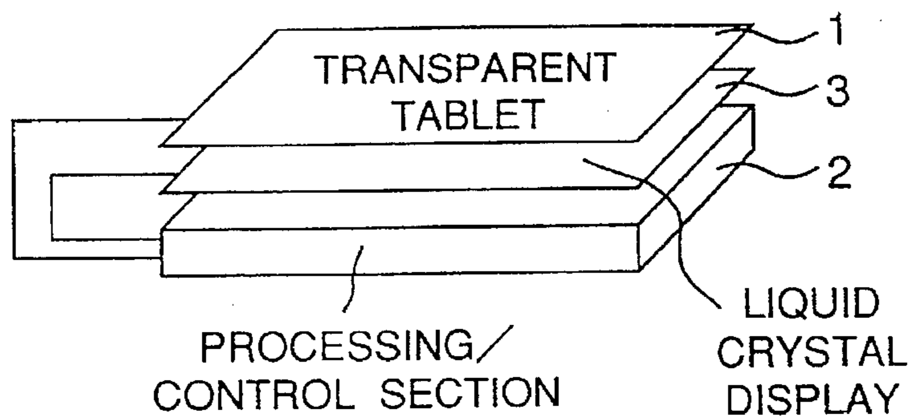
Fig. 11 PRIOR ART
