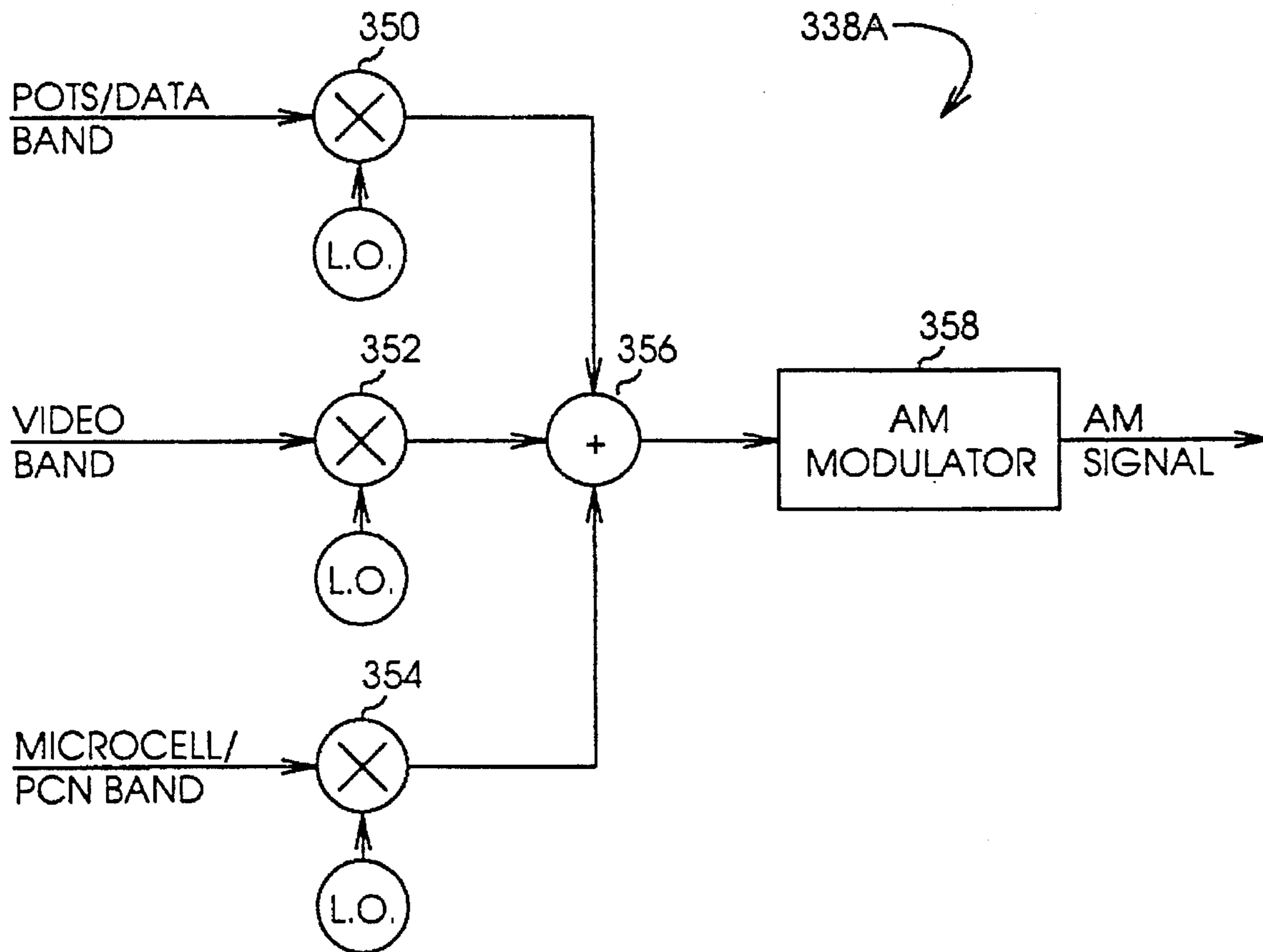
AM Modulator
