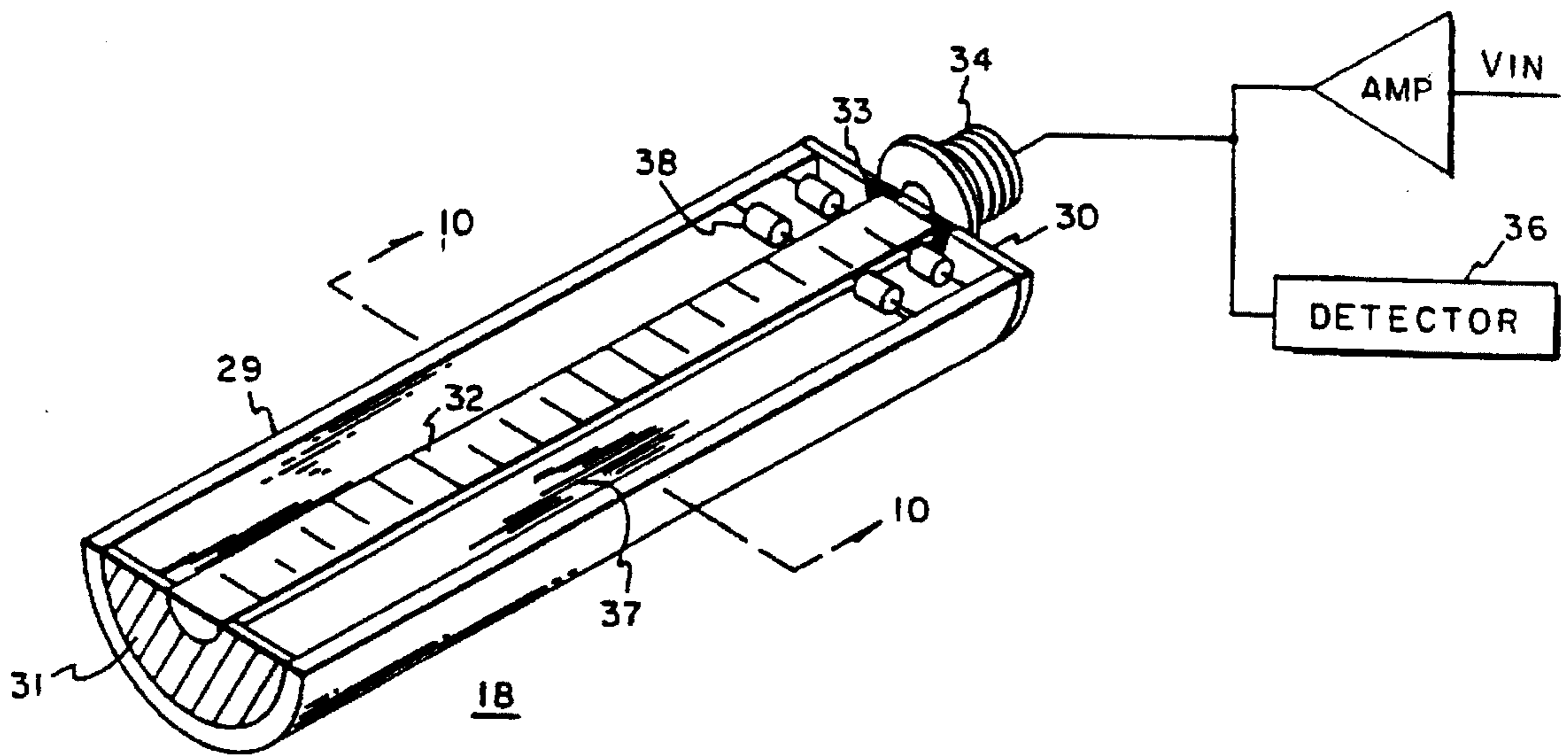
FIG. 3 (PRIOR ART)
