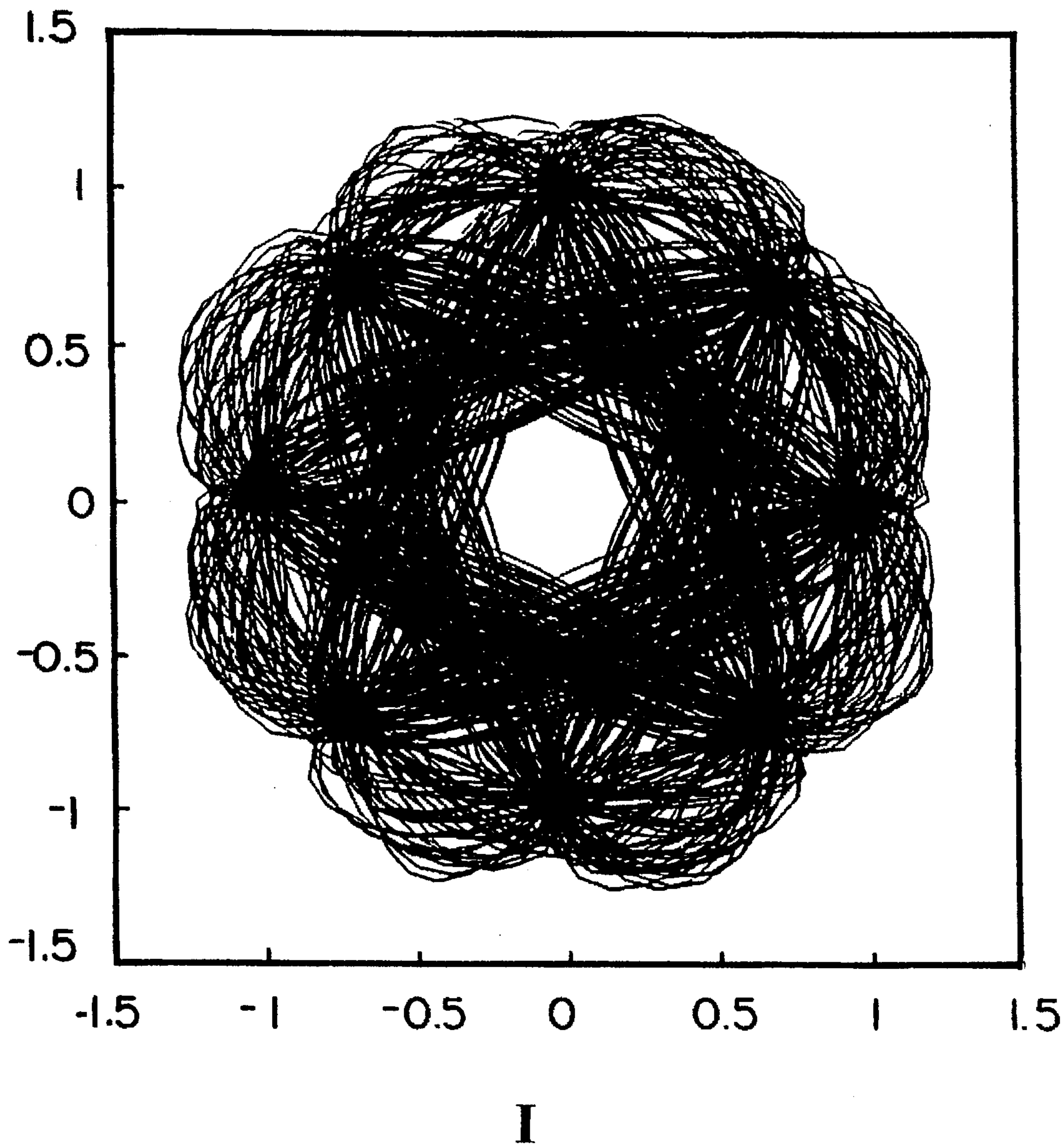
I vs. Q plot for \pi/4 -shifted DQPSK
