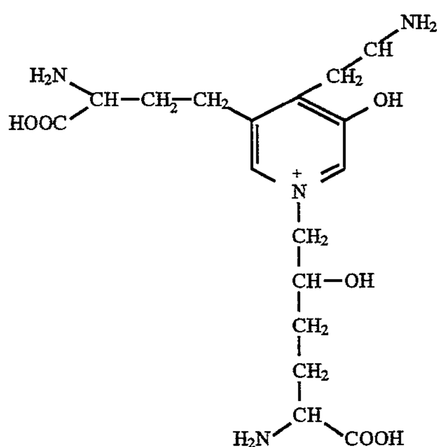
hydroxylysyl pyridinoline (HP)
