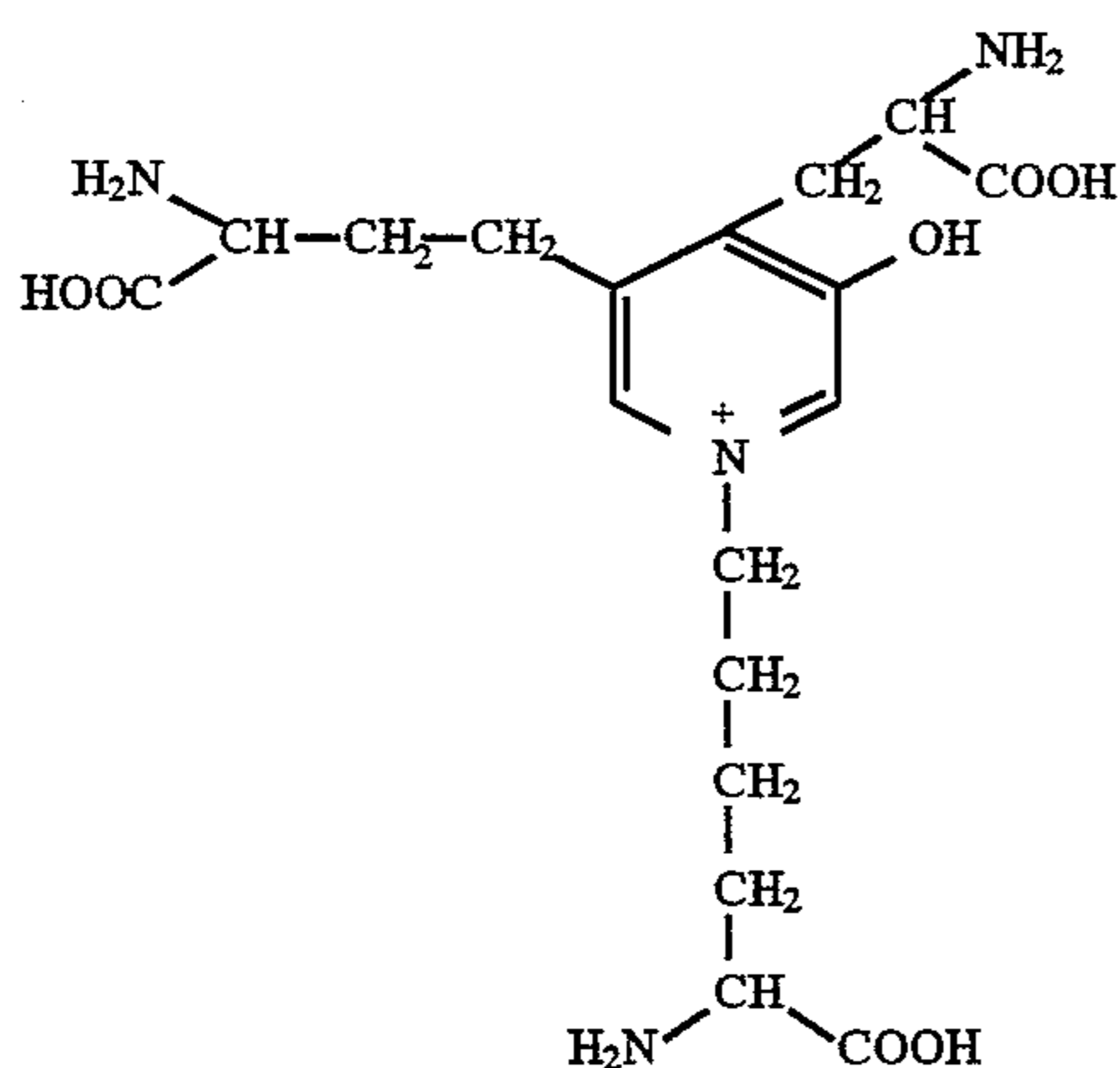
lysyl pyridinoline (LP)
