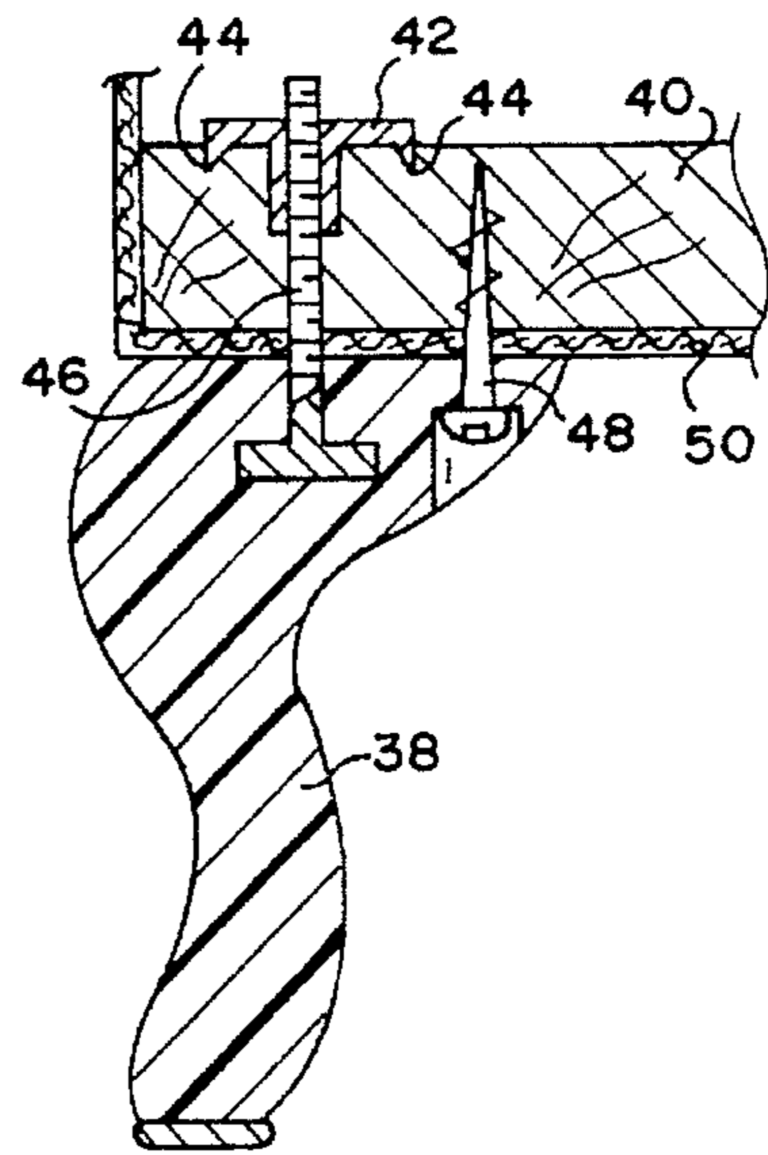
FIG. 3 PRIOR ART
