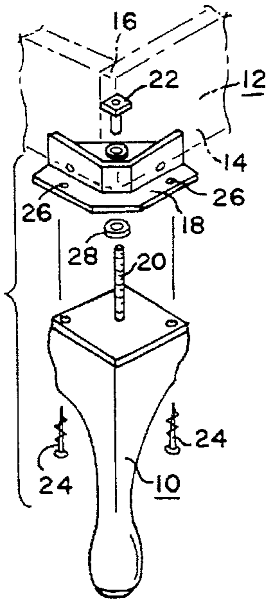
FIG. 1 PRIOR ART
