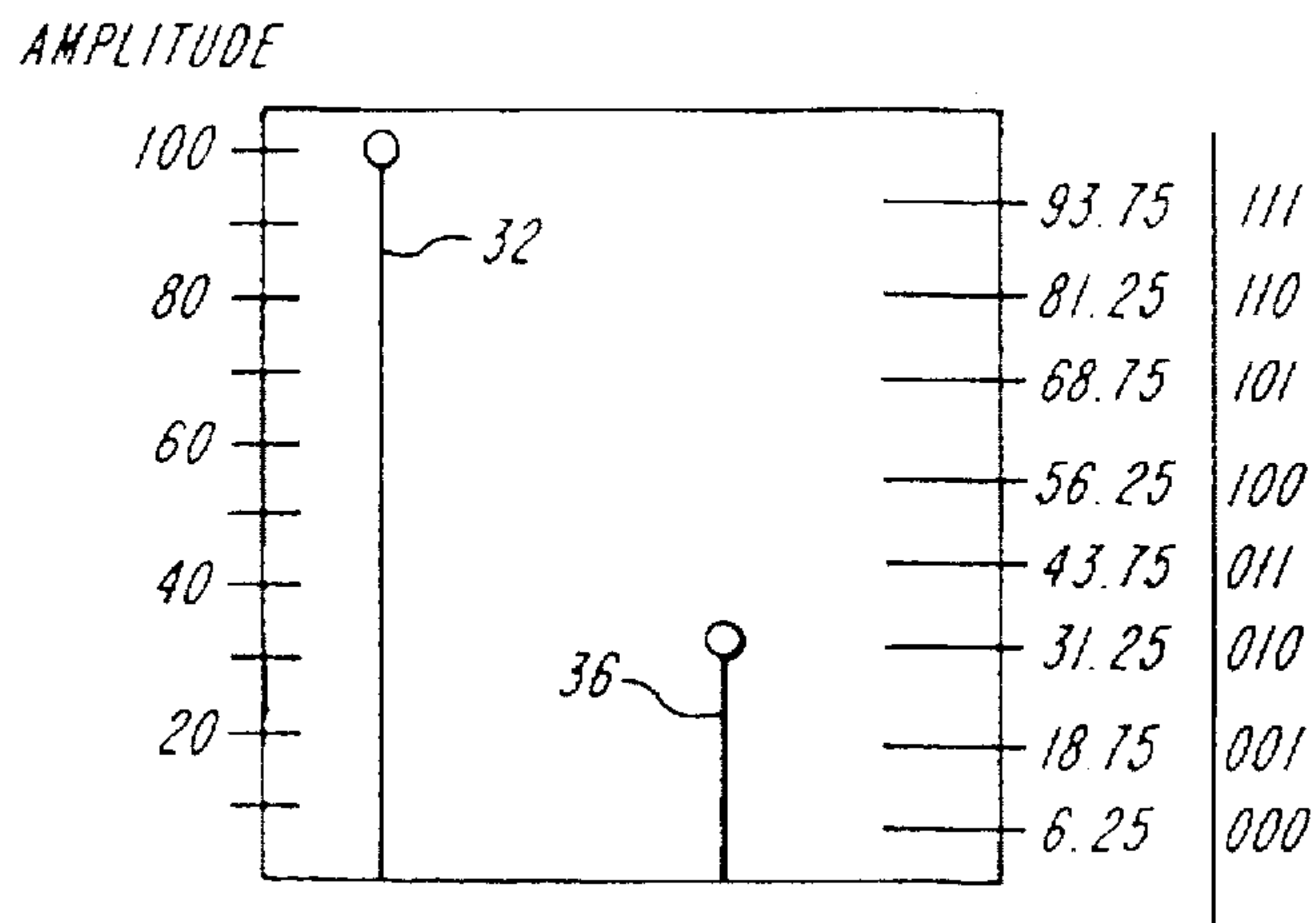
FIG. 5 ( PRIOR ART )
