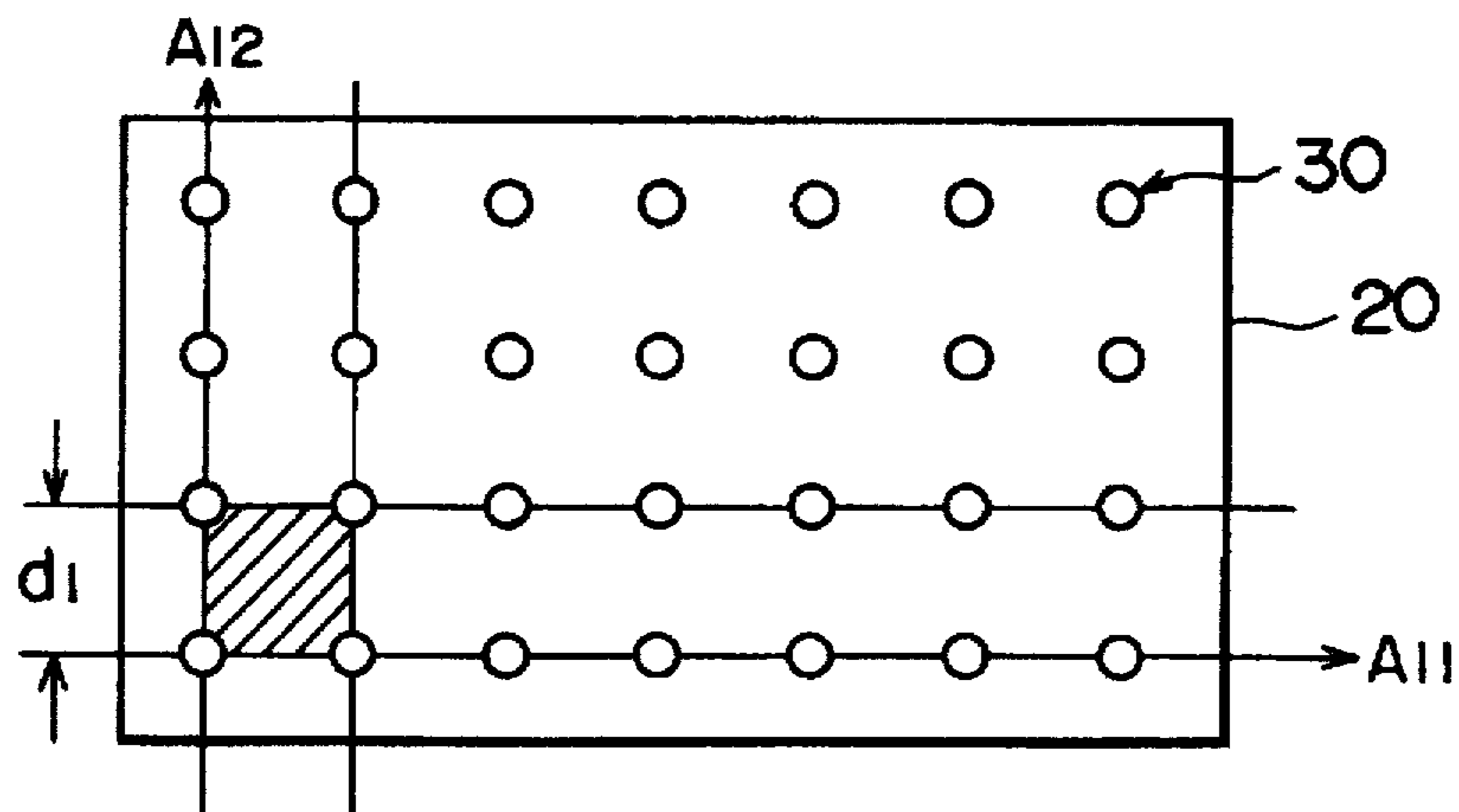
FIG. 1C (PRIOR ART)
