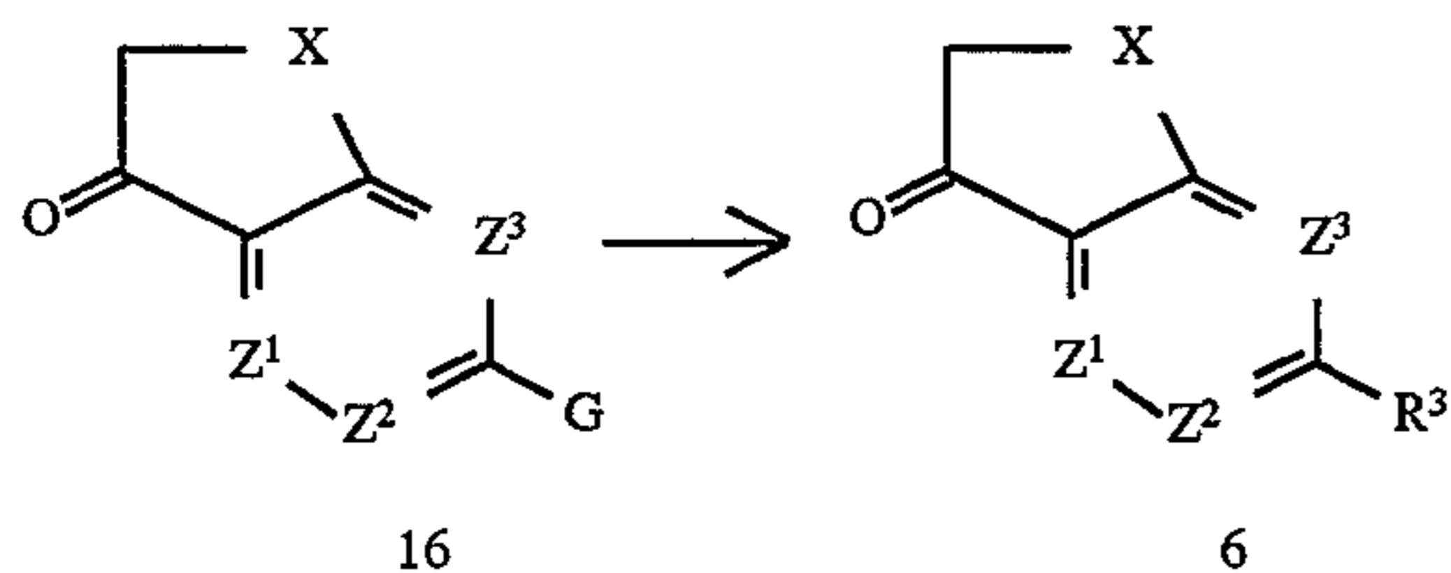
Scheme 7
