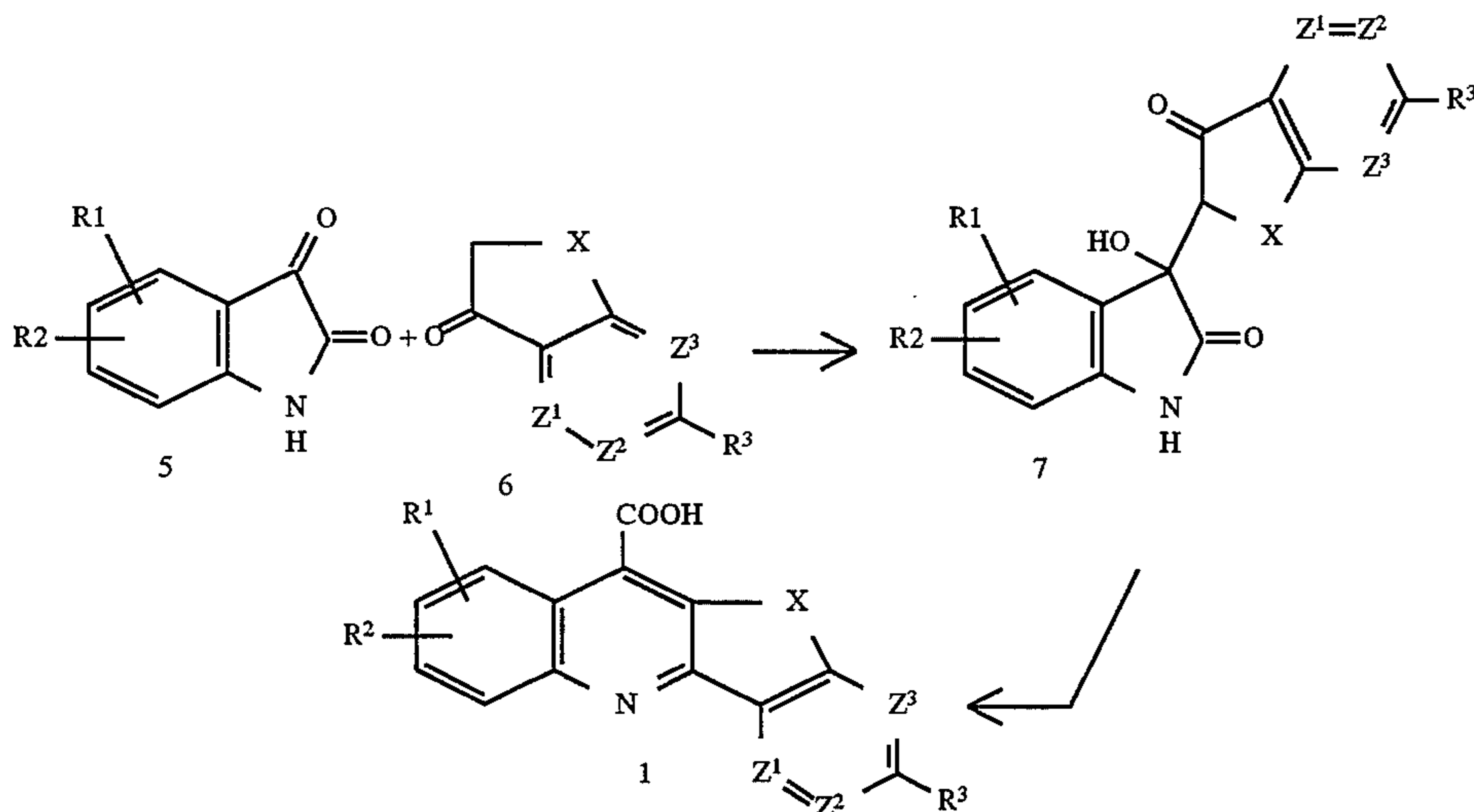
Scheme 2
