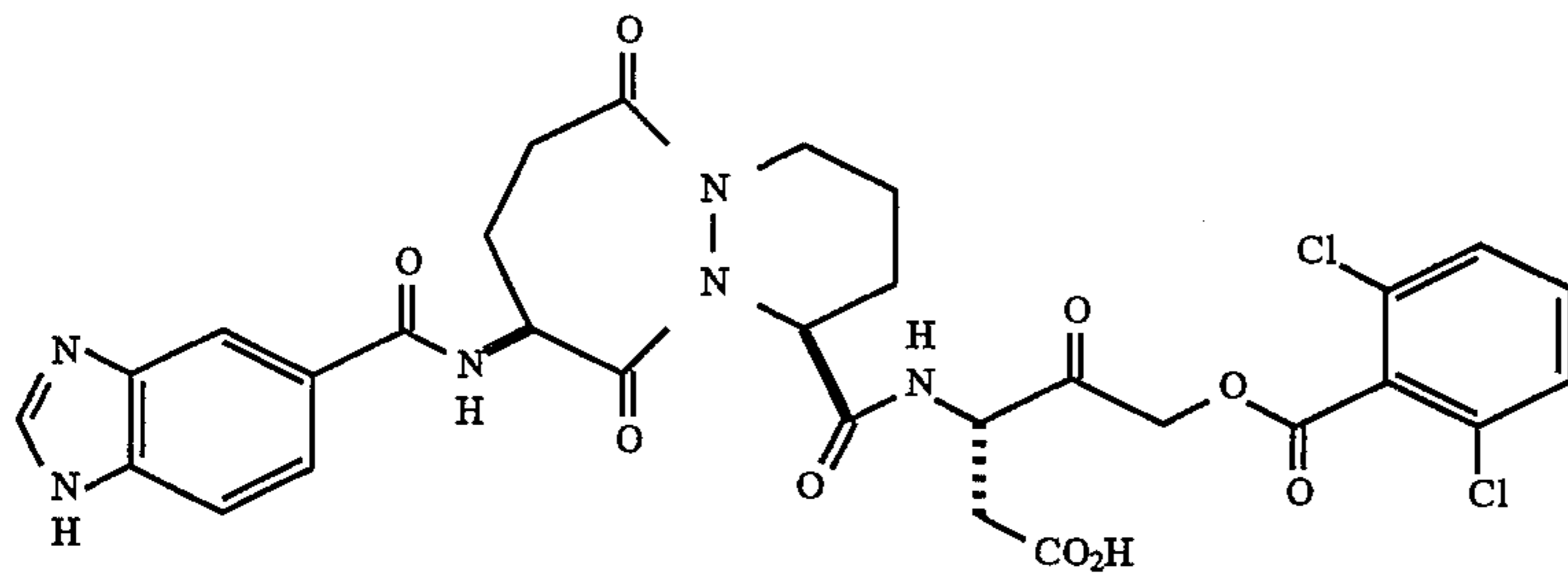
[9-(5-Benzimidazolylamino)octahydro-6,10-dioxo-6H- 15 pyridazino[1,2a][1,2]diazepine-1-formoyl]-L-aspartic acid 2,6-dichlorobenzoyloxymethyl ketone mass spectrum: m/z 687 (M+H)
