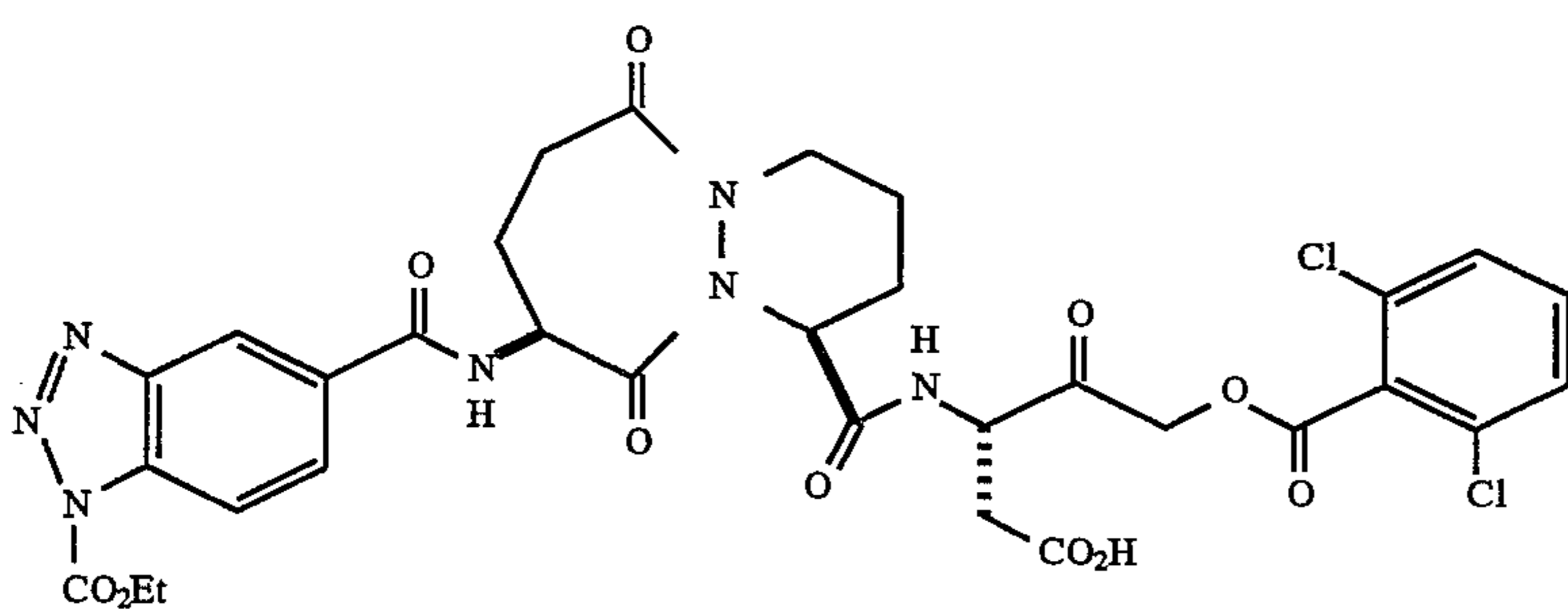
[9-(N-Carboethoxy-5-bentriazolylamino)octahydro-6,10- 55 dioxo-6H-pyridazino[1,2a][1,2]diazepine-1-formoyl]-L- aspartic acid 2,6-dichlorobenzoyloxymethyl ketone mass spectrum: m/z 760 (M+H)
