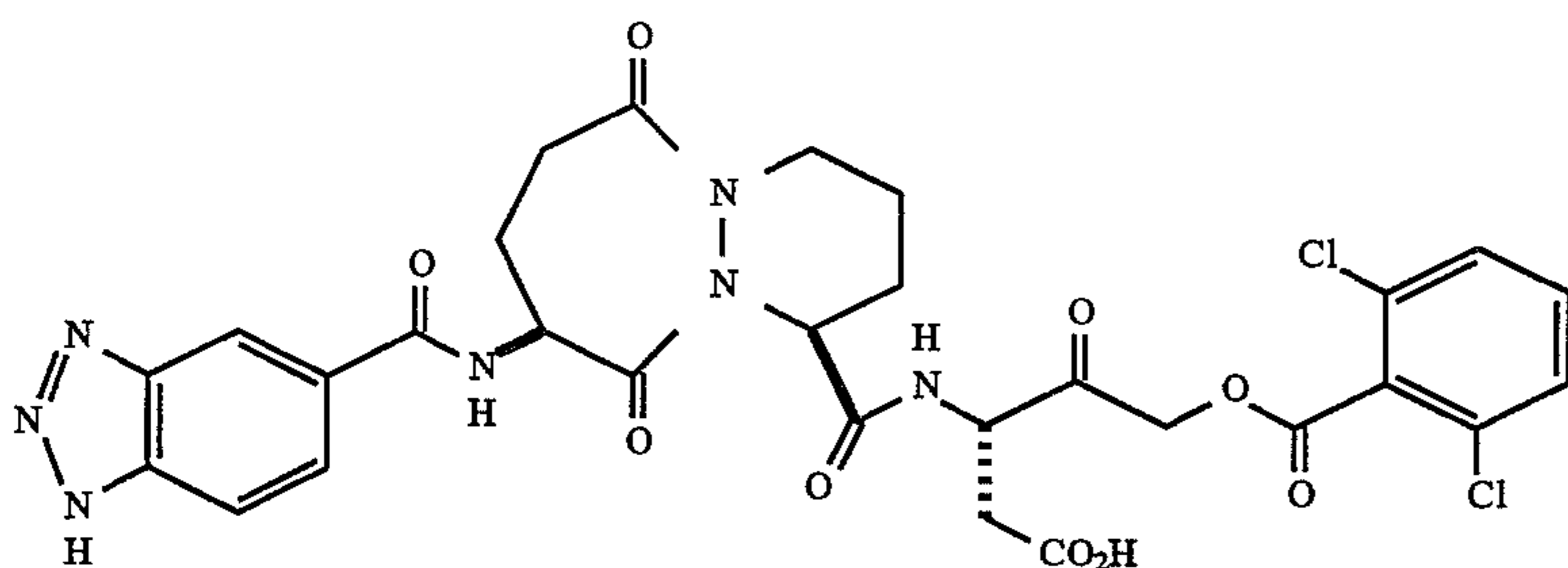
[9-(5-Bentriazolylamino)octahydro-6,10-dioxo-6H- 35 pyridazino[1,2a][1,2]diazepine-1-formoyl]-L-aspartic acid 2,6-dichlorobenzoyloxymethyl ketone mass spectrum: m/z 688 (M+H)
