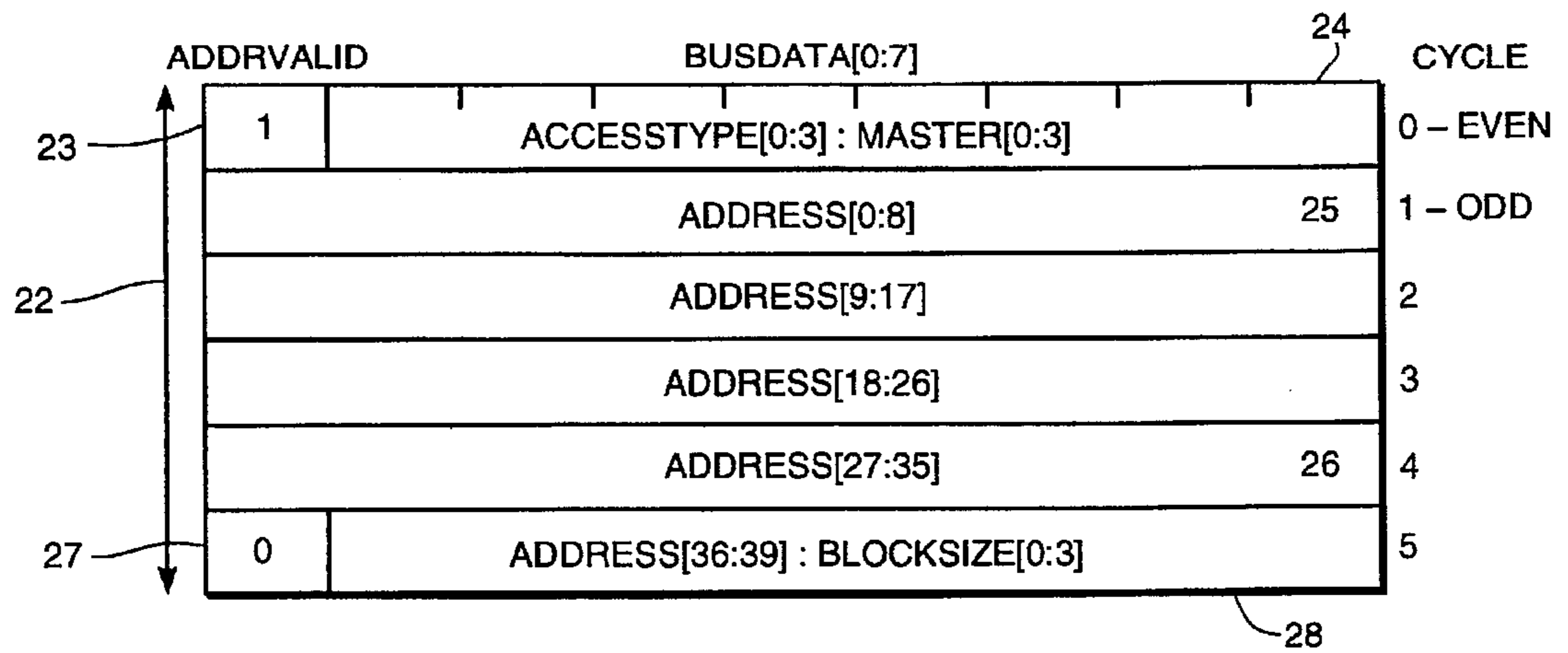
FIG 4 REGULAR ACCESS
