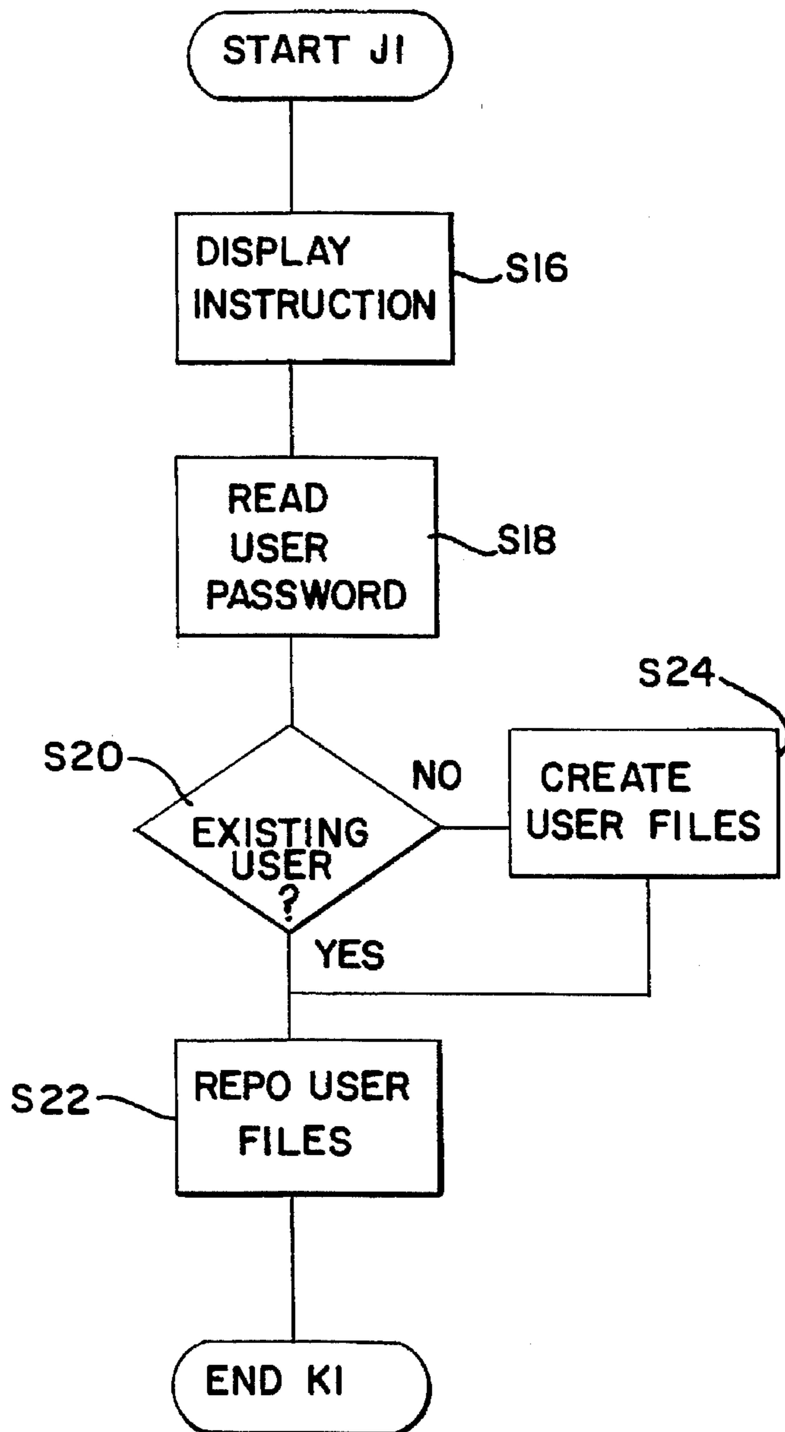
FIG. 8 USER SIGN-ON
