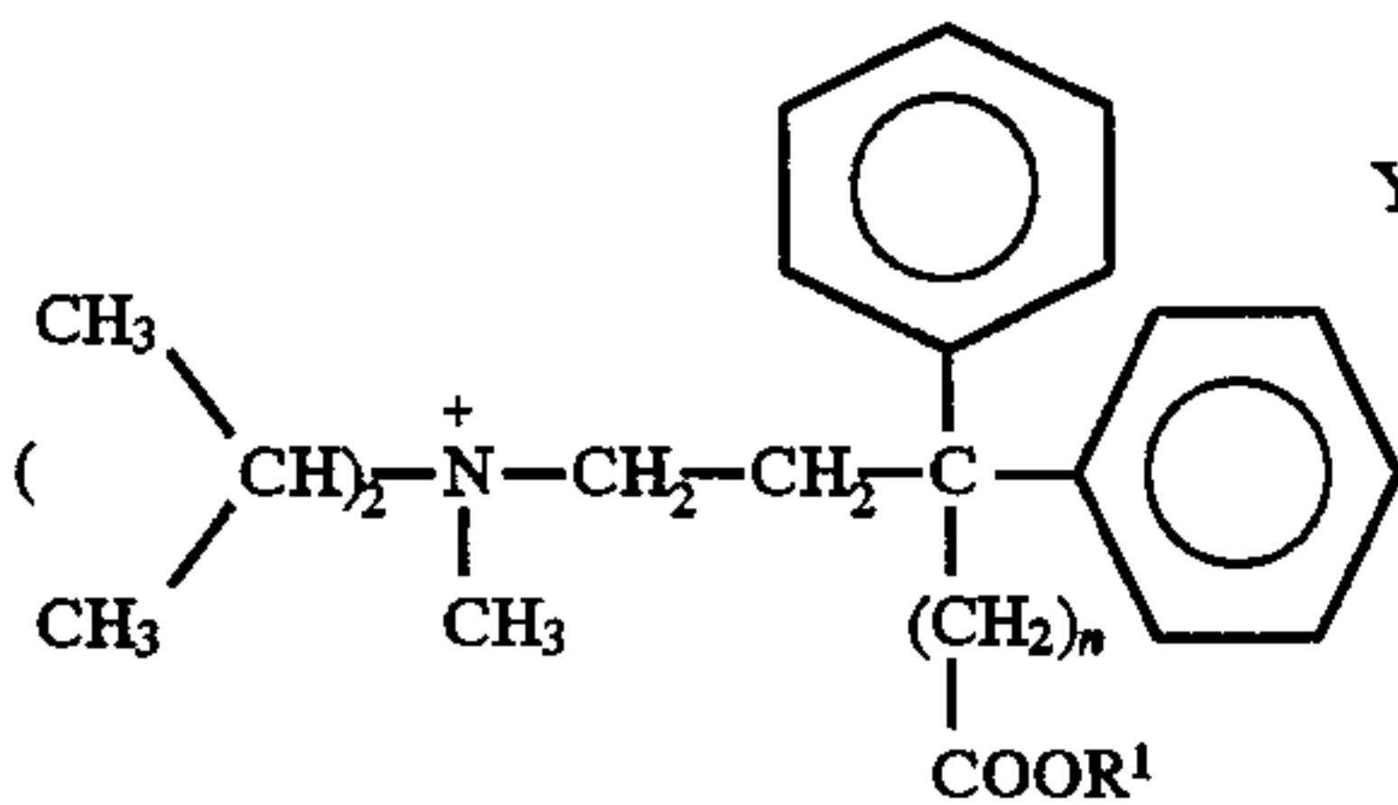
Soft Drug
