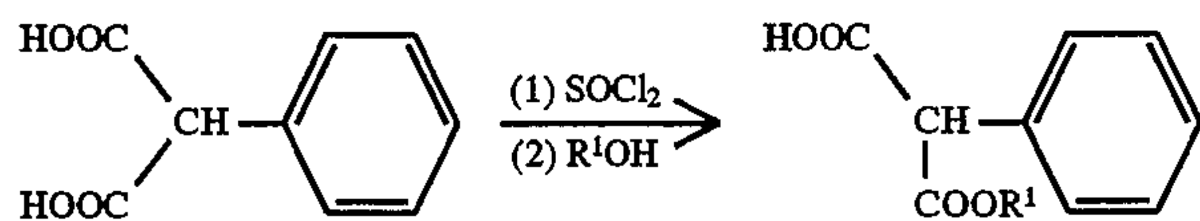
phenylmalonic acid
