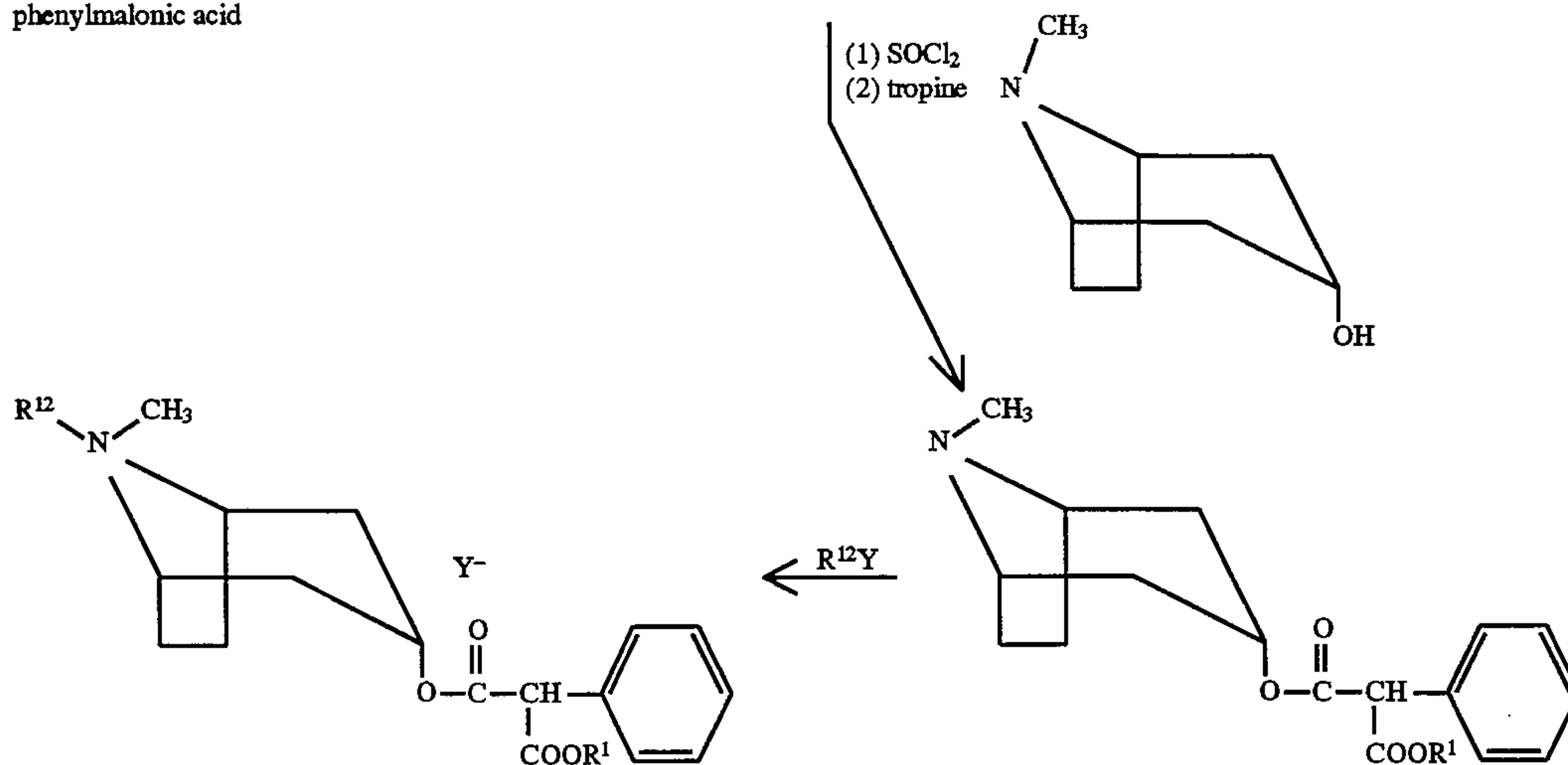
phenylmalonic acid
