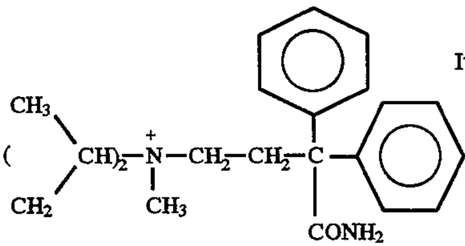
Isopropamide Iodide
