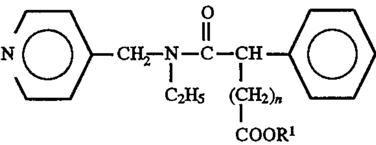
Soft Drug
