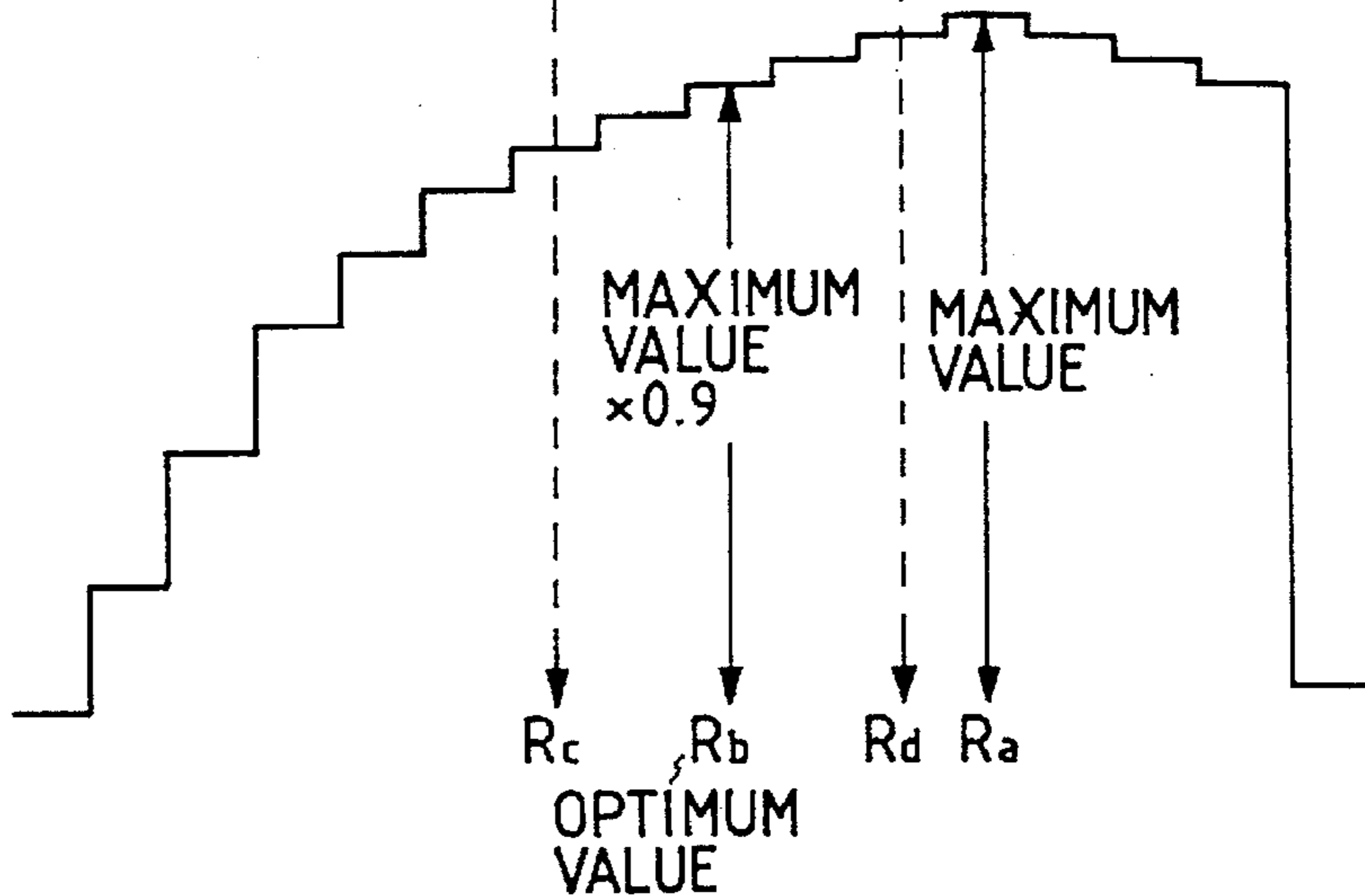
FIG. 9(D) REPRODUCED VIDEO SIGNAL EXAMPLE
