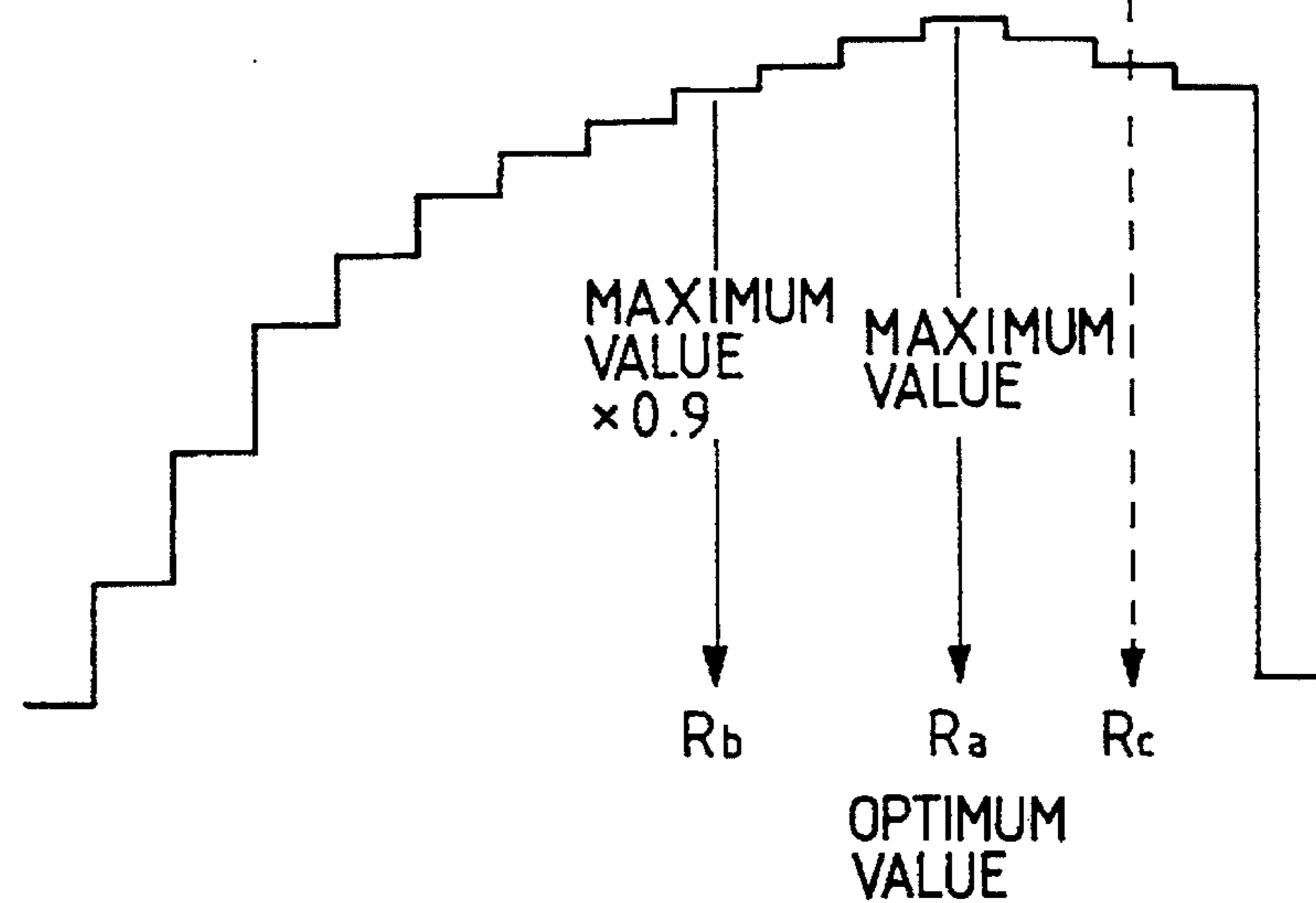
FIG. 7(D) REPRODUCED VIDEO SIGNAL EXAMPLE
