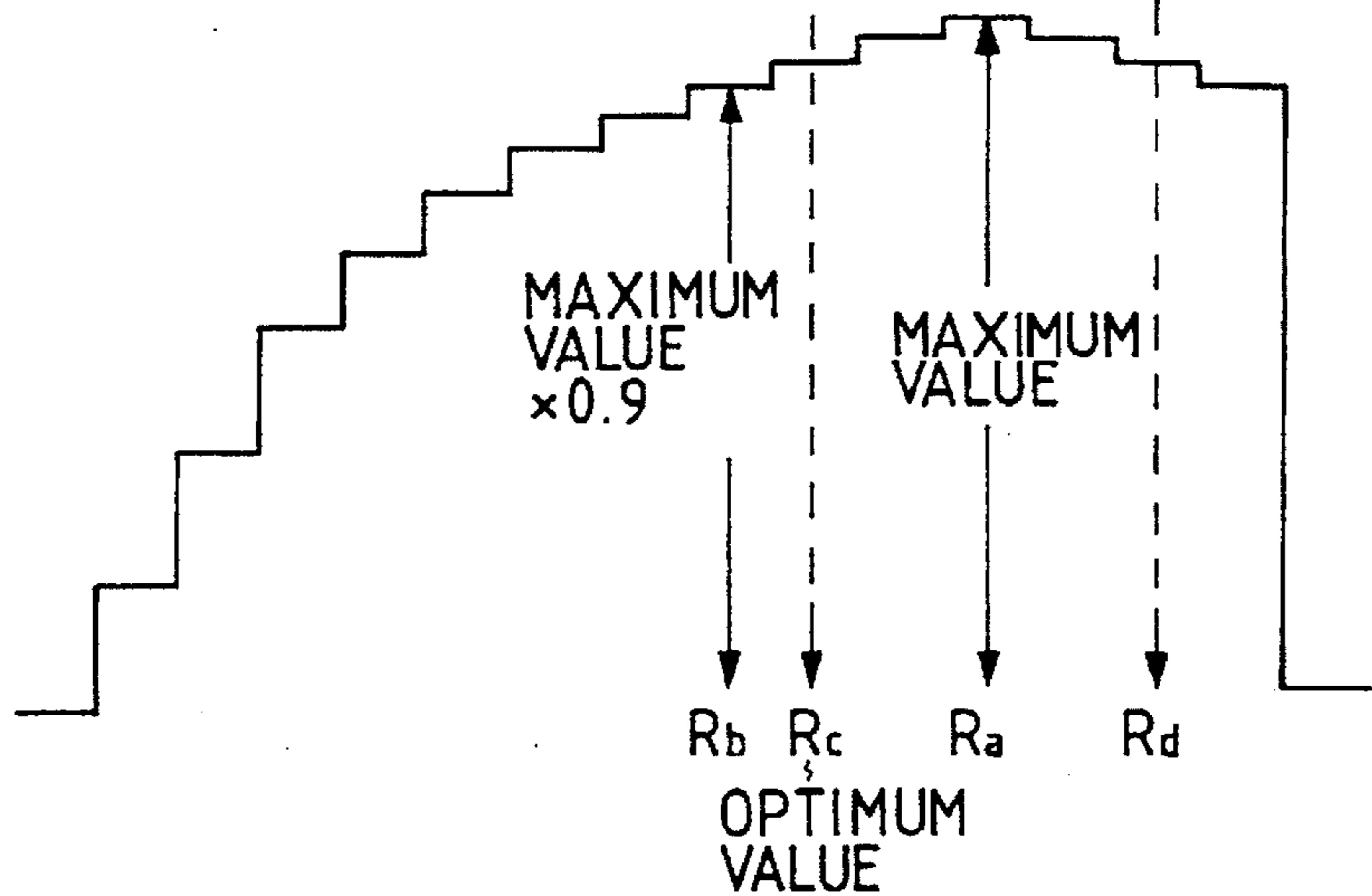
FIG. 8(D) REPRODUCED VIDEO SIGNAL EXAMPLE
