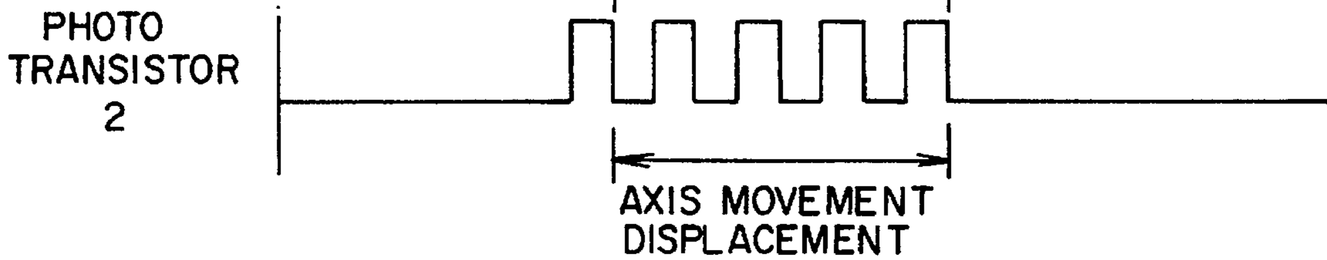
FIG. 2C PRIOR ART
