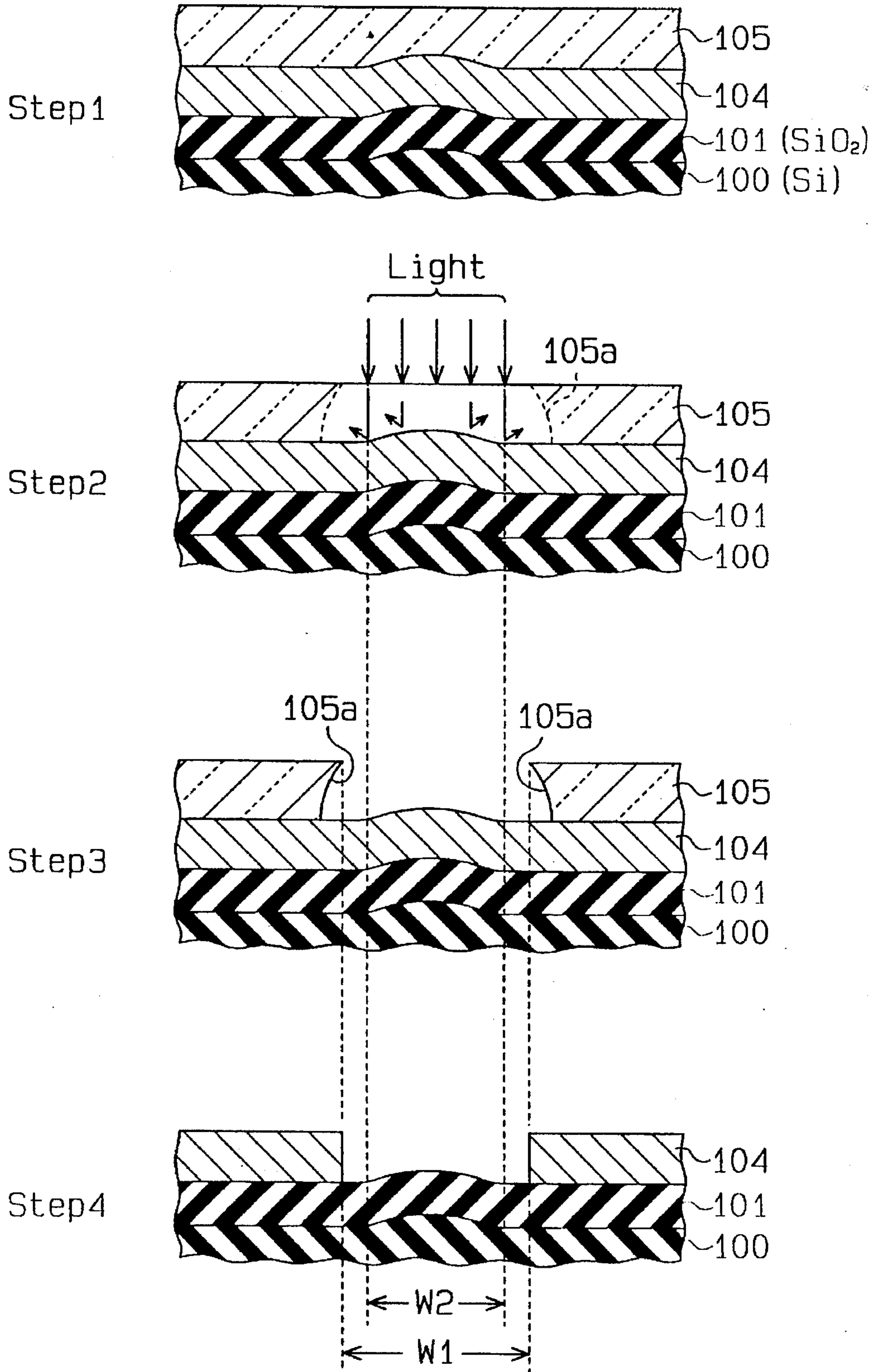
Fig. 2 (Prior Art)
