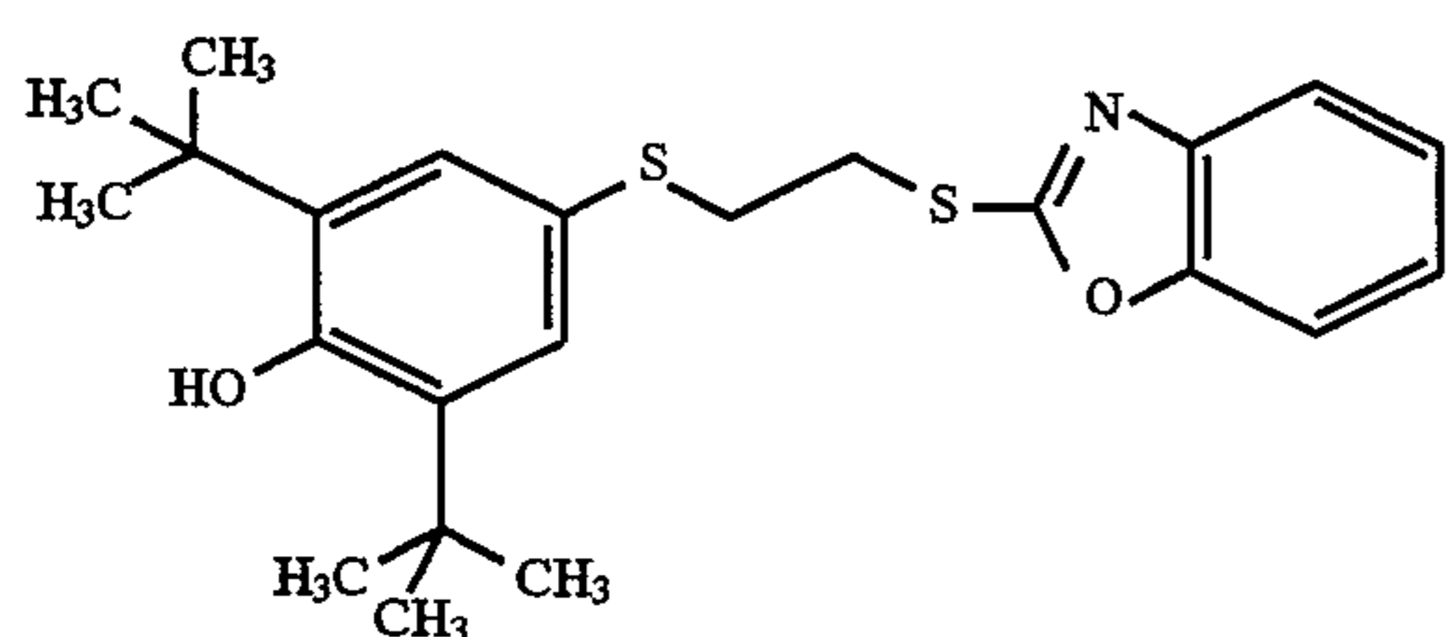
2,6-bis(1,1-dimethylethyl)-4-[[2-[(1,3-benzoxazol-2-yl)thio]ethyl]thio]phenol Hydrate (26)
