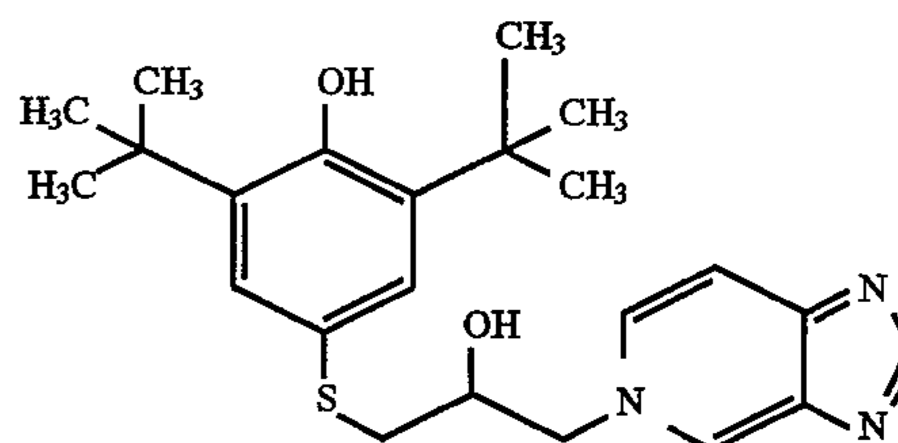
(\pm) 2,6-bis(1,1-dimethylethyl)-4-[[2-hydroxy-3-(5H-imidazo[4,5-c]pyridin-5-yl)propylthio]phenol Hydrate (27)
