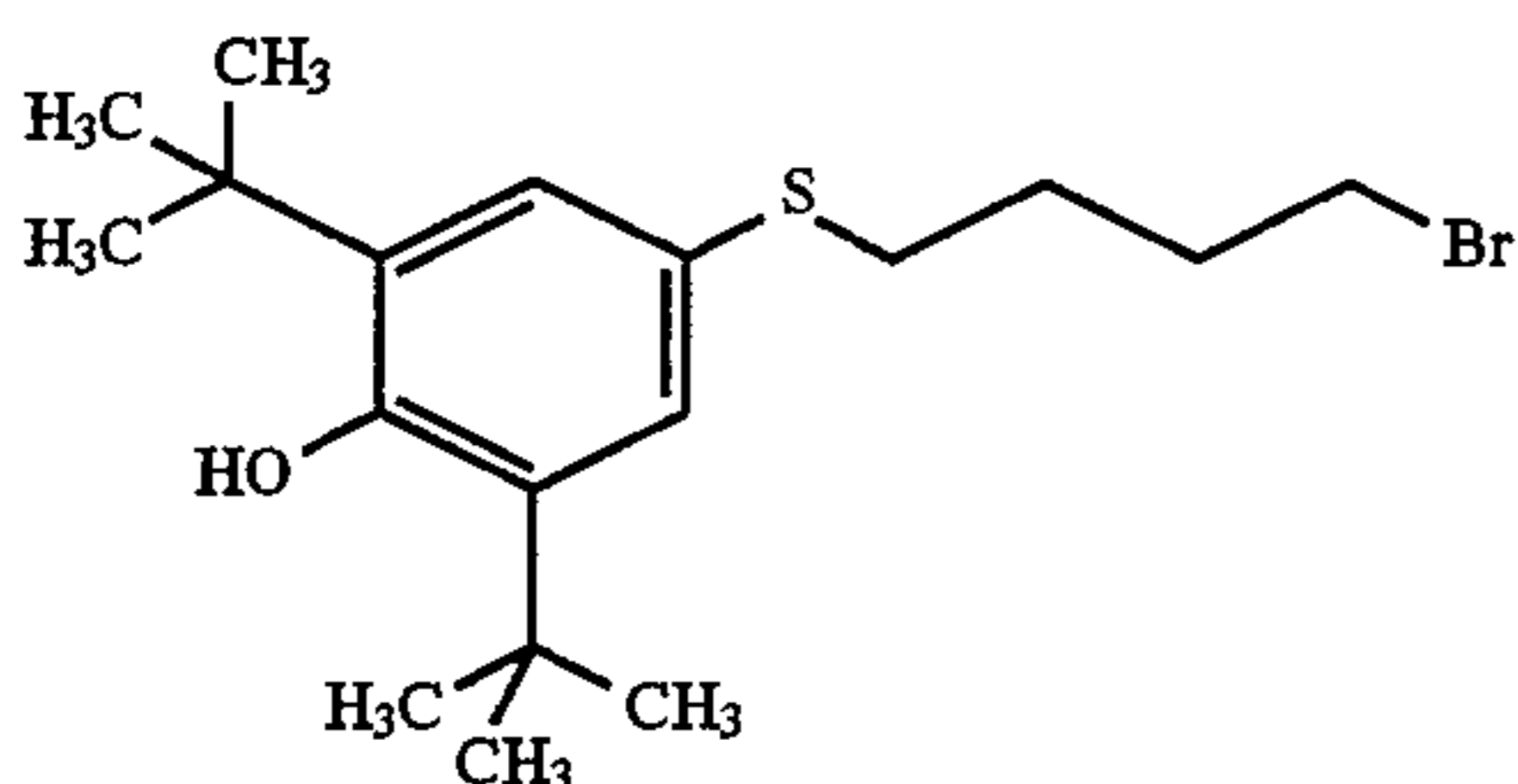
4-[(4-bromobutyl)thio]-2,6-bis(1,1-dimethylethyl)phenol (13)
