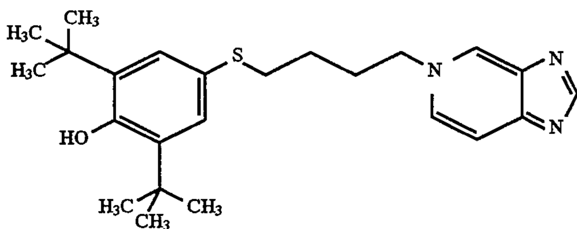
2,6-bis(1,1-dimethylethyl)-4-[[4-(5H-imidazo[4,5-c]pyridin-5-yl)butyl]thiophenol Hydrate (14)
