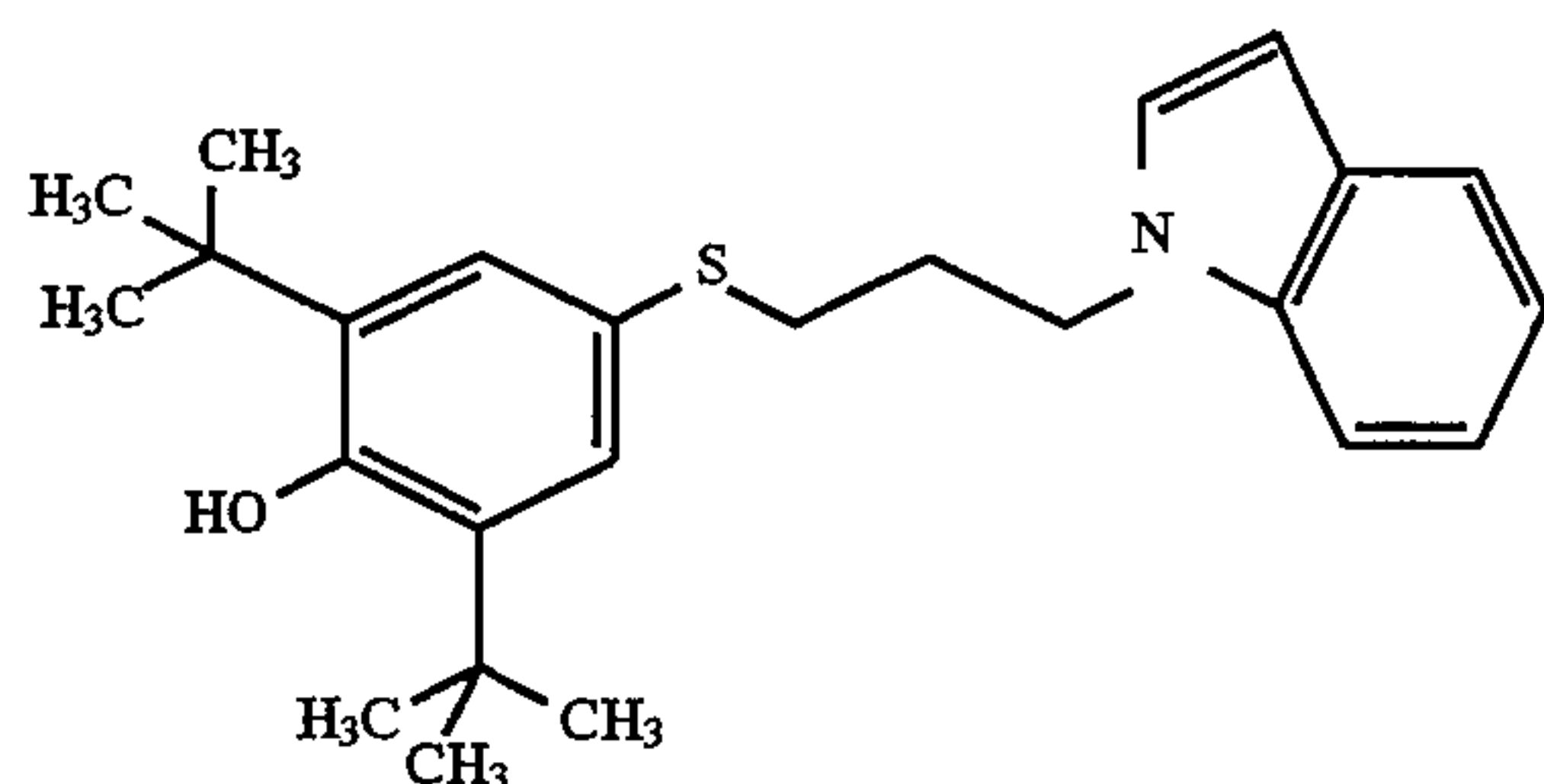
2,6-bis(1,1-dimethylethyl)-4-[[3-(1H-indol-1-yl)propyl]thio]phenol Hydrate (24)
