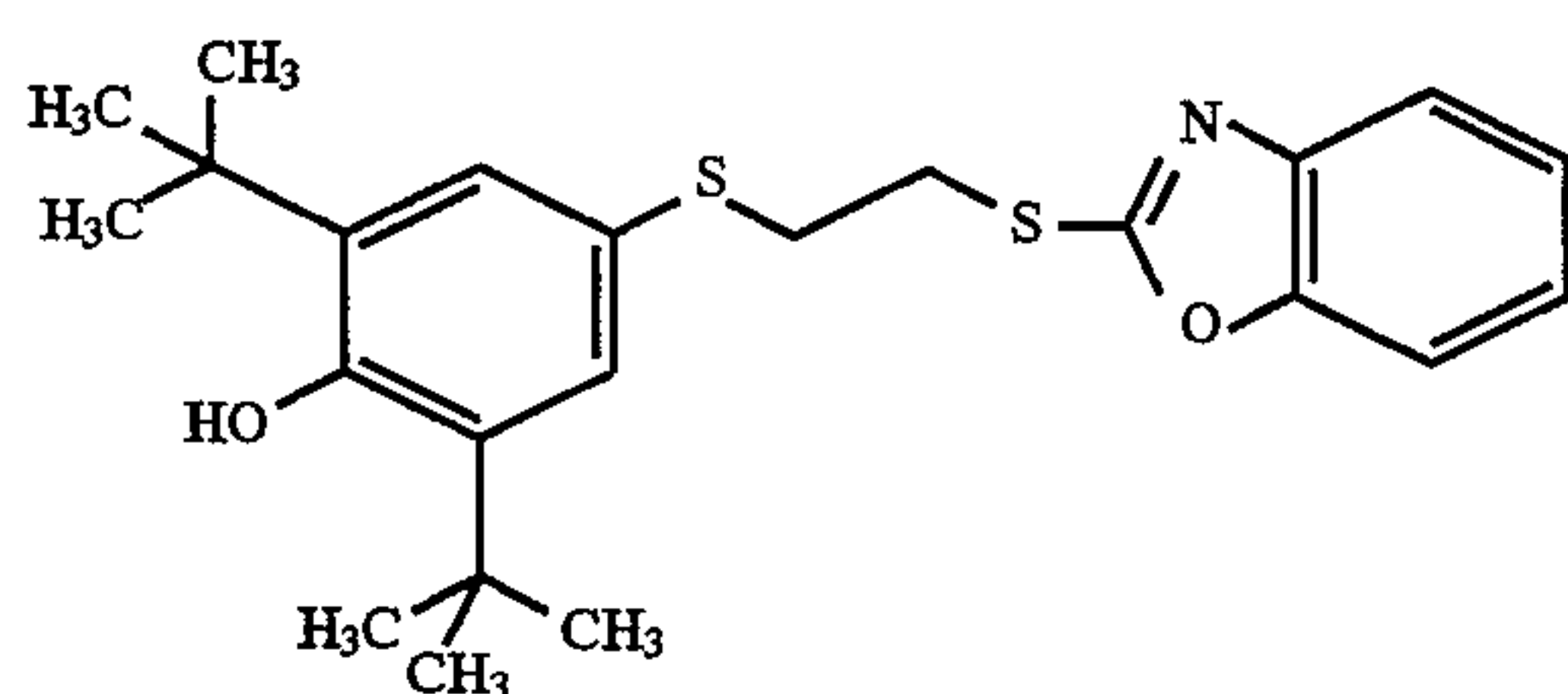
2,6-bis(1,1-dimethylethyl)-4-[[2-[(1,3-benzoxazol-2-yl)thio]ethyl]thio]phenol Hydrate (26)
