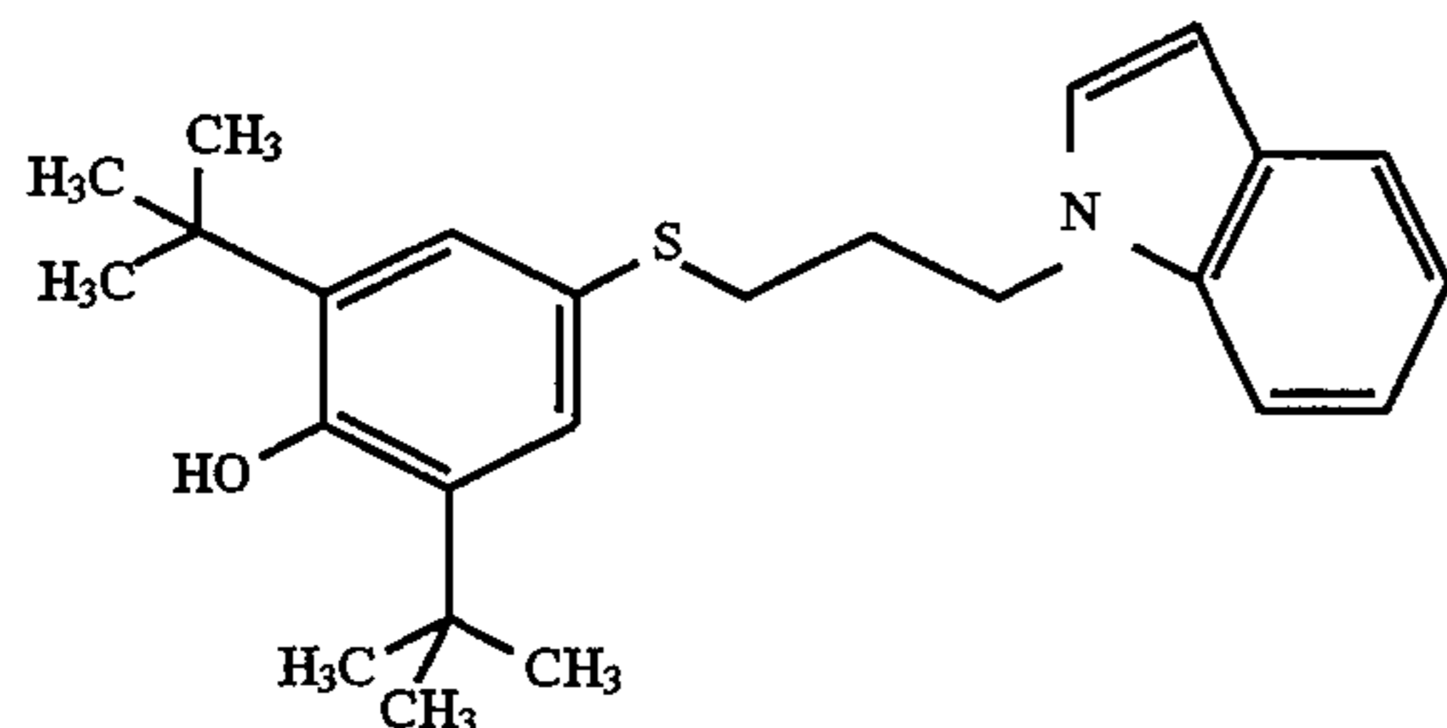
2,6-bis(1,1-dimethylethyl)-4-[[3-(1H-indol-1-yl)propyl]thio]phenol Hydrate (24)
