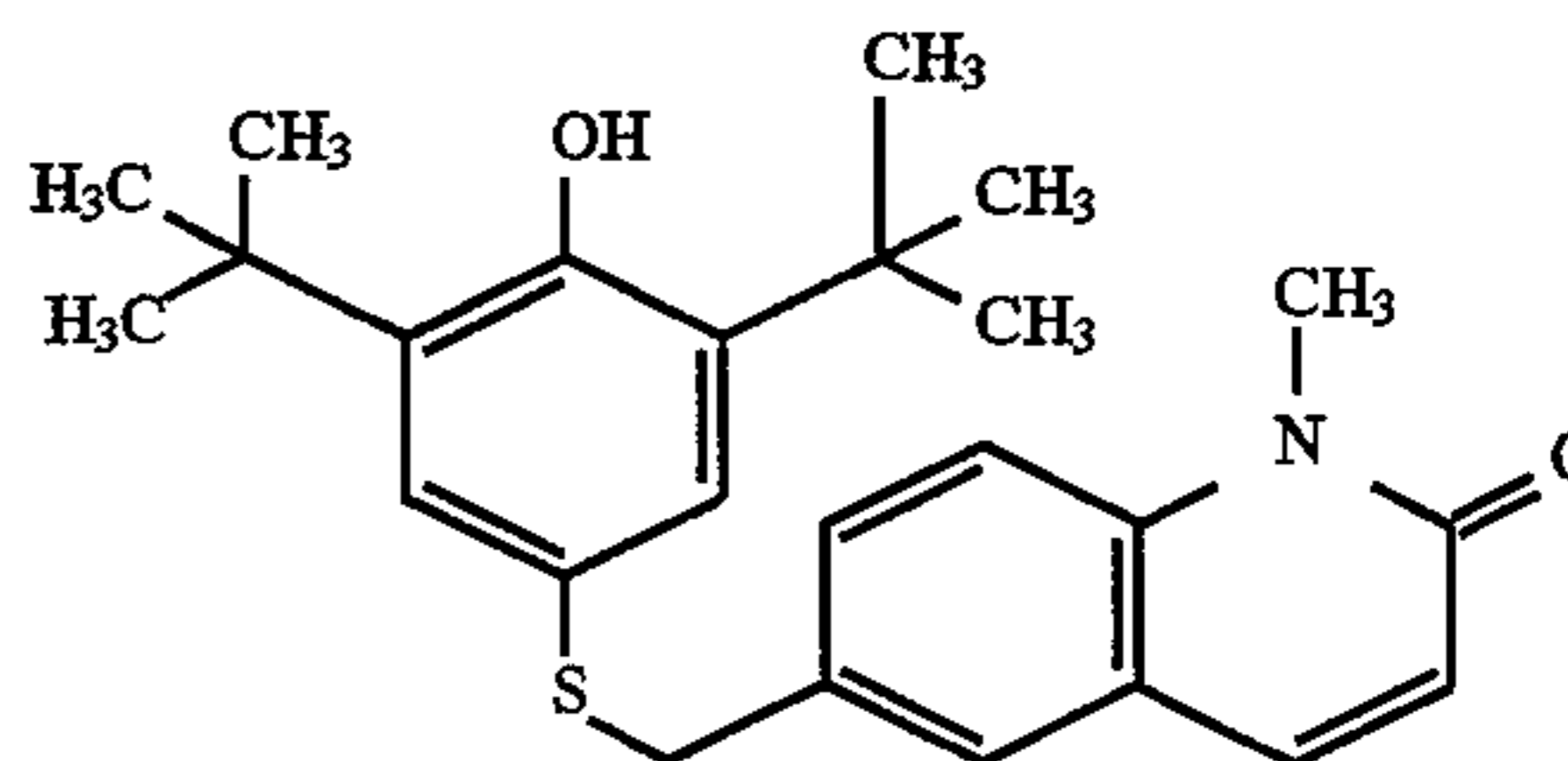
6-[[1,3-bis(dimethylethyl)-4-hydroxy phenyl]thiomethyl]-1-methyl-1H-quinolin-2-one (28)
