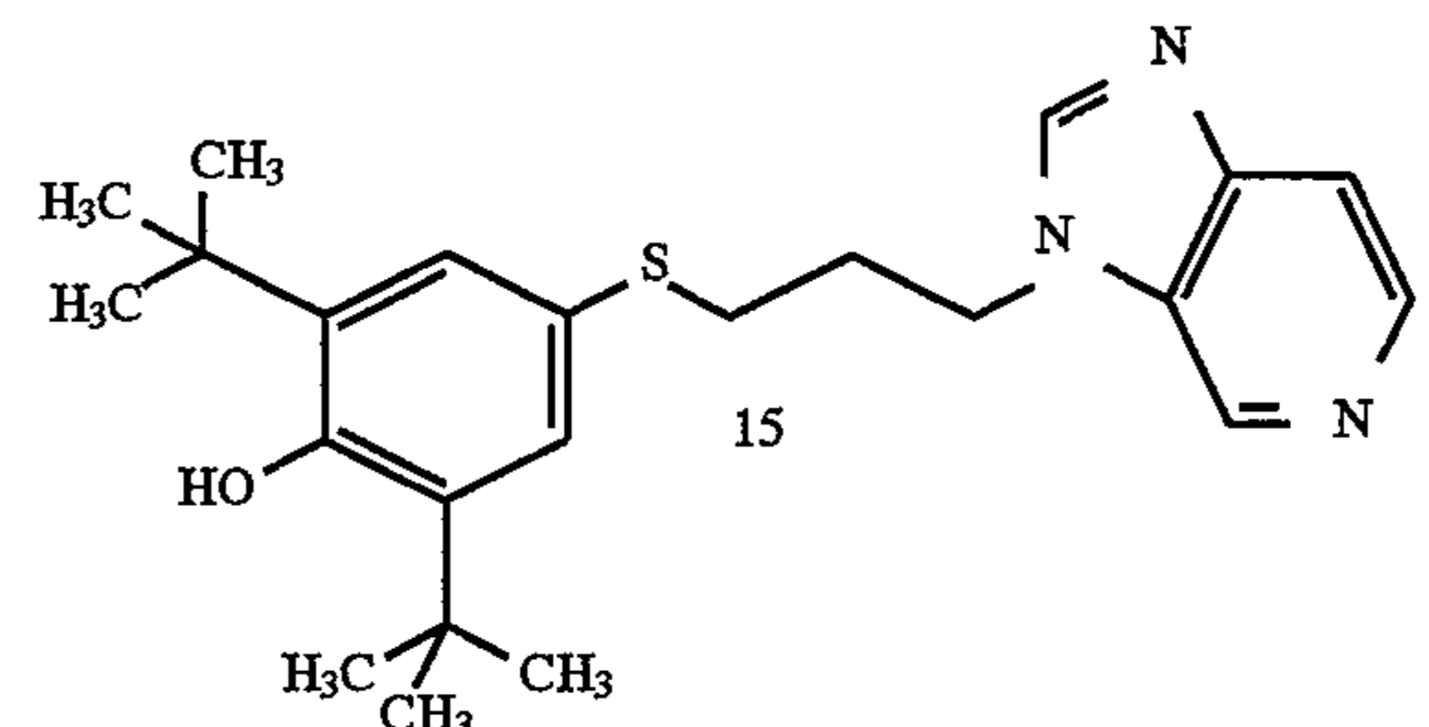
2,6-bis(1,1-dimethylethyl)-4-[[3-(5H-imidazo[4,5-c]pyridin-5-yl)propyl]thio]phenol (5)
