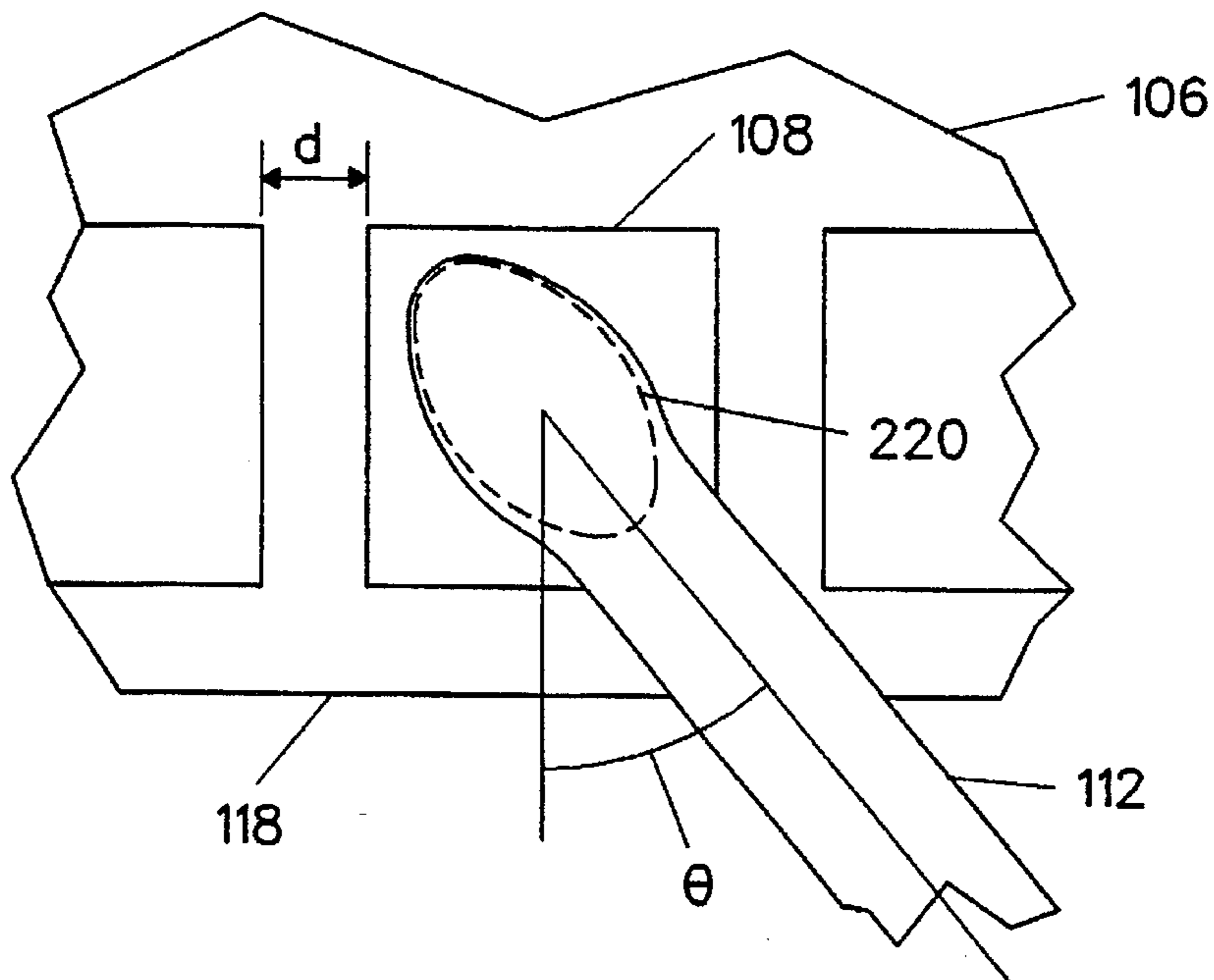
FIG. 2 (PRIOR ART)
