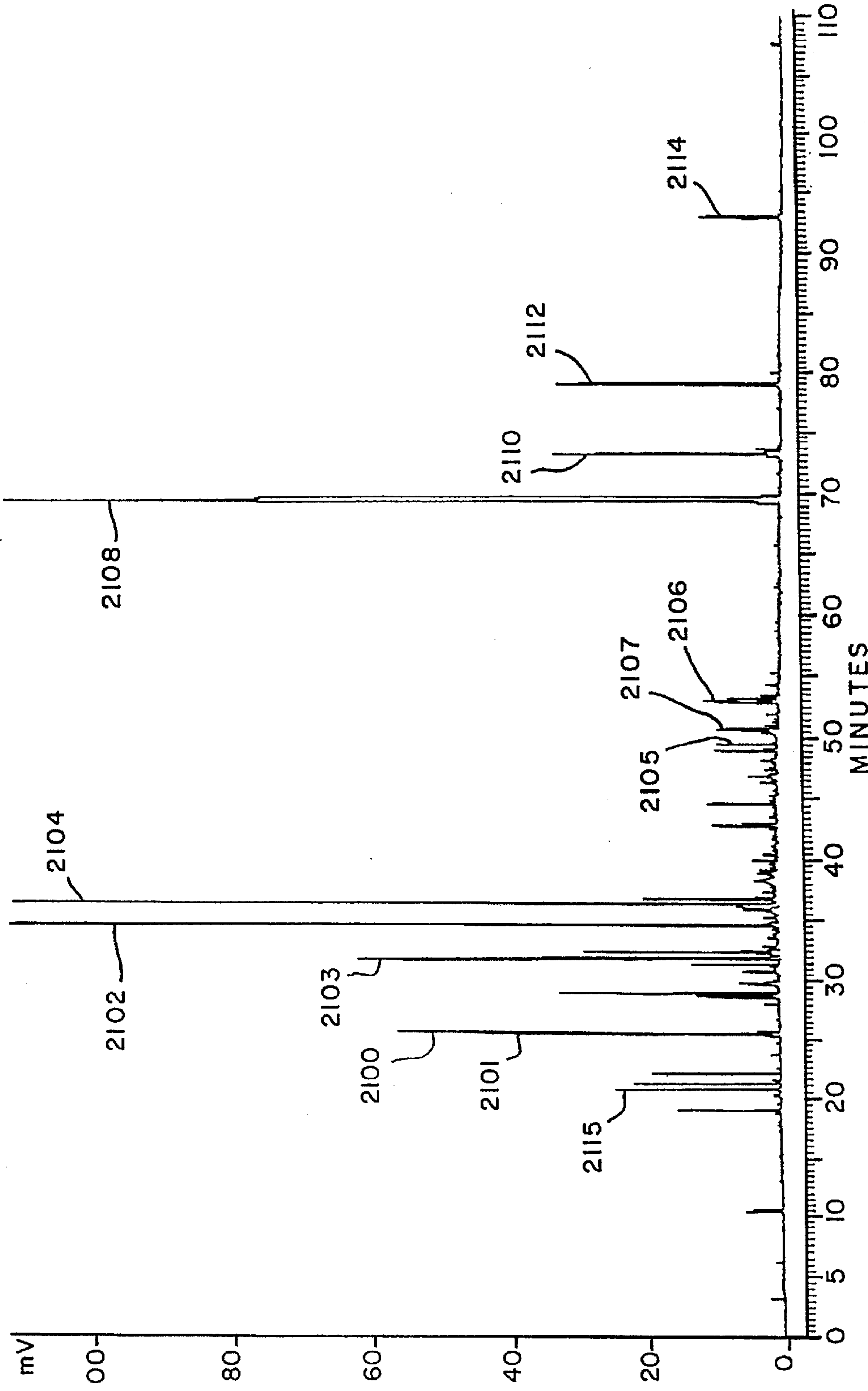
FIG.22 GC-MASS SPECTRUM
