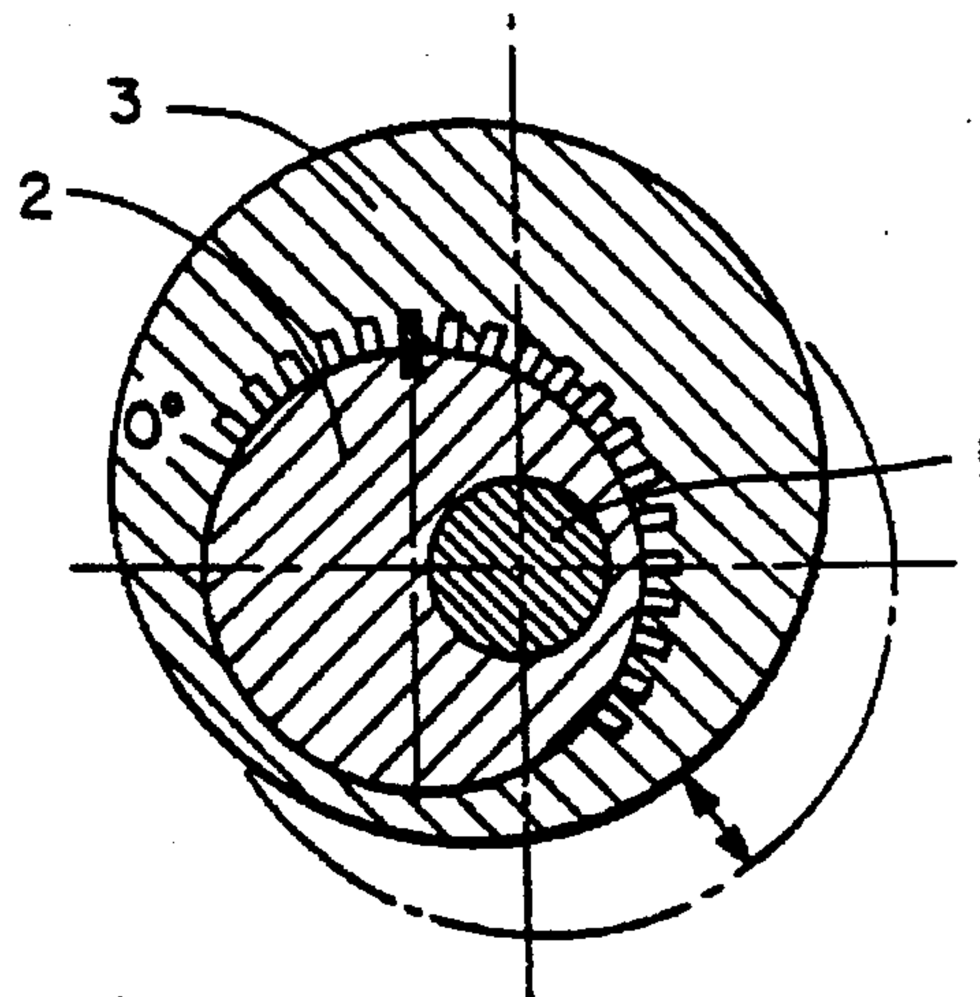
Fig. 29 INTERMEDIATE FIXED POSITION (WITH SPLINE KEY)
