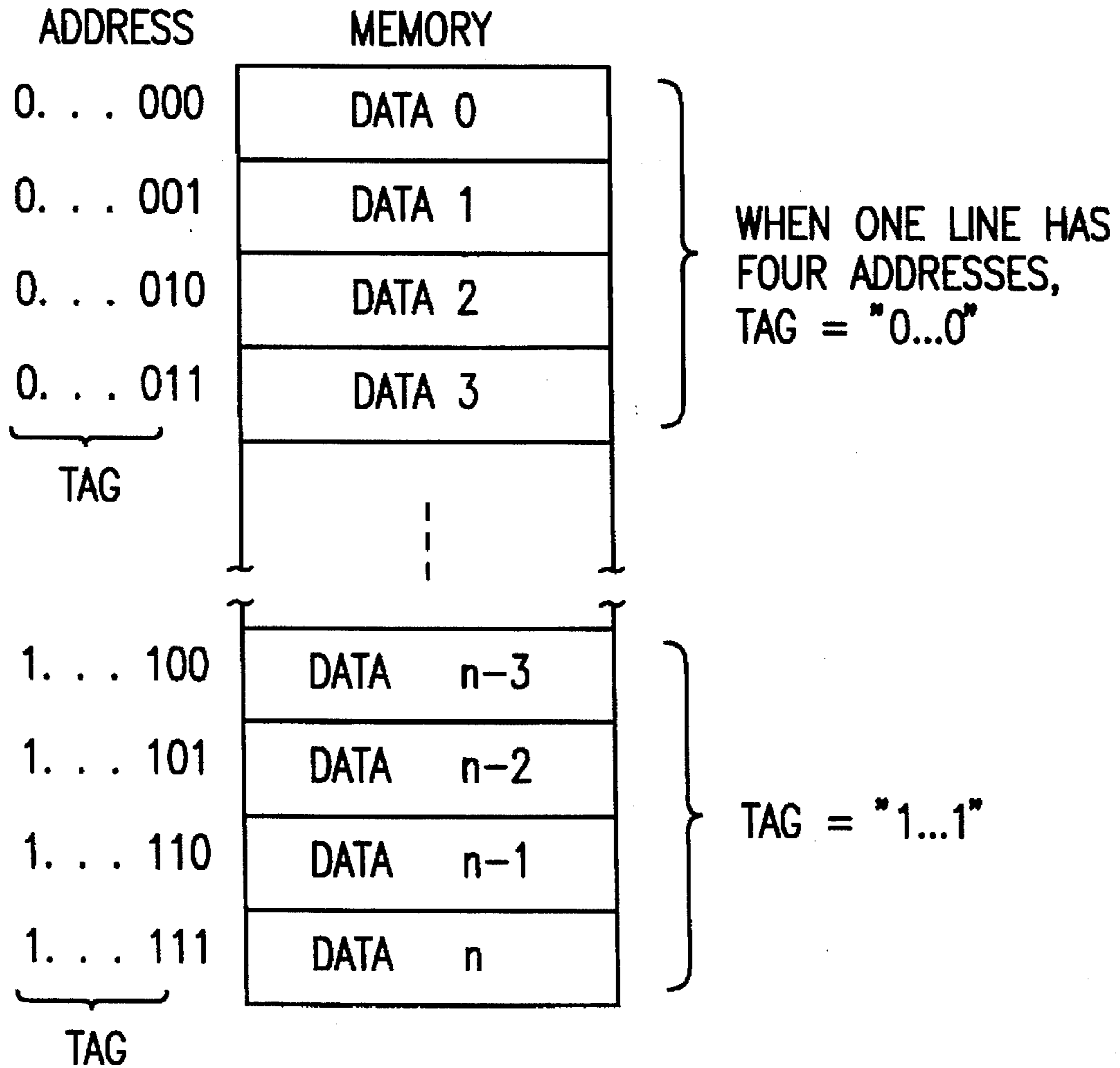
FIG. 3 PRIOR ART
