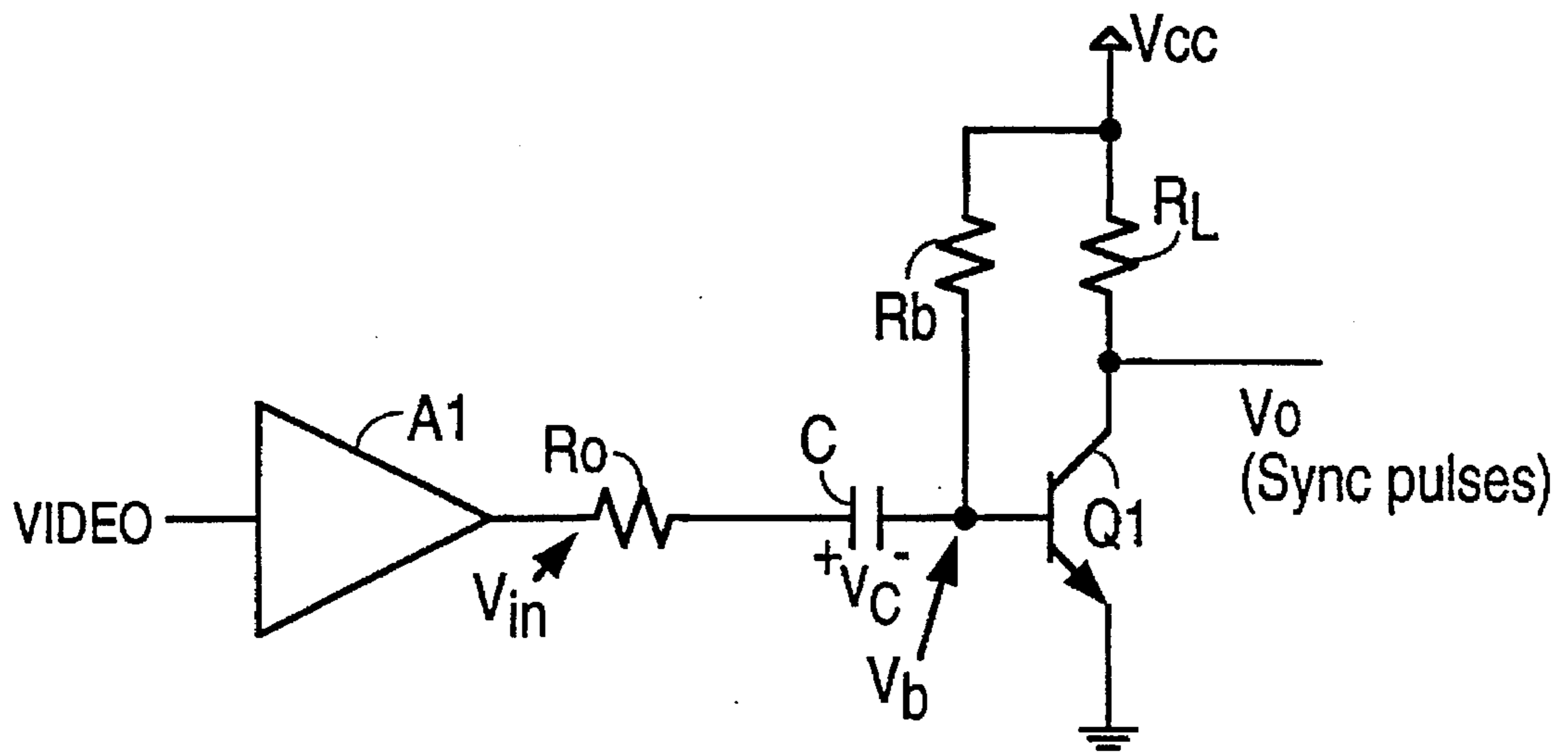
FIG. 10 (PRIOR ART)
