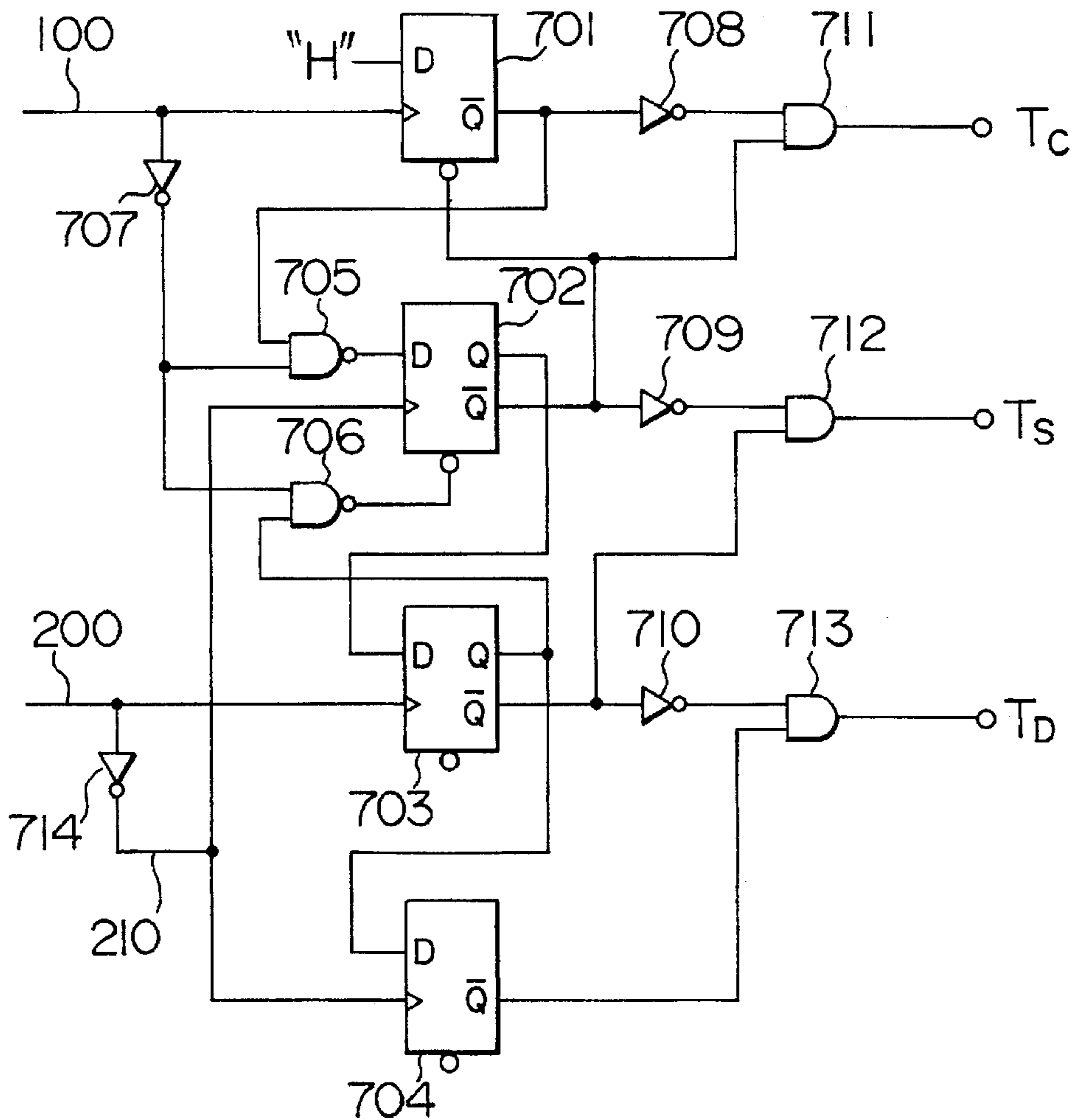
FIG. 23 PRIOR ART
