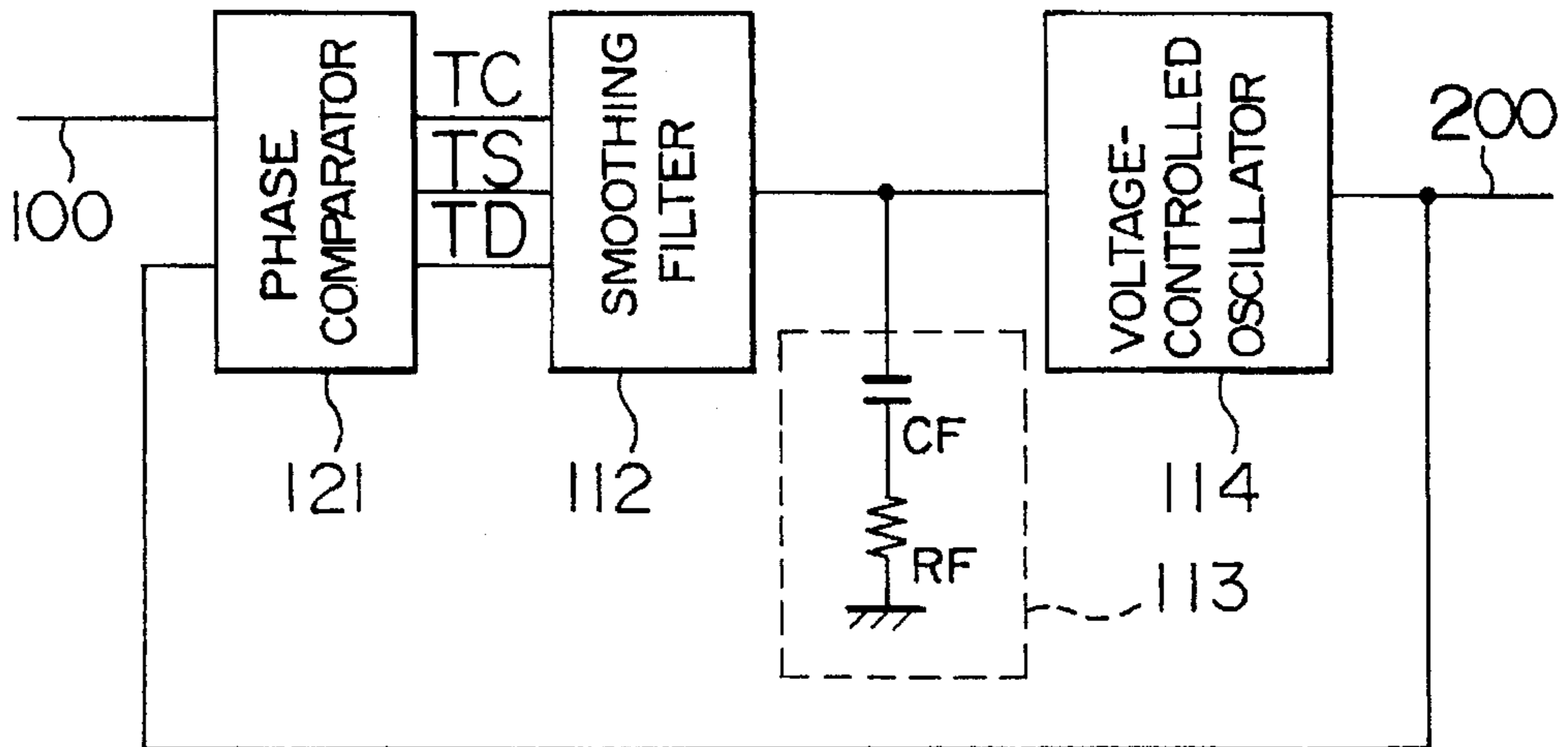
FIG. 22 PRIOR ART
