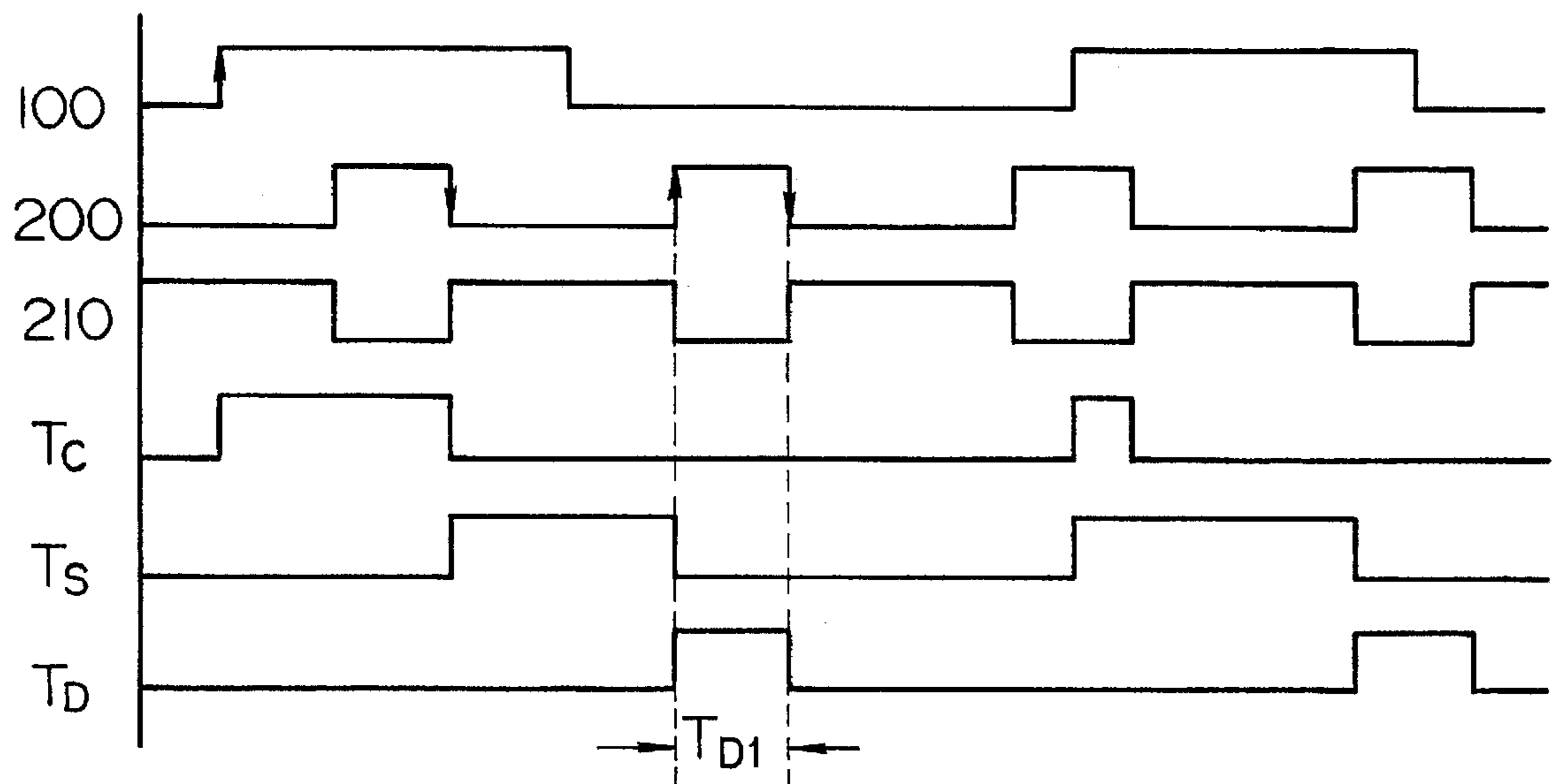
FIG. 24 PRIOR ART
