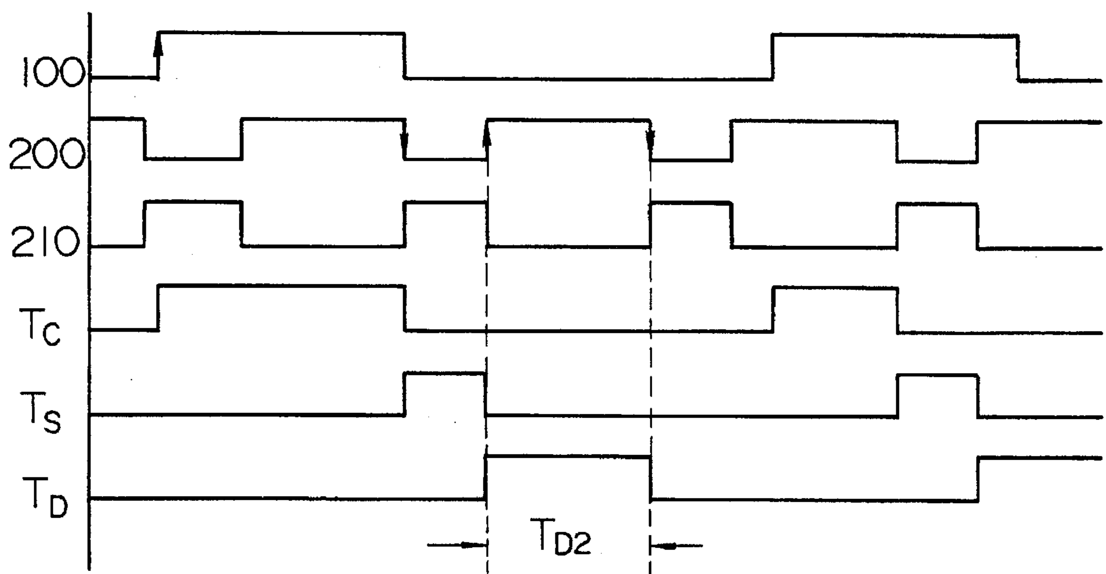
FIG. 25 PRIOR ART
