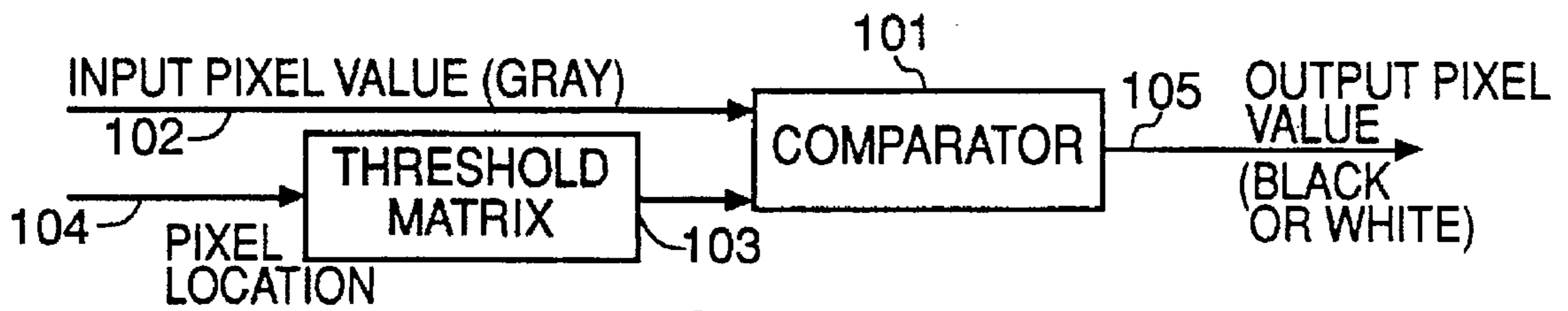
FIG. 1 (PRIOR ART)
