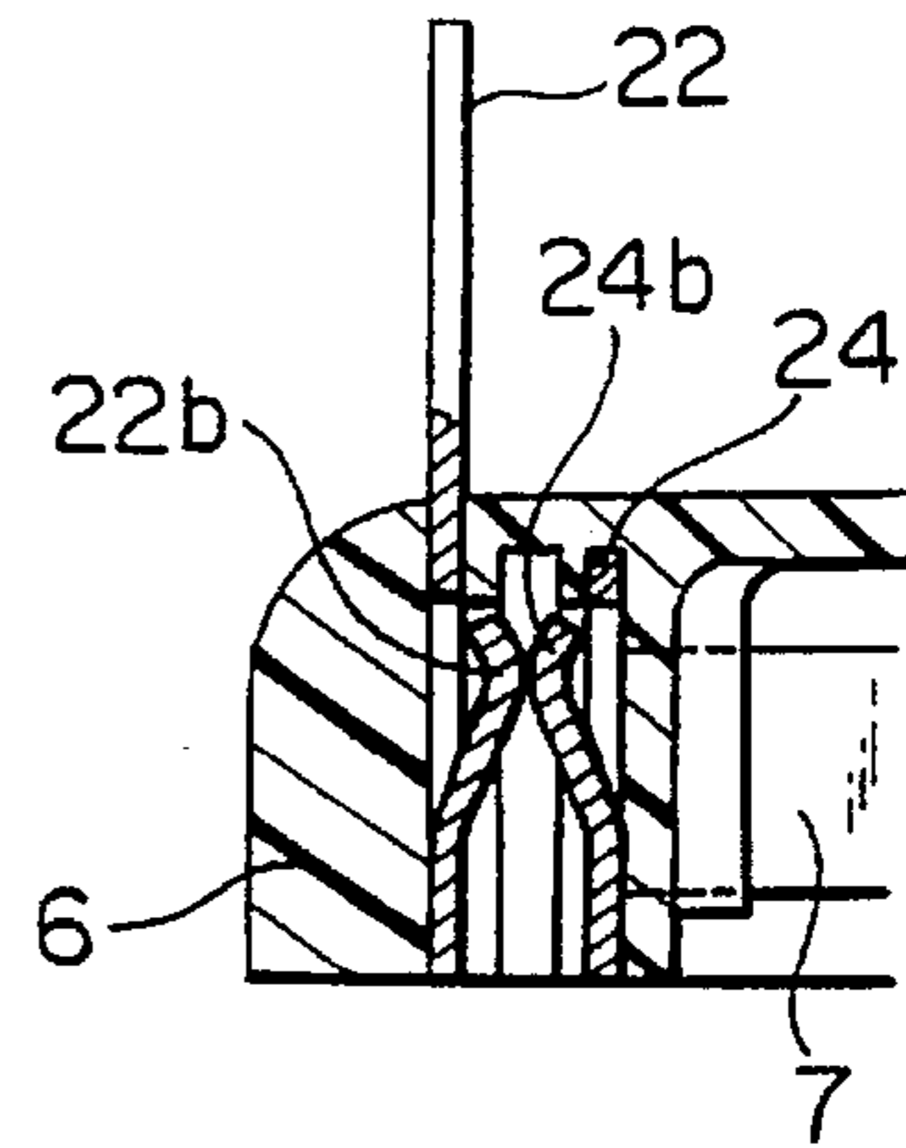
FIG. 4 (PRIOR ART)
