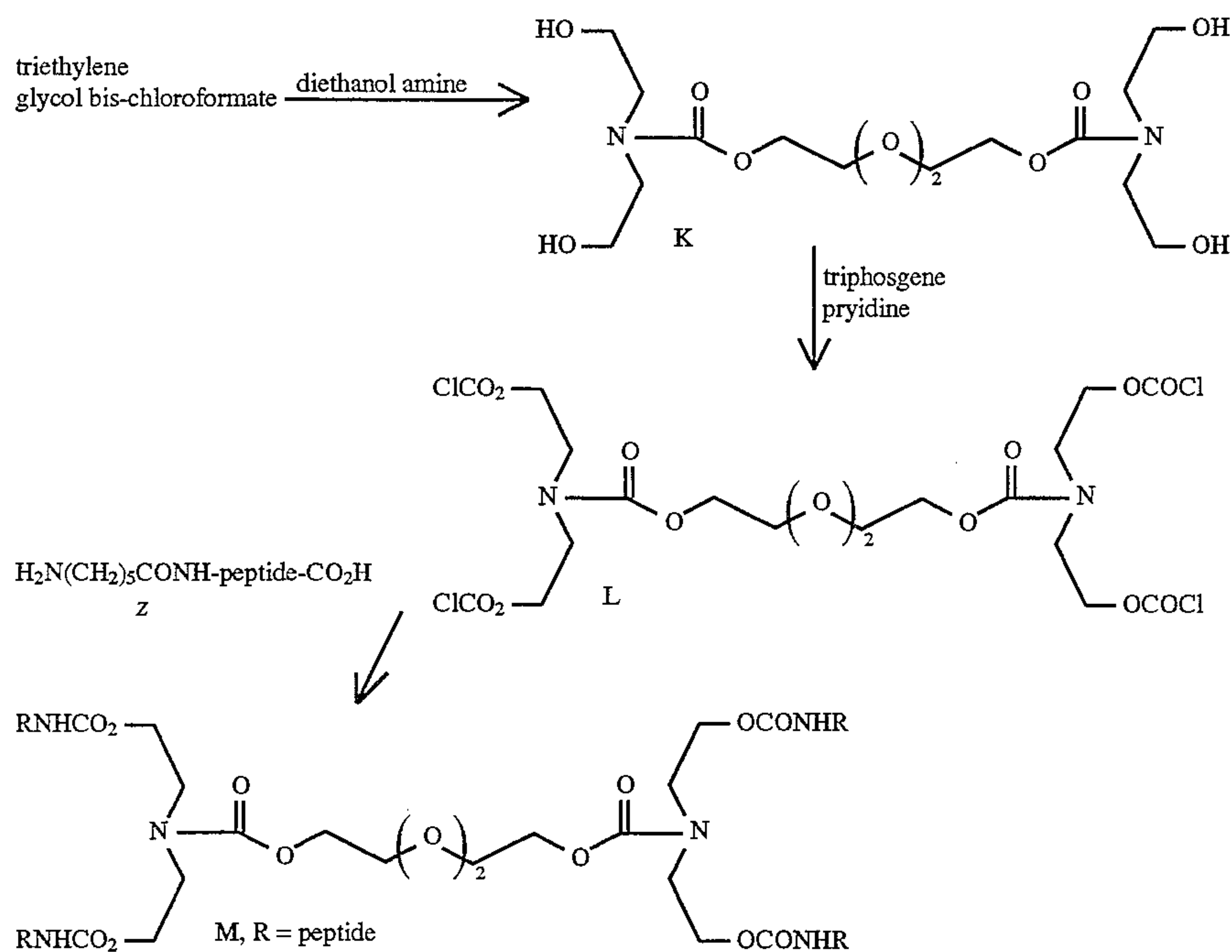
Combination 6: Chloroformate on Platform - Amine on Ligand Reaction Scheme 19
