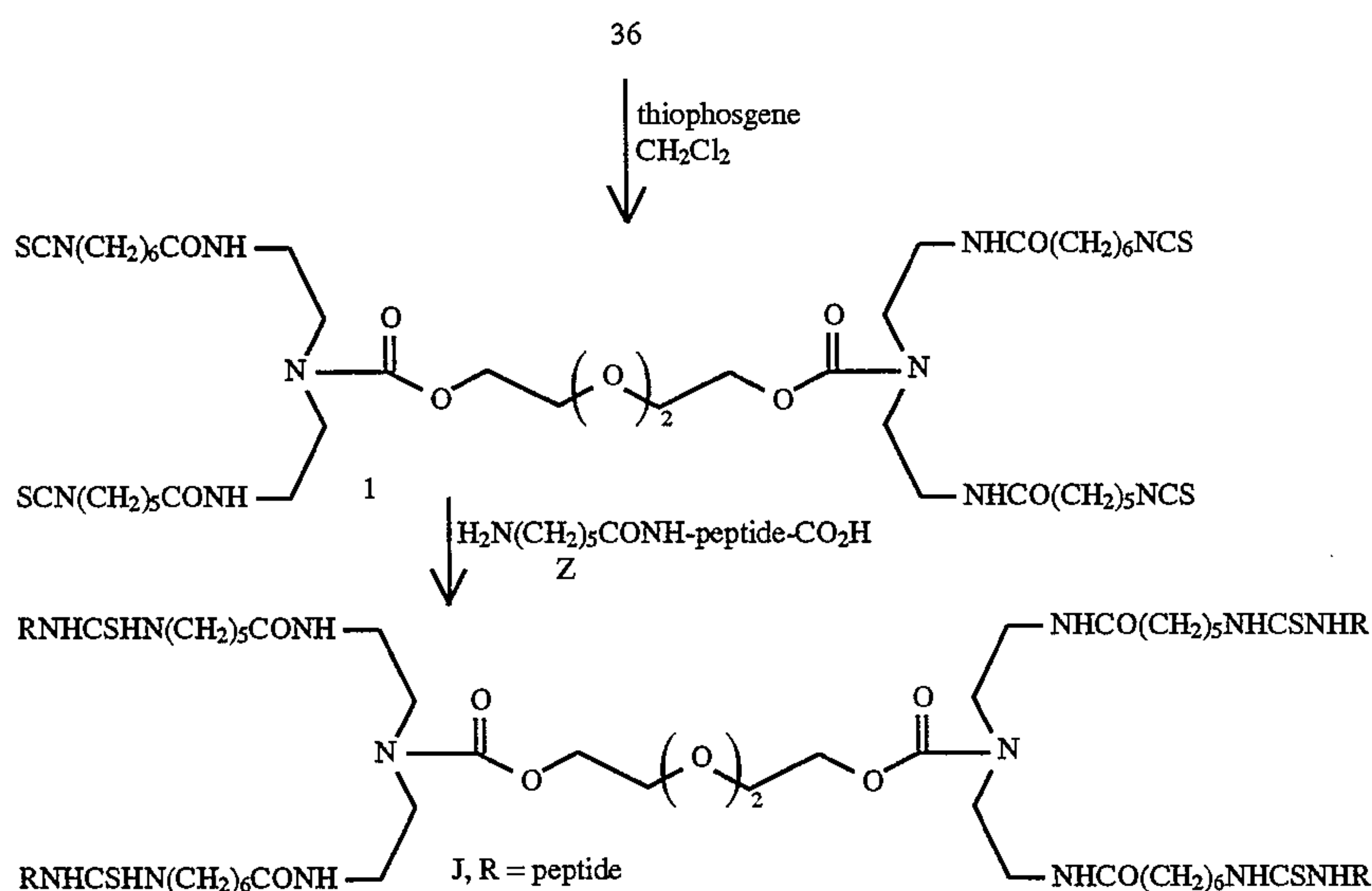
Combination 5: Isothiocyanate on Platform - Amine on Ligand Reaction Scheme 18
