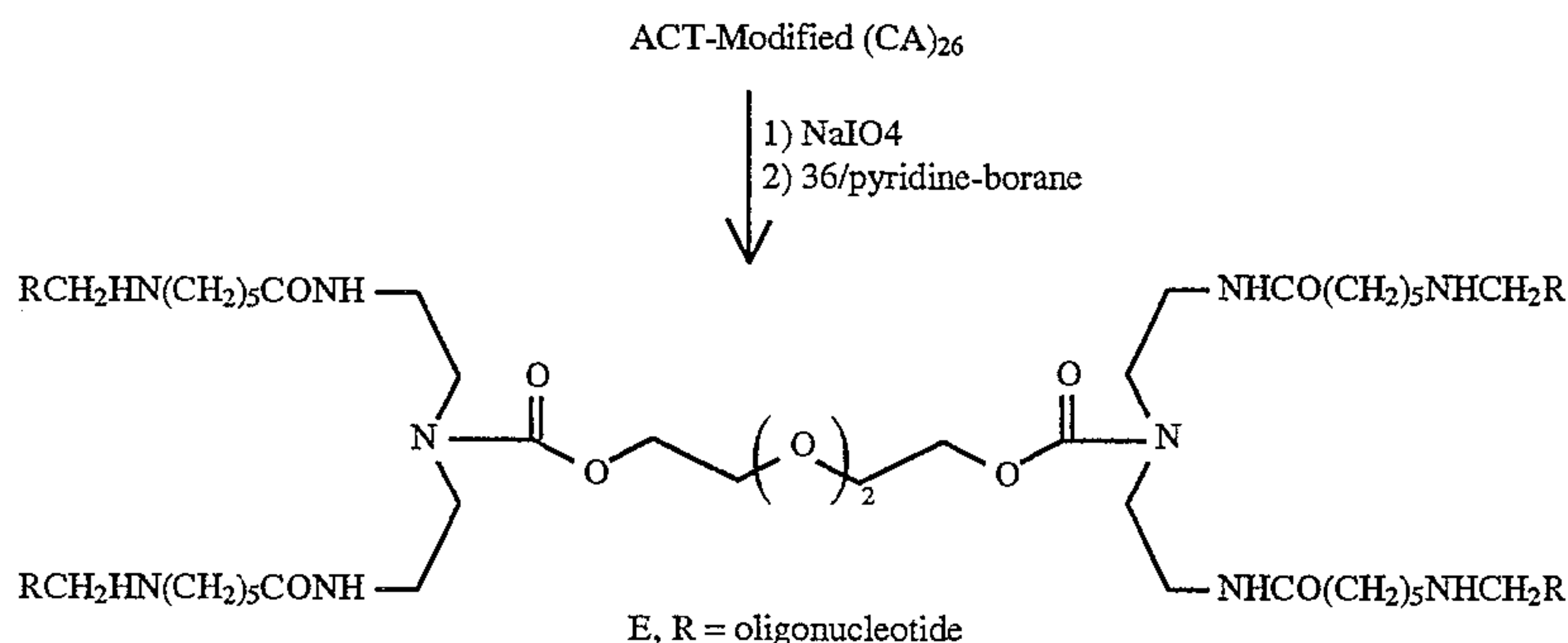
Combination 3: Amine on Platform - Aldehyde on Oligonucleotide Reaction Scheme 16
