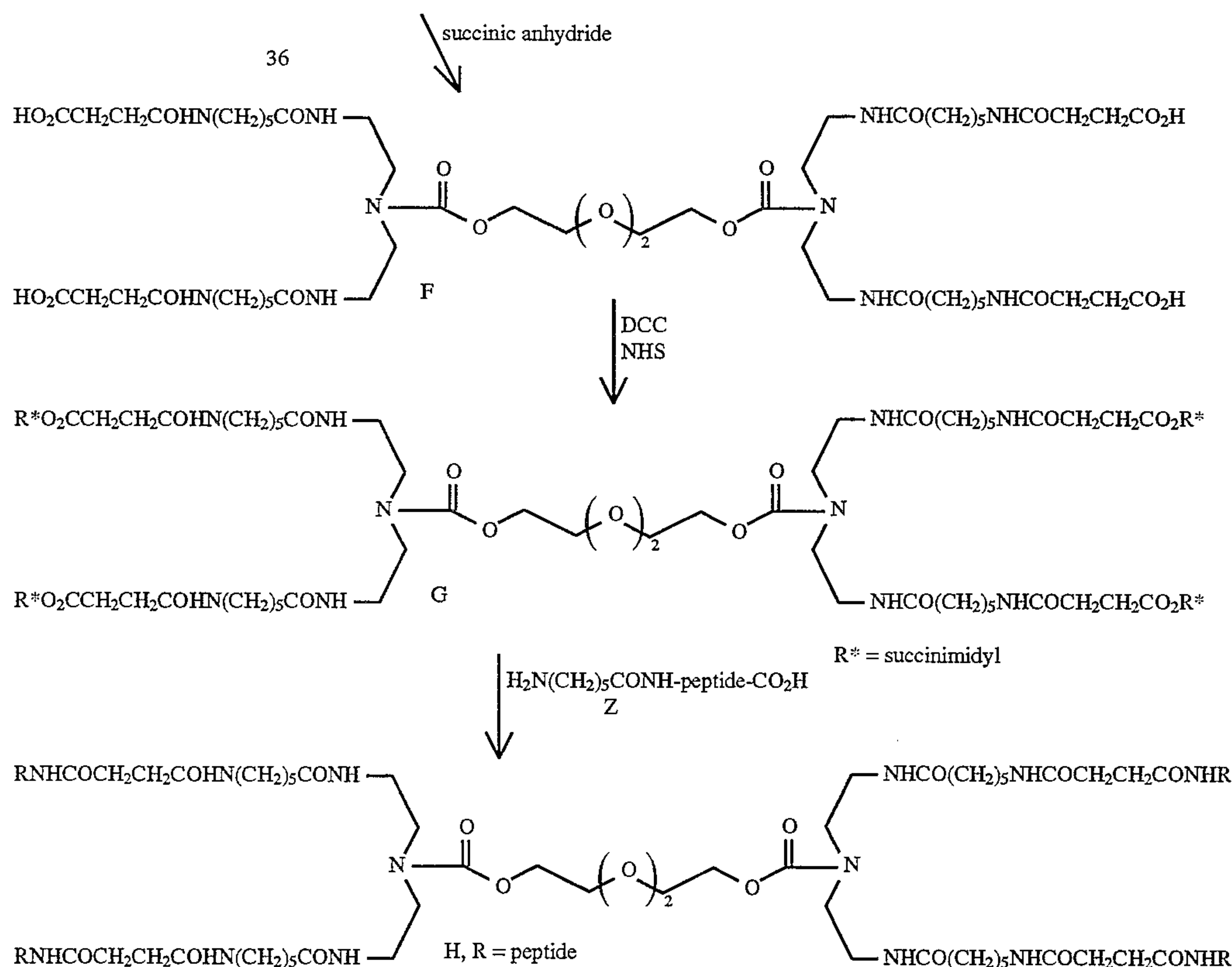
Combination 4: Activated Carboxylate on Platform - Amine on Ligand Reaction Scheme 17
