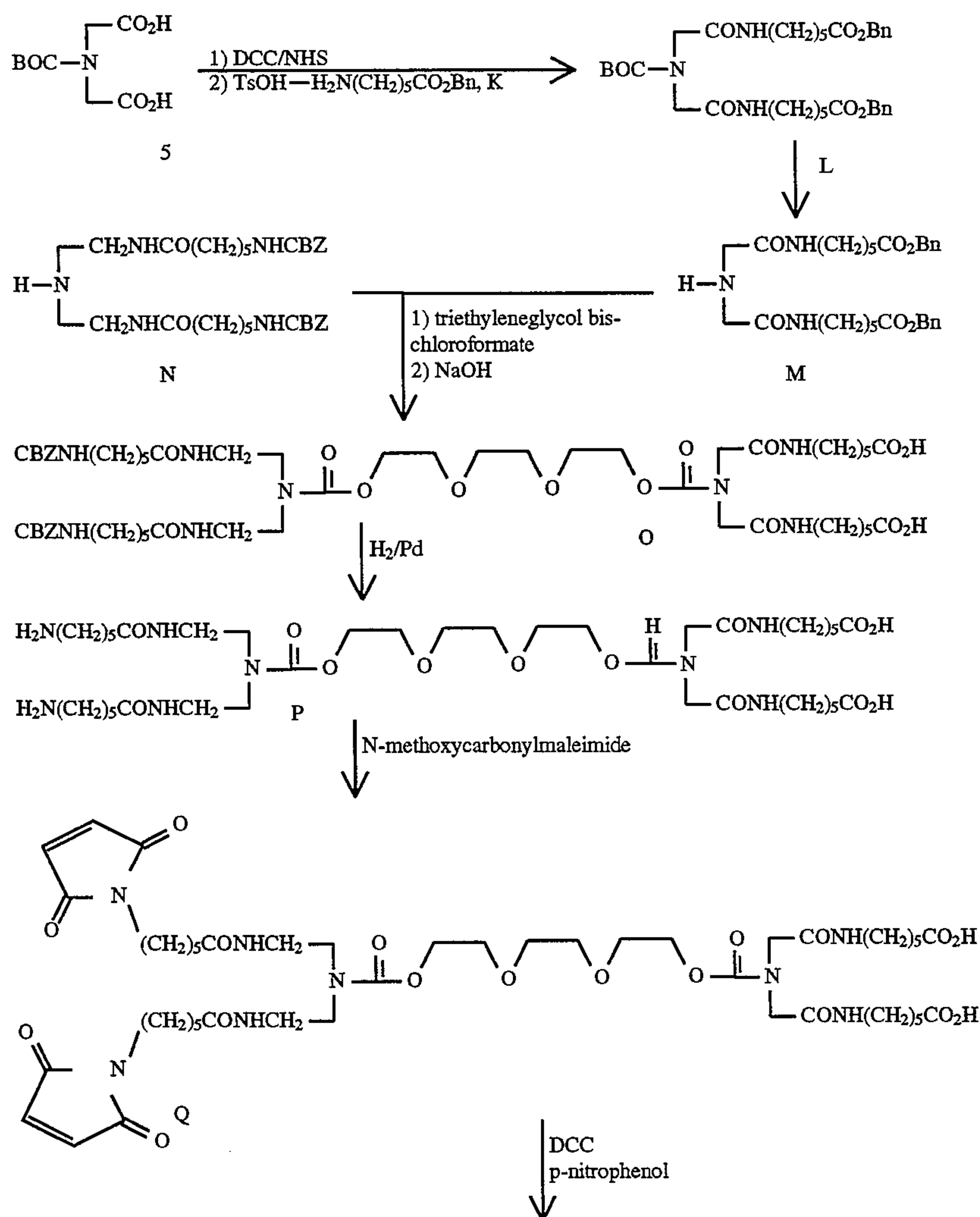
Reaction Scheme 20
