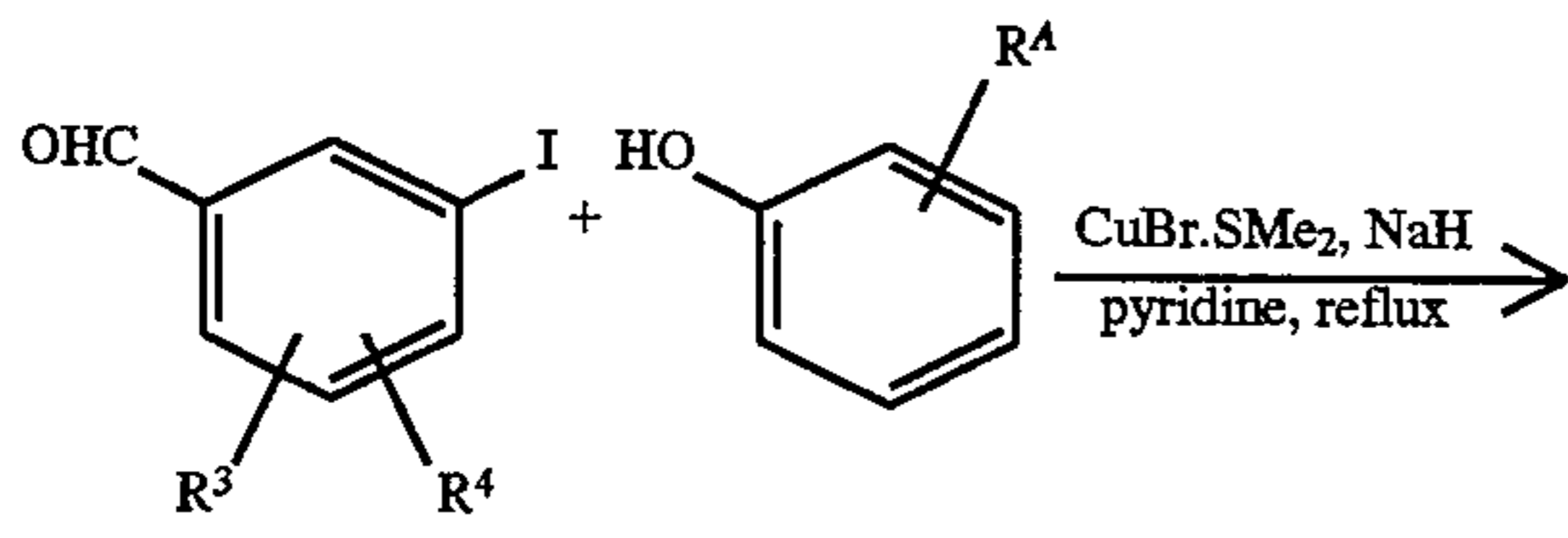
SCHEME 7
