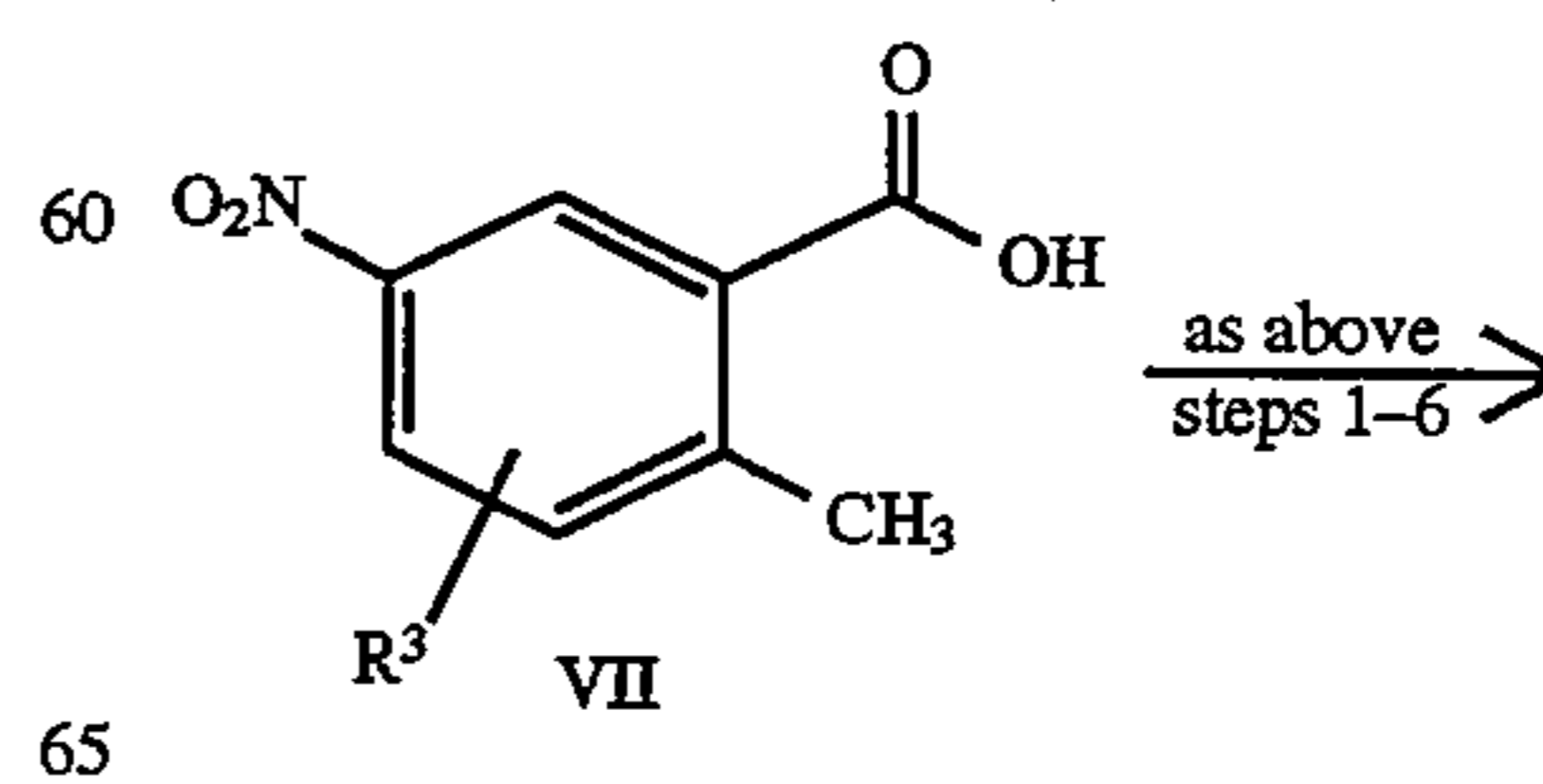
SCHEME 17
