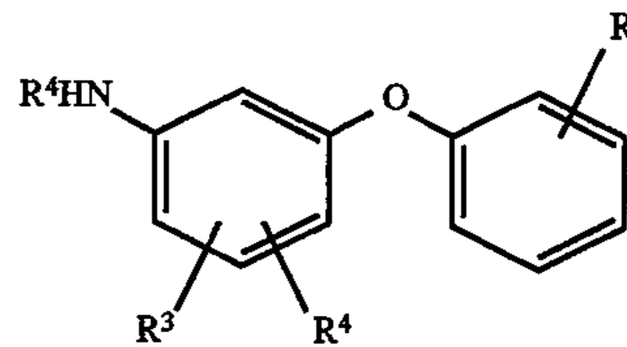
SCHEME 8
