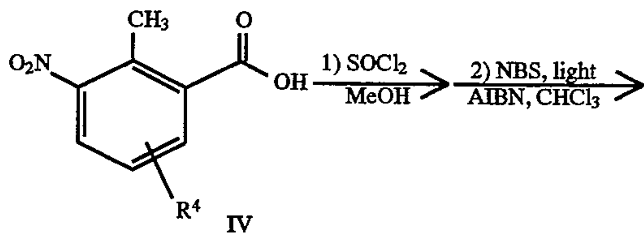
SCHEME 16
