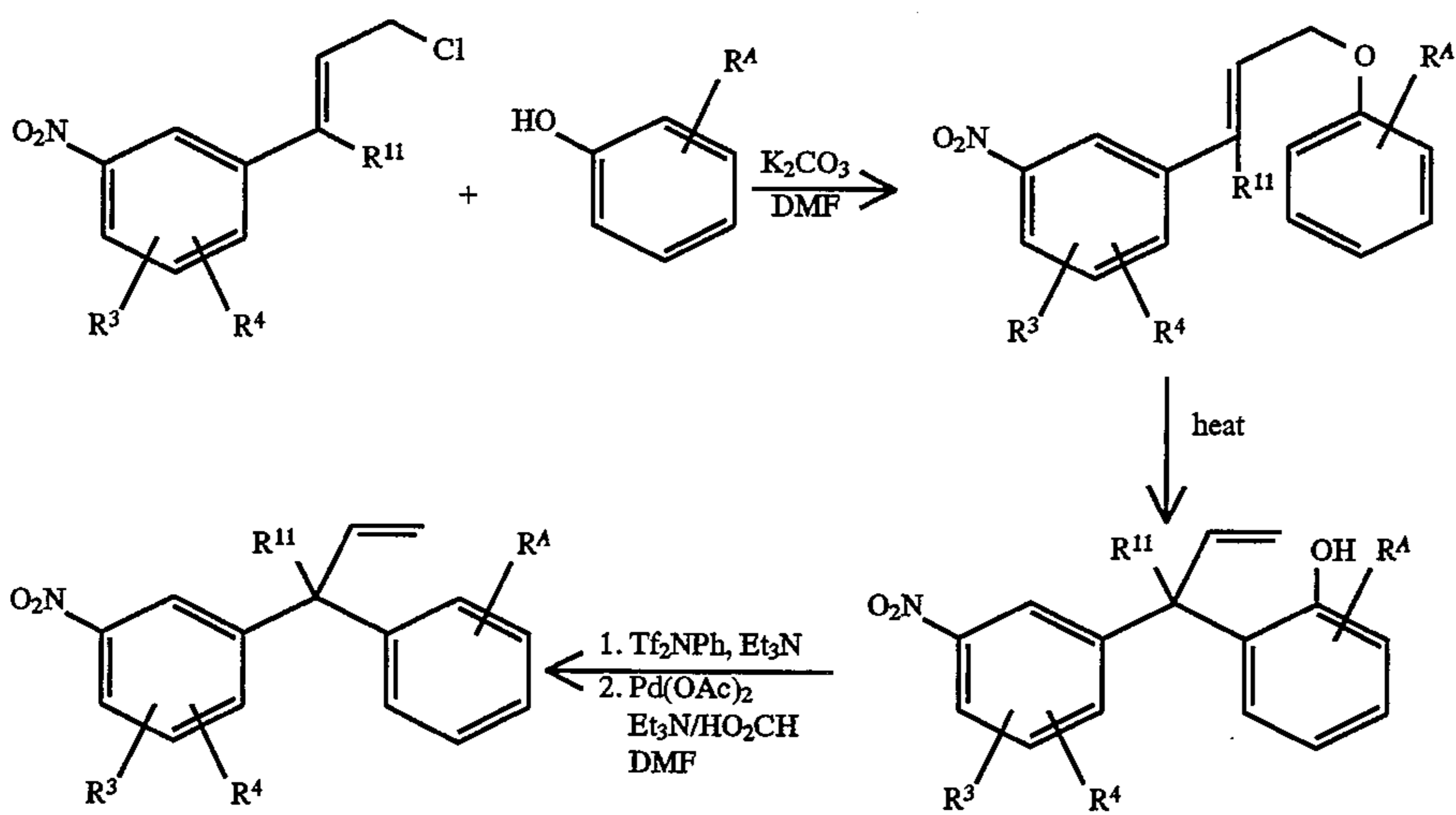
SCHEME 15
