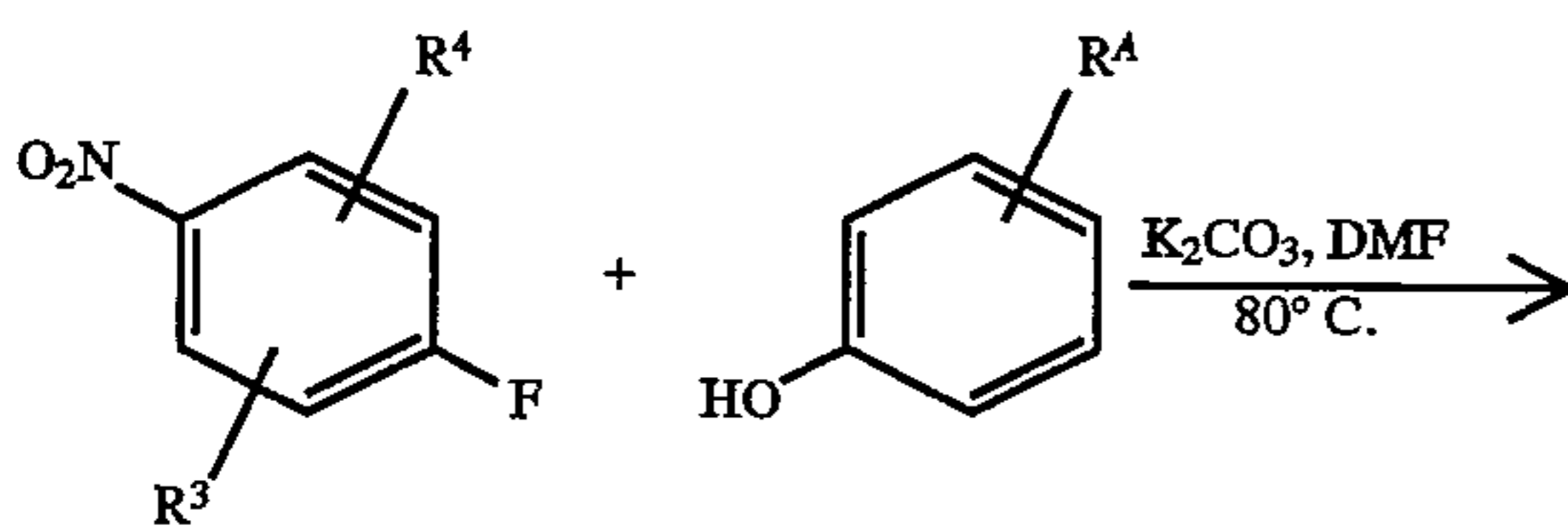
SCHEME 8
