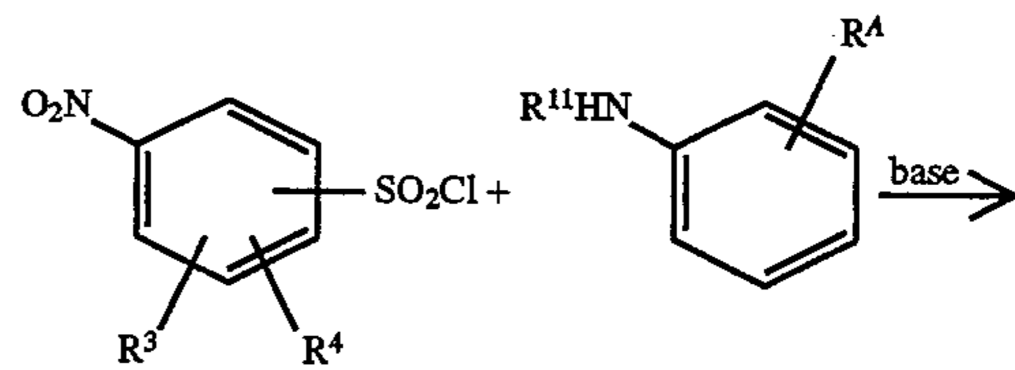
SCHEME 9
