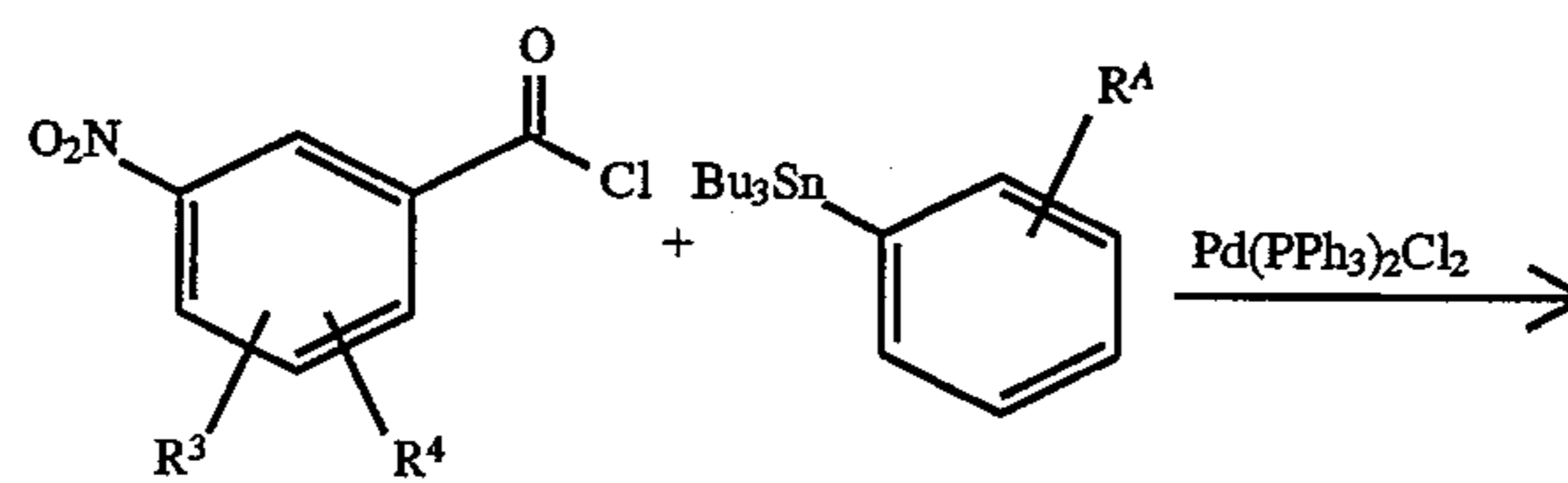
SCHEME 10
