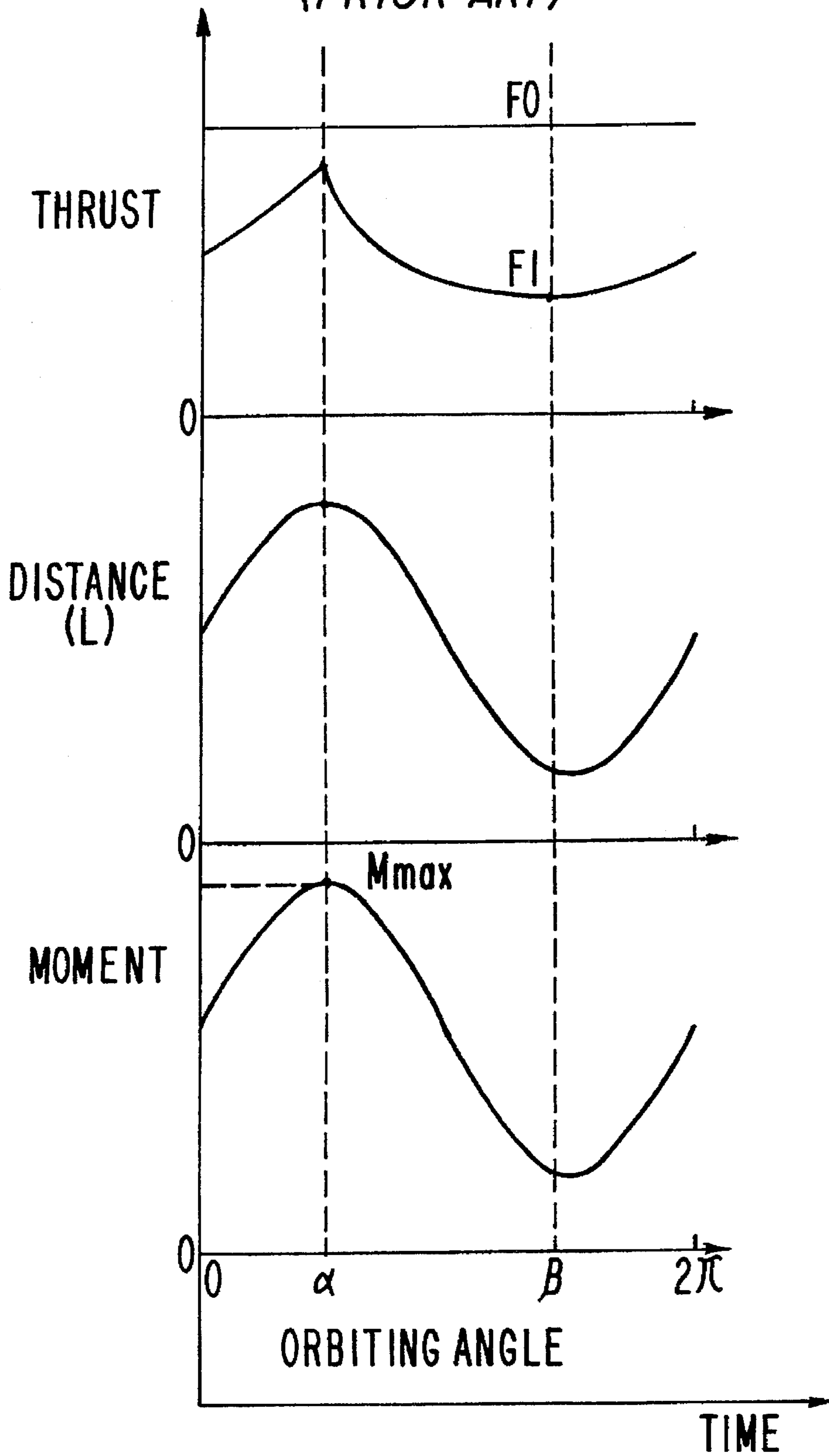
FIG. 17 (PRIOR ART)
