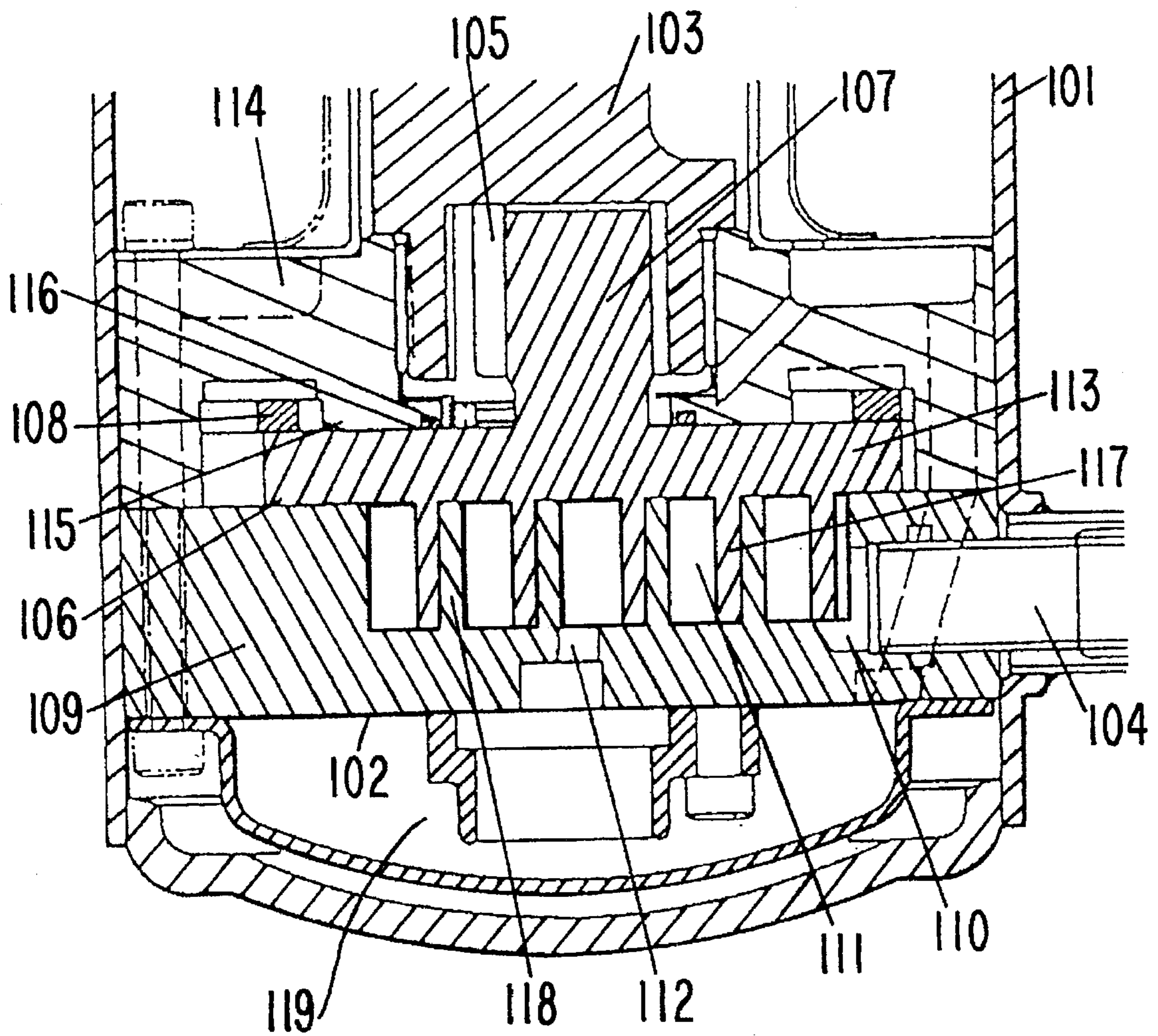
FIG. 14 (PRIOR ART)
