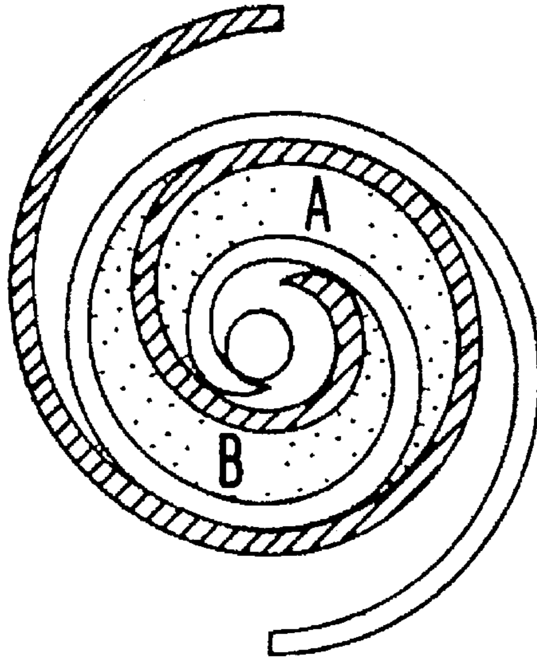
FIG. 15C (PRIOR ART)
